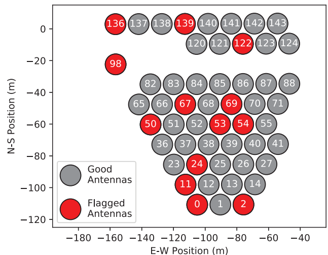
Figure 5. Layout of HERA antennas between JD 2458098 and 2458116. These 14-m diameter dishes are on a hexagonal grid with a separation of 14.6 m and will eventually be part of the Southwest sector of the split HERA core when HERA-350 is complete. Antennas flagged for non-redundancy or otherwise suspected of malfunctioning (see Section 3.2) are noted in red and excluded from the final redundant-baseline calibration examined in this work.
