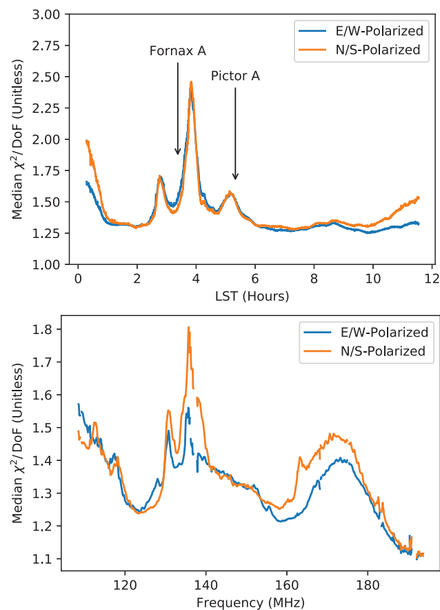
Figure 10. Collapsing Fig. 9 along both the frequency and time axis (while breaking it up into two polarizations) reveals significant structure in \chi^2 , likely due to the primary beam. We attribute the temporal structure to bright point sources moving through the main lobe of the primary beam – lowering \chi^2 by making gain and beam variations degenerate – or through the sidelobes – highlighting the antenna-to-antenna variation. We explore this explanation more in Section 4. The frequency structure appears correlated with beam directivity, though the underlying cause of that correlation is less well understood.
