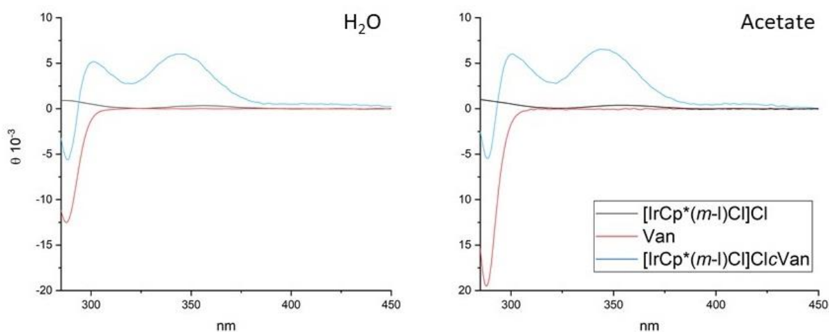
Figure 2. CD spectra of [\text{IrCp}^*(m\text{-I})\text{Cl}]\text{Cl} and [\text{IrCp}^*(m\text{-I})\text{Cl}]\text{Cl}\text{-Van} in water and acetate (2.5 mM concentration, 25°C).
