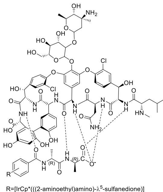
Figure 1. H-bond interactions between Van and DADA.
