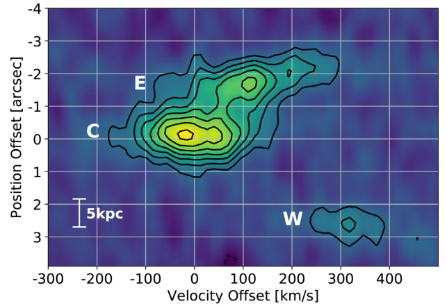
Figure 3. Position–velocity diagram taken east–west, centred on the central source, with a total width of 8 arcsec and an averaging width of 5 pixels. Contours begin at 3\sigma , where 1\sigma = 0.6 \text{ mJy beam}^{-1} , and are in steps of 2\sigma . East is up and west is down. Scale of 5 kpc shown to lower left.
