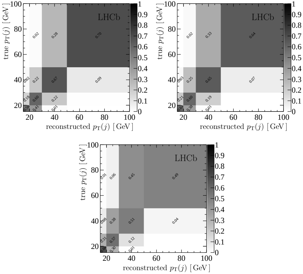
Figure 5. Detector-response matrices for (left) D^0 -, (right) D^{+-} - and (bottom) DV-tagged charm jets. The shading represents the interval-to-interval migration probabilities ranging from (white) 0 to (black) 1 such that each row sums to unity when the underflow and overflow bins are included. Jets with true (reconstructed) p_T(j) in the 20–100 GeV region but whose reconstructed (true) p_T(j) is either below 15 GeV or above 100 GeV are included in the unfolding but not shown graphically.
