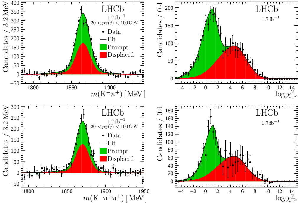
Figure 2. Background-subtracted (left) invariant mass and (right) \log \chi^2_{\text{IP}} projections and fit results for all (top) D^0 \rightarrow K^- \pi^+ and (bottom) D^+ \rightarrow K^- \pi^+ \pi^+ candidates associated with jets reconstructed in the efficiency-reporting region. The background uncertainties, which are included in the error bars, predominantly affect the displaced components.
