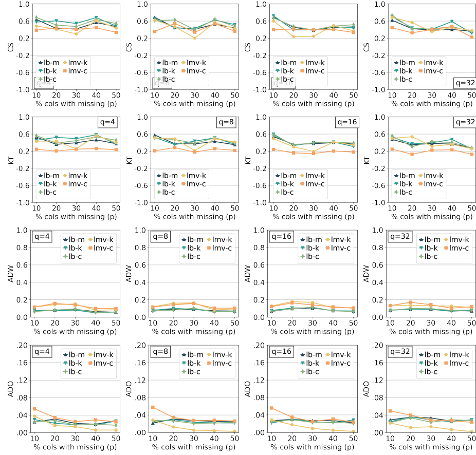
Fig. 4. Impact on evaluation measures of the variation of percentage of features with missing values ( p ) and percentage of missing values in features ( q ) for german .
