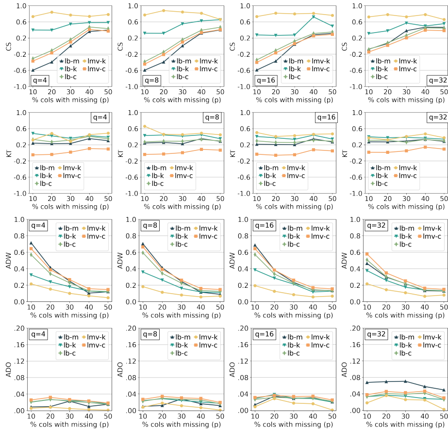
Fig. 3. Impact on evaluation measures of the variation of percentage of features with missing values ( p ) and percentage of missing values in features ( q ) for adult .
