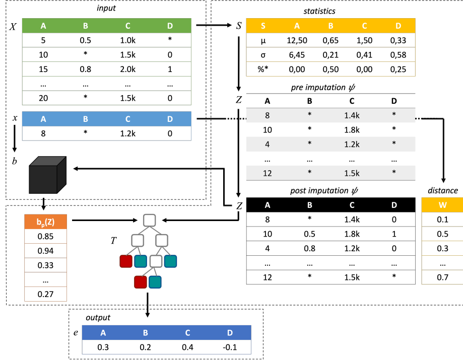
Fig. 1. LIMEMV takes as input the reference dataset X , the instance to explain x and the black-box b , and returns as output a feature importance explanation e . The workflow highlights the statistics S calculated considering missing values and shows the synthetic neighborhood Z before and after the imputation with \psi . Finally, e is returned as feature importance extracted from a local regressor tree using as target variable the probability b_p(x) for the decision y = b(x) .
