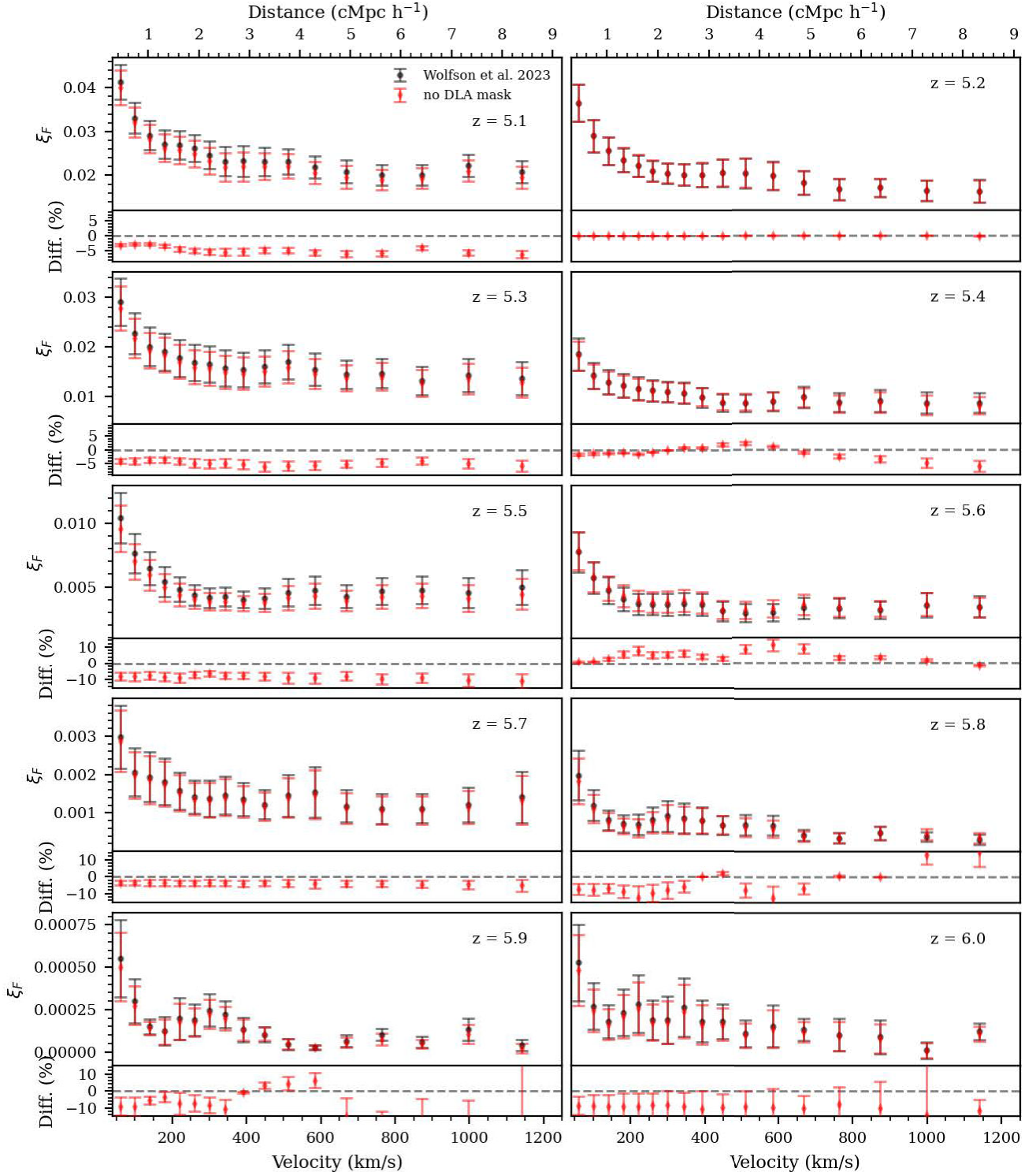
Figure B1. The black points show autocorrelation function of Ly \alpha transmission in ten redshift bins measured in this work. The red points show the measured autocorrelation function of the Ly \alpha transmission when ignoring the masks for the DLAs as described in Section 3.3. In general, ignoring the DLA mask decreases the autocorrelation function values.
