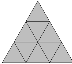
Figure 7: How to subdivide the 2-cells of Y to obtain a simplicial complex.
