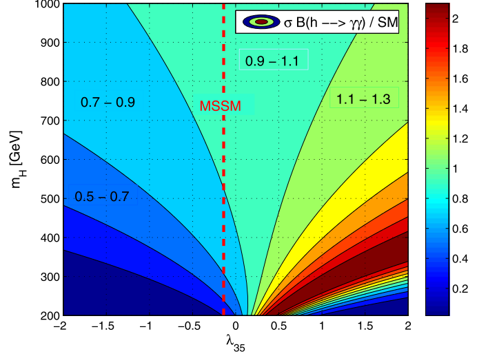
Fig. 1. Contours of \sigma \times BR(h \rightarrow \gamma\gamma)/(SM) vs. \lambda_{35} and m_H , for m_h = 125 GeV and \lambda_7 = 0 . (Recall \lambda_{35} = \lambda_3 + \lambda_5 .) The MSSM prediction, neglecting loop corrections to the bottom Yukawa (but effectively including corrections to the Higgs potential), is shown by the dashed line.
