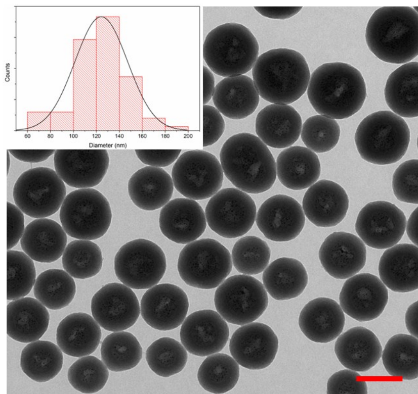
Figure S3: TEM image of t NAs. Scale bar 100nm. The inset shows the size histogram of t NAs calculated on n=151 nanoparticles.
