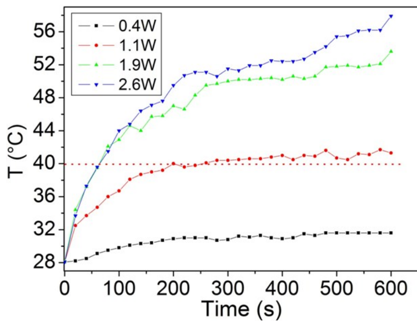
Figure S4: Temperature trend of colloidal dispersion of t NAs upon irradiation at varying laser output power for 10 minutes.
