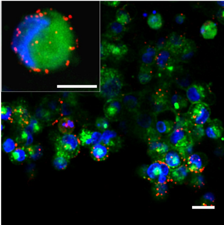
Figure S9: Confocal images of 3D MIA PaCa-2 model after 2 hours of incubation with NAs. Red, blue and green LUTs represent AlexaFluor 647 from t NAs, Hoechst 33342, and CellMask green plasma membrane stain, respectively. Scalebar: 20 \mu m. Inset: NAs on a single cell. Scalebar: 10 \mu m.
