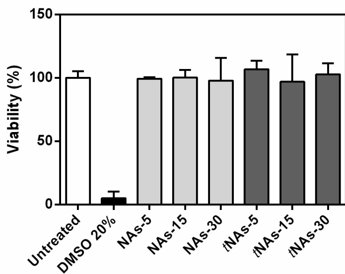
Figure S7: WST-8 viability assay on NAs and t NAs incubated in Mia PaCa-2 cells at increasing amount of nano-architectures (5, 15 and 30 μg).
