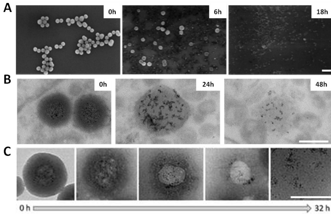
Figure S2: Electron microscopy imaging of NAs biodegradation in (A) full human serum, (B) 2D-cultured Mia PaCa-2 cells, (C) full human blood. Scale bars: 100 nm
