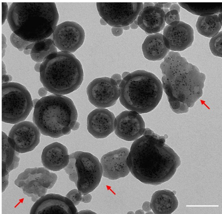
Figure S5: TEM images of t NAs after 4 PT cycles at laser power 2.6 W. Red arrows highlights t NAs that underwent structural breakage most probably for the pressure caused by the high temperature reached in the core. Scale bar: 100 nm.
