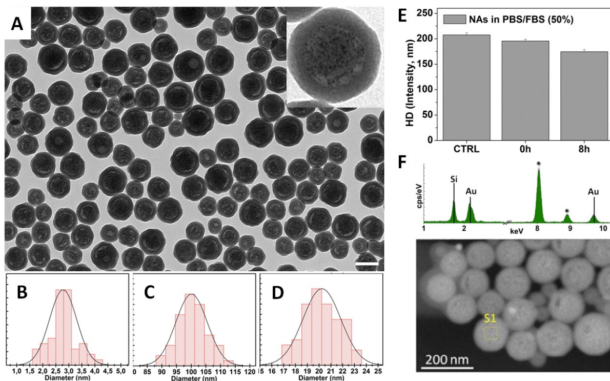
Figure S1: (A) Typical wide-area TEM image of NAs. Scale bar 100 nm. Inset: zoom on one NA. Size histogram of gold USNPs (B), NAs (C), and NAs shell (D) made on at least 100 NAs observed by TEM. (E) DLS measurements on NAs in blood-mimicking solution over 8 hours vs CTRL (NAs in PBS buffer). (F) EDX analysis on NAs revealing the presence of silicon and gold (copper peaks from TEM grid are marked with a black star).
