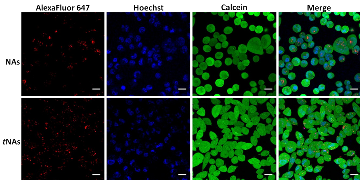
Figure S6: Confocal fluorescence images of the cellular uptake assessment for NAs and t NAs on 2D cultured MIA PaCa-2 cells. Red, blue and green LUTs represent AlexaFluor 647 from nano-architectures, Hoechst and Calcein, respectively. Scale bars: 10 \mu m.
