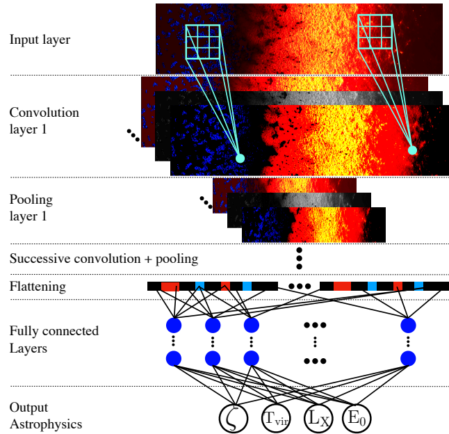
Figure 4.10: An example architecture of a convolutional neural network. Showing the architecture from an input two-dimensional light-cone of the 21-cm signal down to the output astrophysical parameters. Reproduced from [64]. Copyright of OUP Copyright 2019.
