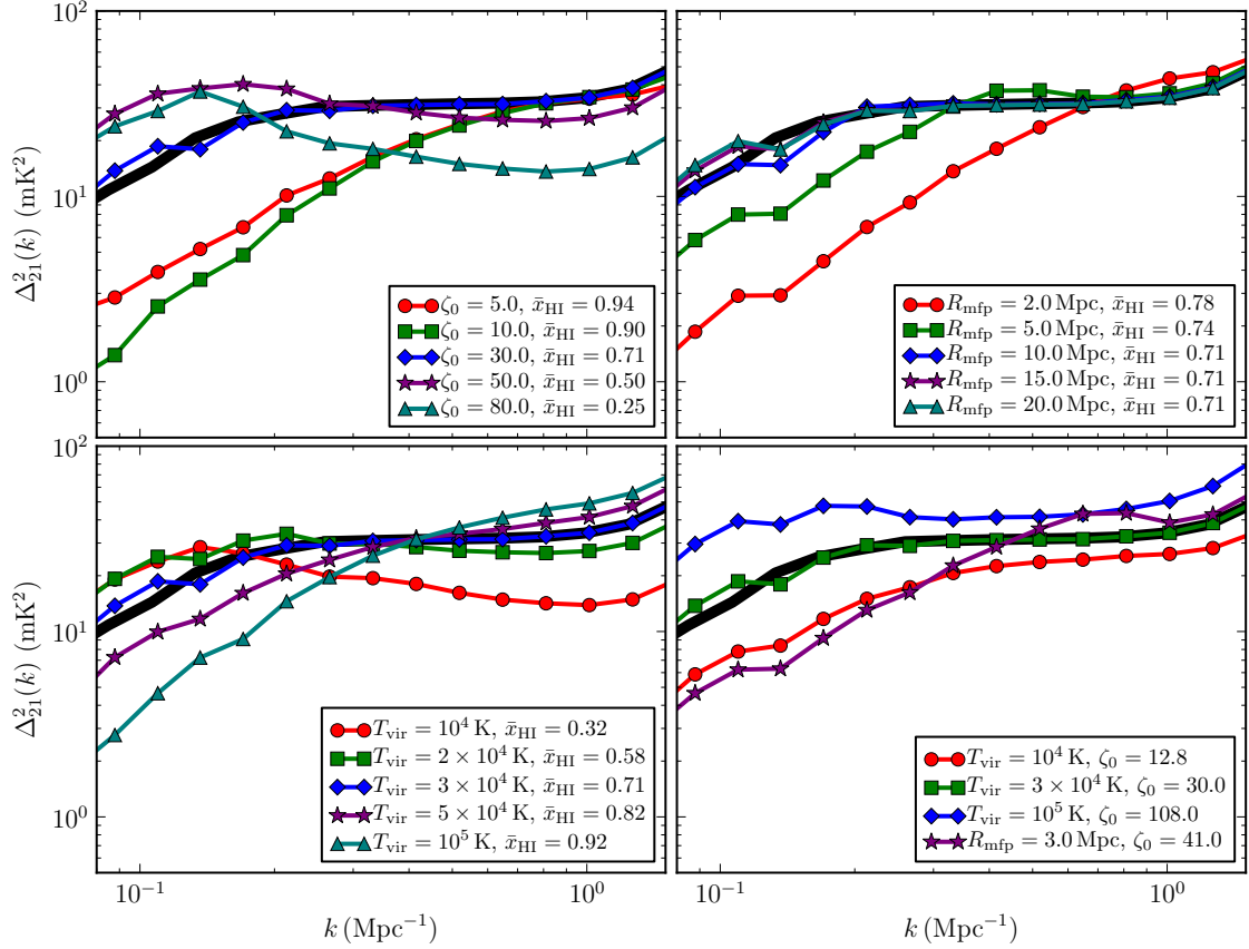
Figure 4.4: The three dimensional spherically averaged 21-cm power spectrum at z = 9.0 when varying astrophysical parameters controlling different astrophysical processes, assuming T_{\text{S}} \gg T_{\text{CMB}} . Top left: the number of ionising photons produced per baryon (ionising efficiency, \zeta ), top right: maximum ionising photon horizon (proxy for maximum allowable bubble size, R_{\text{mfp}} ) and bottom left: minimum mass of halo hosting star-forming galaxy (represented here as T_{\text{vir}} ). Bottom right: several models at the same ionisation fraction. Reproduced from [74]. Copyright of OUP Copyright 2019.
