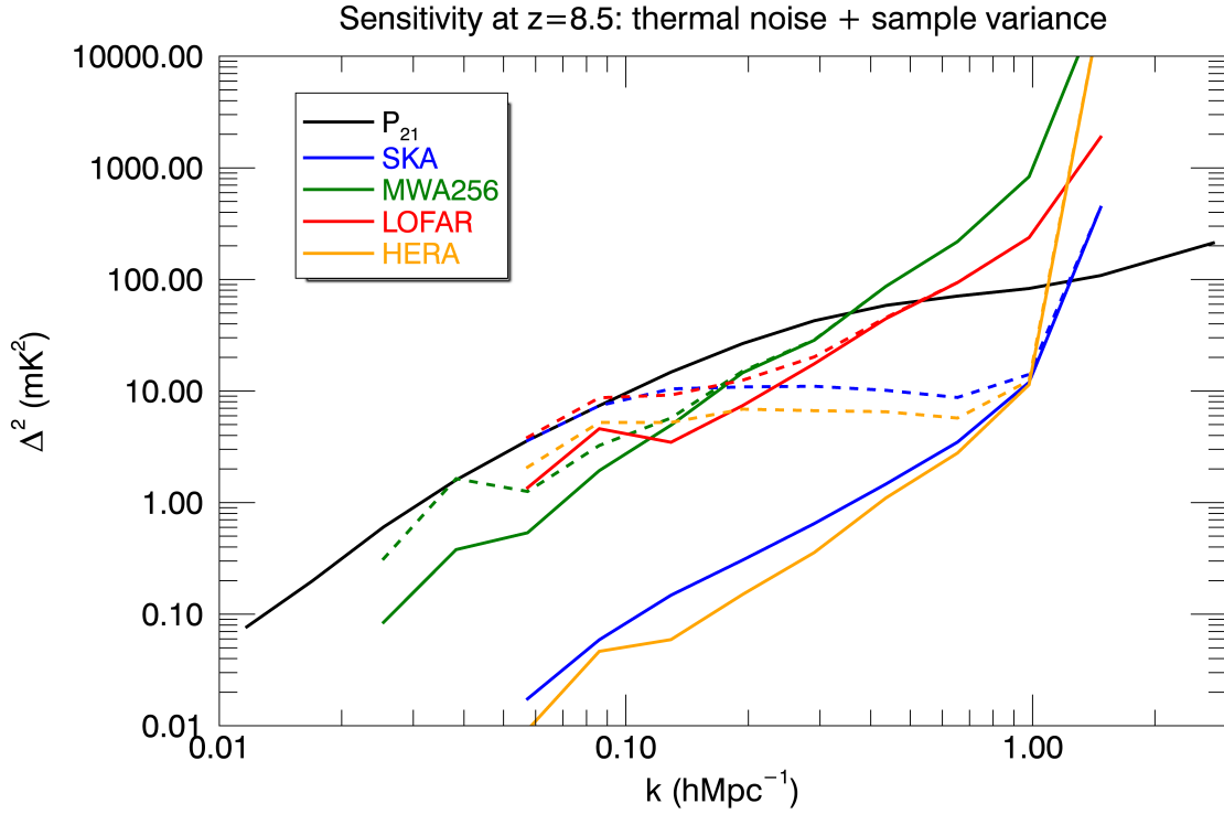
Figure 8.1: Estimated total uncertainty on the dimensionless power spectrum for a 1000 hour observation with several experiments at z=8.5 compared with a model input power spectrum (21cmFAST,[75]), and assuming that modes within the horizon are inaccessible. Solid lines are only thermal noise uncertainty, while dashed lines include sample variance. (Black) Model cosmological signal; (blue) SKA; (green) MWA256; (red) LOFAR; (orange) HERA.
