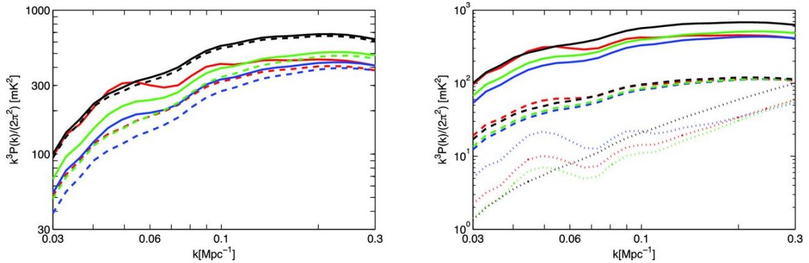
Figure 2.12: Effects of LW feedback on the 21-cm power spectrum [39]. Left: Power spectra with different feedback models, including no feedback (red), weak (blue), strong (green), and saturated (black). Dashed curves exclude the baryon-DM velocity offset effect [147]. Right: All models here include the baryon-velocity offset effect – linestyles indicate power spectra at three different redshifts. Note that because changes to the strength of feedback shift the timing of events, models are compared at fixed increments relative to the “heating redshift,” z_0 , which in these models occurs between z \sim 15 and z \sim 18 [39]. Dashed lines are power spectra at z = z_0 , while z = z_0 + 3 and z = z_0 + 9 are shown by solid and dotted lines, respectively.
