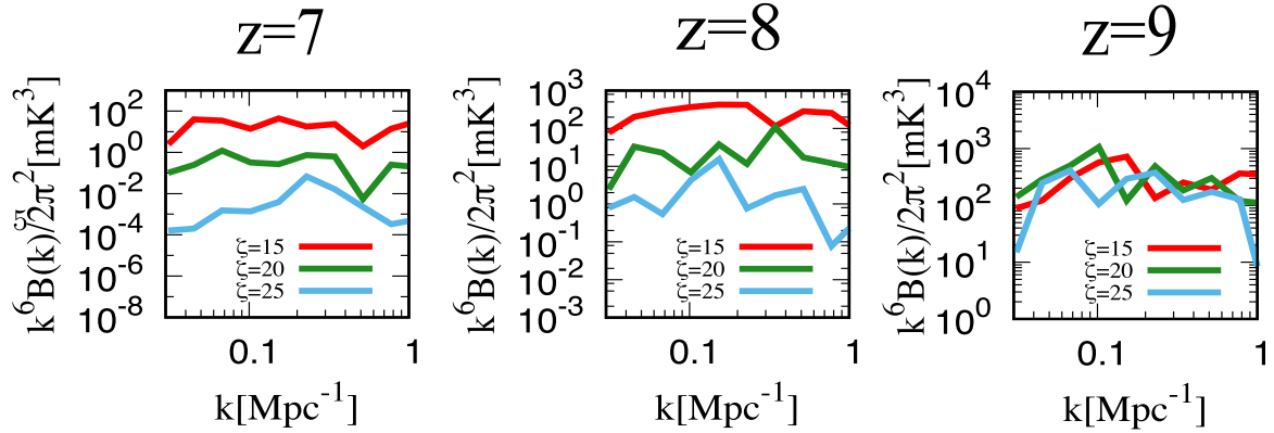
Figure 4.5: Variation in the amplitude of the equilateral bispectrum at z = 7, 8 and 9 for different ionising efficiencies, \zeta . Reproduced from [198]. Copyright of OUP Copyright 2019.
