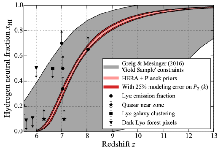
Figure 9.4: 95% confidence region on the Hydrogen neutral fraction X_{\text{HI}} (grey, from [21]). The inclusion of HERA measurements leads to a dramatic improvement in the constraints (red and pink areas, [27]). Constraints from other reionization probes are shown as well (see [12] for a detailed description).
