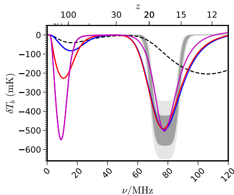
Figure 3.4: Left: The Dark Ages 21-cm absorption trough in the standard cosmology. The shape at z > 30 is independent of astrophysical sources. Right: The black dashed line shows the mean 21-cm brightness temperature (averaged across the sky) in the standard cosmology. The gray contours show schematically the reported EDGES absorption signal [7]. The solid curves are phenomenological models that invoke extra cooling to match the amplitude of the EDGES signal but that also dramatically affect the Dark Ages absorption trough at z > 50 . Courtesy J. Mirocha, based on calculations in [49].
