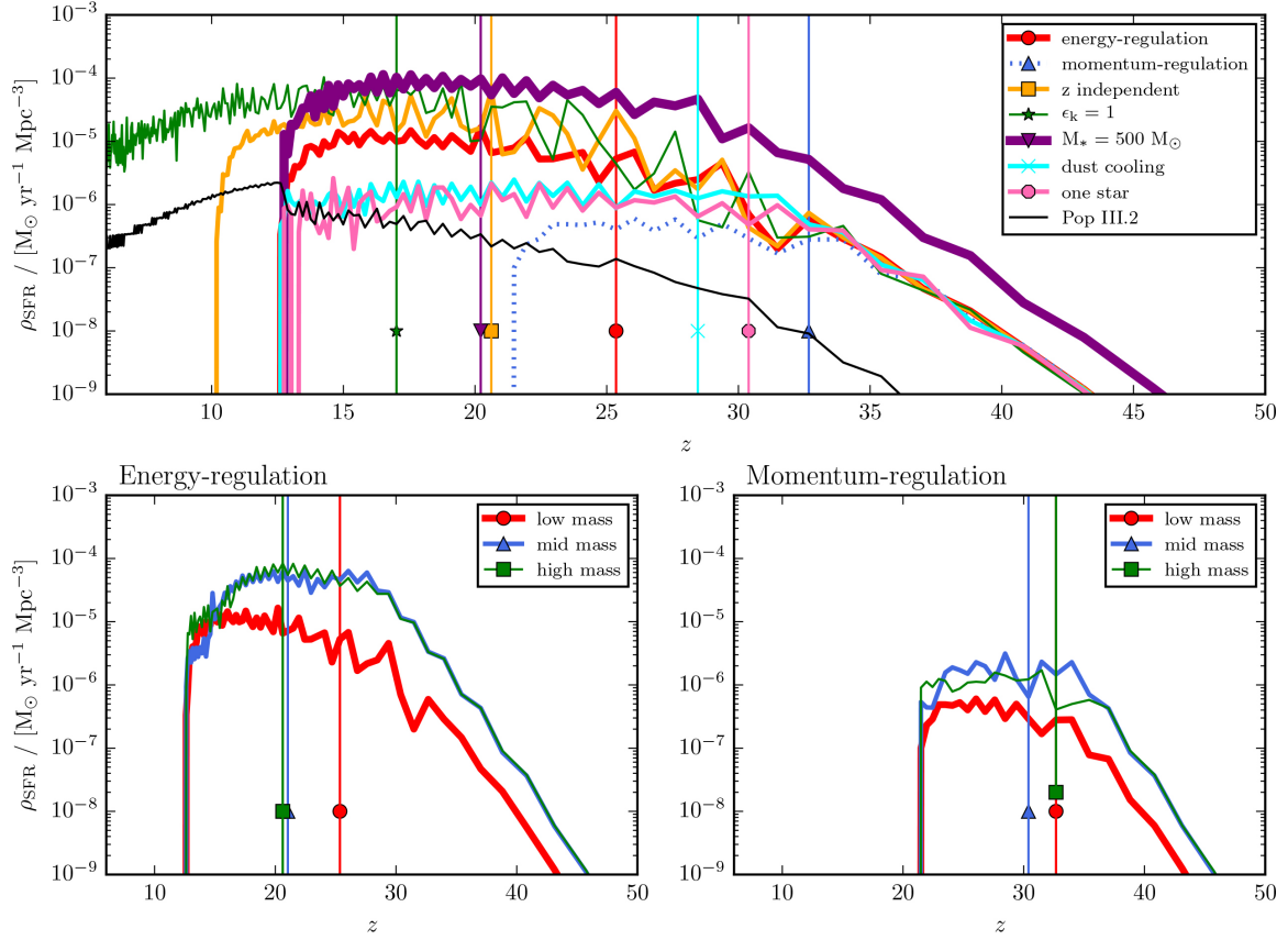
Figure 2.4: Predictions for the Pop III SFRD at high- z [84]. Upper panel shows results assuming a low-mass Salpeter-like Pop III IMF with different assumptions about the Pop II and Pop III star formation prescriptions. Lower panels study the effects of Pop III IMF between energy-regulated (left) and momentum-regulated (right) stellar feedback from Pop II stars. Note that the Pop II SFRD inferred from current UVLF measurements is of order \sim 10^{-2} M_{\odot} \text{ yr}^{-1} \text{ cMpc}^{-3} at z \sim 6 [10, 43].
