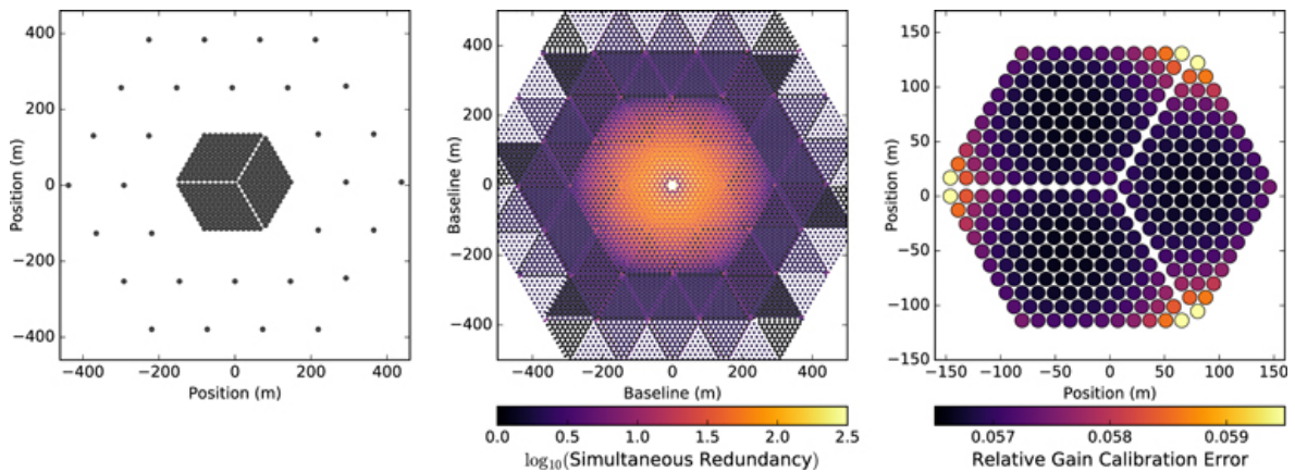
Figure 9.3: The HERA layout (left panel): 320 dishes are located in the hexagonal core and 30 more outrigger dishes are planned to be deployed out to a maximum baselines of \sim 800 m to improve angular resolution and imaging capabilities. The core is split in three sectors that are displaced from each other by a fraction of the dish diameter (see [15] for a detailed discussion). The split core provides a significantly improved instantaneous uv coverage (central panel) whilst retaining high redundancy. The right panel shows the expected relative antenna gain errors after using redundant calibration (from [15]).
