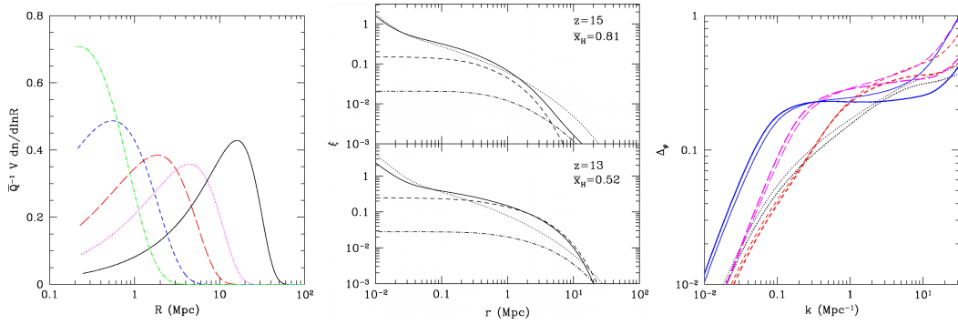
Figure 2.7: Analytic models of bubble growth during the EoR [48]. Left: Bubble size distributions at bubble filling fractions of Q = 0.037, 0.11, 0.3, 0.5 , and 0.74 , from left to right. Middle: Correlation function of \psi = x_{\text{HI}}(1 + \delta) (solid) at x_{\text{HI}} = 0.81 (top) and x_{\text{HI}} = 0.52 (bottom) as well as its constituent components, including the ionization auto-correlation function (dashed), density auto-correlation function (dotted), and cross-correlation function between ionization and density (dot-dashed). Right: Dimensionless power spectrum of \psi for different values of \zeta , including \zeta = 12 (thin) and \zeta = 40 (thick), at several neutral fractions, x_{\text{HI}} = 0.96 (dotted), 0.8 (short-dashed), 0.5 (long-dashed), and 0.26 (solid).
