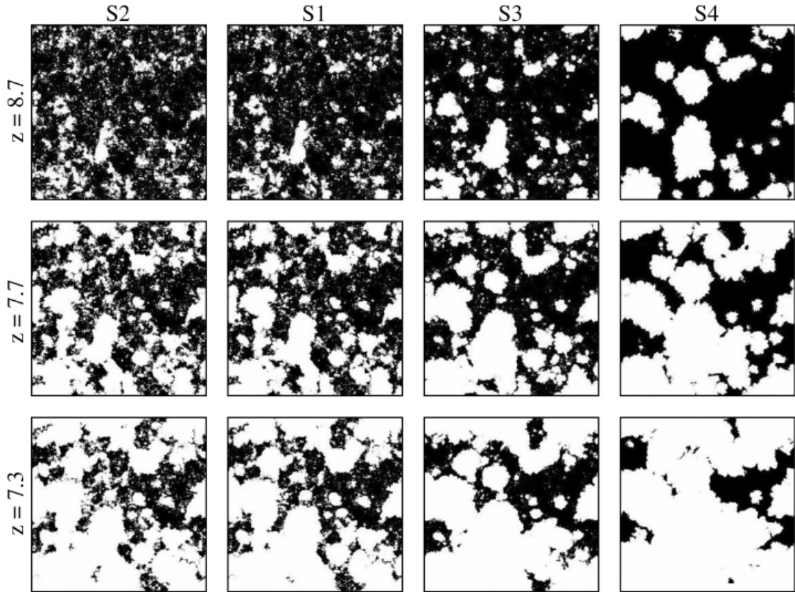
Figure 2.8: Ionization field in (94 \text{ cMpc})^3 box for different ionizing efficiency assumptions [83] as a function of redshift (top to bottom). Neutral gas is black, while ionized regions are white. Each column shows results from a different simulation, with S1-S3 using \zeta = \text{constant} , \zeta \propto m_h^{-2/3} , and \zeta \propto m_h^{2/3} , respectively. S4 is the same as S1 except only halos with m_h > 10^{10} M_\odot are included.
