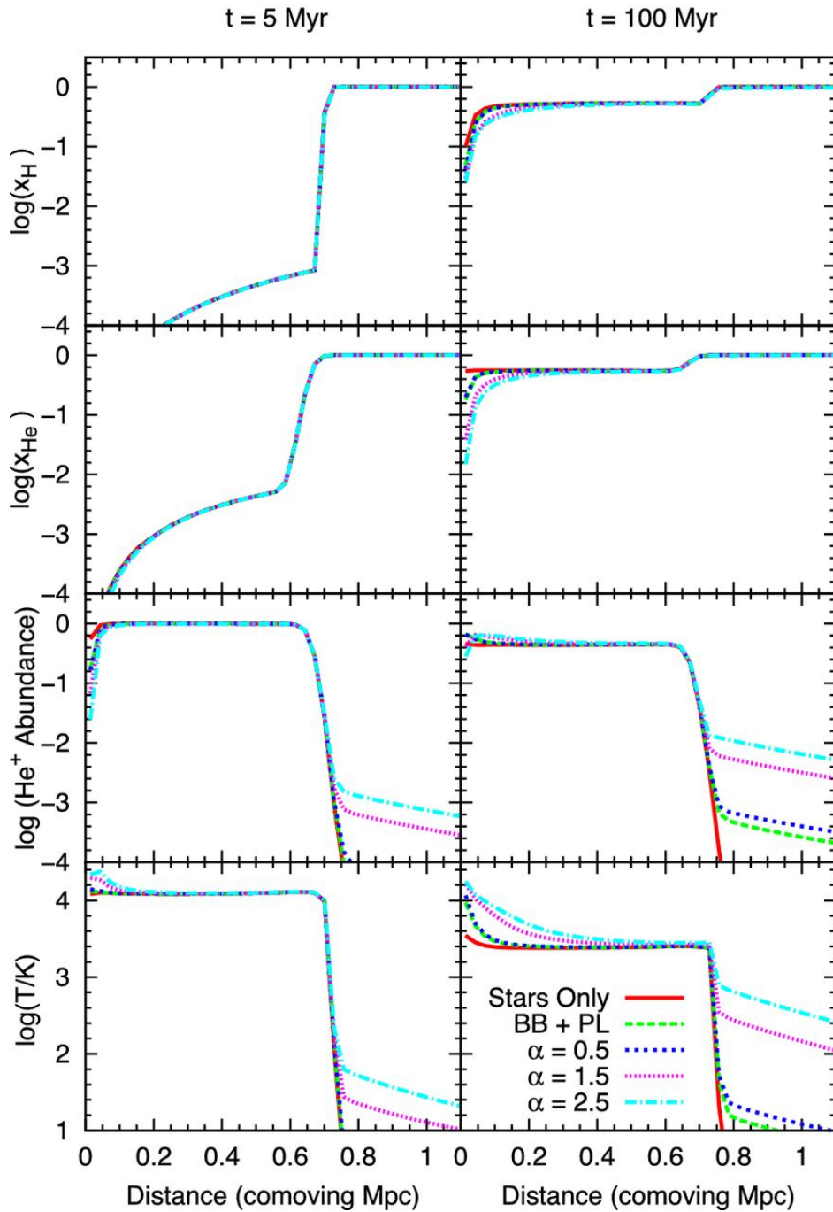
Figure 2.1: Ionization and temperature profile around stellar UV and X-ray sources in a one-dimensional radiative transfer model [67]. From top to bottom, this includes the hydrogen neutral fraction, neutral helium fraction, singly-ionized helium fraction, and kinetic temperature, while the left and right columns indicate different time snapshots after sources are first turned on. Different lines adopt different source models, from a “stars only” model (solid red), to hybrid models with stars and X-ray sources with different power-law spectra (dashed and dotted curves).
