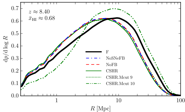
Figure 4.8: Variation in the bubble size distribution with changes in the underlying astrophysics of the source model. Reproduced from [58]. Copyright of OUP Copyright 2019.
