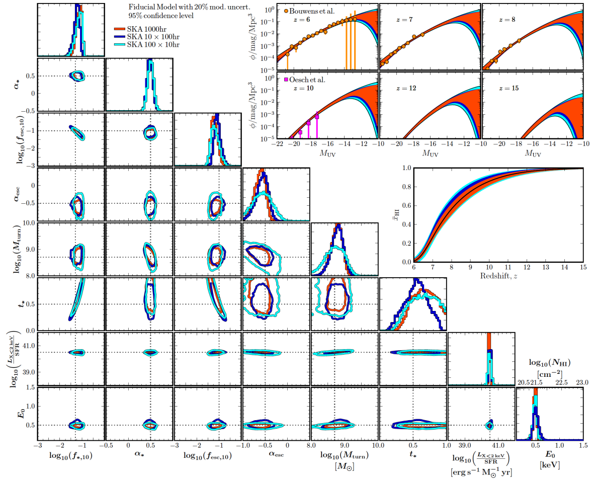
Figure 9.2: Astrophysical parameter constraints for a standard 21-cm signal model using 1000 h of observations with SKA1-low ([22]).
