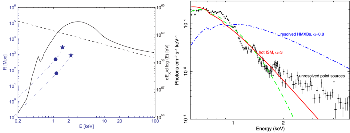
Figure 2.5: Models for the X-ray spectra of star-forming galaxies. Left: Template Cygnus X-1 HMXB spectrum (solid) compared with power-law (dashed), with mean free path shown on left scale and relative luminosity on right [38]. Right: Typical HMXB spectrum (blue) compared to soft X-ray spectrum characteristic of bremsstrahlung emission from hot ISM gas [109].
