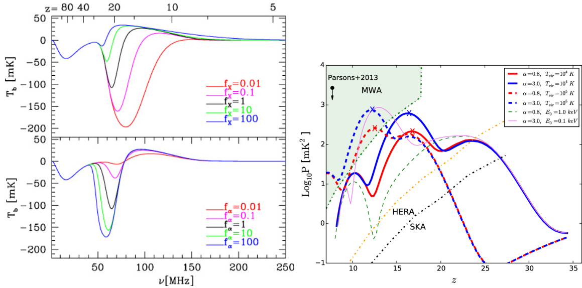
Figure 2.9: Effects of Ly- \alpha and X-ray efficiencies on the global 21-cm signal [117, 109]. Left: Predictions for the global 21-cm signal showing sensitivity to the normalization of the L_X -SFR relation, f_X (top), and the production efficiency of Ly- \alpha photons, f_\alpha (bottom) [117]. Right: Predictions for evolution in the 21-cm power spectrum at k = 0.2 \text{ Mpc}^{-1} for models with different X-ray spectra [109]. Blue curves indicate soft power-law spectra with indices of \alpha = 3 , while red curves are indicative of hard spectra sources with \alpha = 0.8 . Linestyles denote different minimum virial temperatures, T_{\text{min}} , and lower energy cutoffs for the X-ray background, E_0 .
