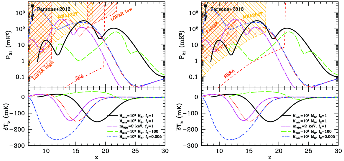
Figure 2.11: Effects of the minimum mass on the global 21-cm signal and 21-cm power spectrum on k = 0.1 \text{ Mpc}^{-1} scales [85]. Solid black, red dotted, and magenta dash-dotted curves hold constant f_\chi = 1 and vary the m_{\text{min}} by-hand (first two) and via a 2 keV warm dark matter particle (magenta). Left and right panels differ only in which sensitivity curves are included for comparison.
