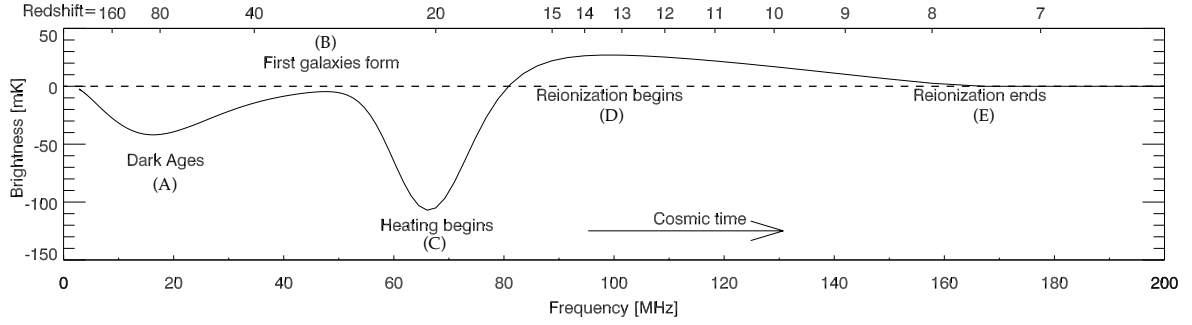
Figure 4.1: A representative example of the all-sky averaged (global) 21-cm brightness temperature signal, demarcating the major cosmological transitions. Reproduced from [180]. ©IOP Publishing Ltd. All rights reserved.
