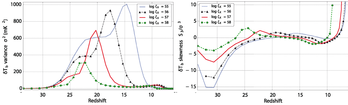
Figure 4.6: The variance (left) and normalised skewness (right) of the 21-cm brightness temperature when varying the efficiency of X-ray heating in the IGM. Reproduced from [214]. Copyright of OUP Copyright 2019.
