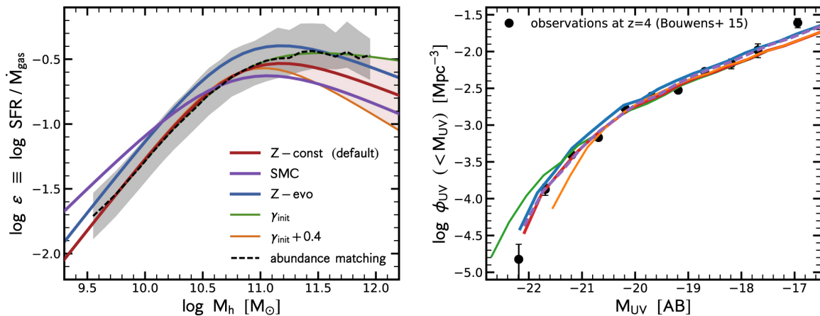
Figure 2.3: Relationship between halos and star formation recovered via semi-empirical modeling [139]. Left : Star formation efficiency as a function of halo mass for a variety of different approaches, including constant metallicity “Z-const”, an evolving metallicity model “Z-evo”, a model with SMC dust instead of the standard relation from [88] (see §2.2.3), and the pure abundance matching approach. Right : Modeled luminosity function at z = 4 compared to measurements from [10].
