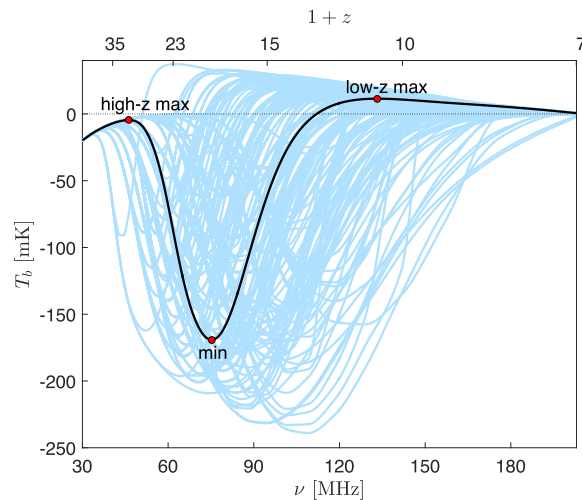
Figure 4.2: The all-sky averaged (global) 21-cm brightness temperature signal obtained when varying the astrophysical parameters in \sim 200 theoretical models. Reproduced from [32]. Copyright of OUP Copyright 2019.
