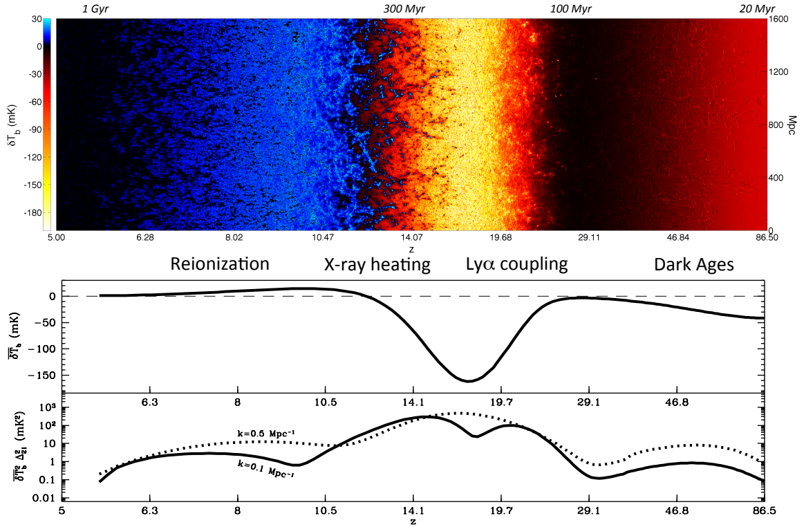
Figure 2.6: Predictions from the 21CMFAST Evolution of Structure (EoS) model suite [87]. Top: 2-D slice of the brightness temperature field, with red colors indicating a cool IGM, blue colors indicative of a heated IGM, and black representing a null signal (either due to ionization or T_S = T_{\text{CMB}} ). Middle: Global 21-cm signal, with dashed line indicating \delta T_b = 0 . Bottom: Evolution of the dimensionless 21-cm power spectrum, \Delta^2 = k^3 P(k) / 2\pi^2 , on two different scales, k = 0.5 \text{ Mpc}^{-1} (dotted) and k = 0.1 \text{ Mpc}^{-1} (solid).
