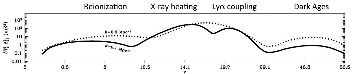
Figure 4.3: The 21-cm power spectrum amplitude for two different Fourier modes, k = 0.1 \text{ Mpc}^{-1} (solid) and k = 0.5 \text{ Mpc}^{-1} (dashed). Peaks in the 21-cm power spectrum amplitude correspond to the different cosmic milestones. Reproduced from [143]. Copyright of OUP Copyright 2019.
