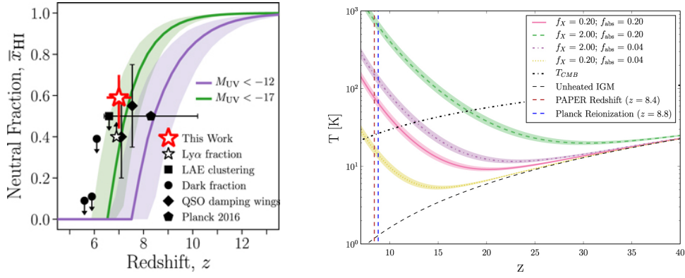
Figure 2.2: Predictions for the evolution of the mean properties of the IGM. Left: Predictions for the mean neutral fraction of the IGM as a function of redshift compared to several observational constraints [80]. Magenta curve includes all galaxies brighter than UV magnitude M_{\text{UV}} < -12 , while green curve includes only brighter galaxies with M_{\text{UV}} < -17 . Right: Predictions for the mean kinetic temperature of the IGM [112] for different assumptions about how efficiently galaxies produce X-rays (parameterized via f_X and the fraction of X-ray energy absorbed in the IGM, f_{\text{abs}} ; see §2.2), compared to an early power spectrum limit from PAPER [111, 113]. Note that the PAPER limit has since been revised [20, 68].
