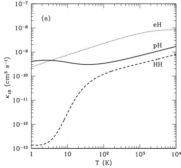
Figure 1.1: De-excitation rate coefficients for H-H collisions (dashed line), H-e - collisions (dotted line), and H-p collisions (solid line). Note that the net rates are also proportional to the densities of the individual species, so H-H collisions still dominate in a weakly-ionized medium. Reproduced from Furlanetto, S. R. & Furlanetto, M. R. “Secondary ionization and heating by fast electrons,” Monthly Notices of the Royal Astronomical Society , vol. 404, pp. 1869-1878. Copyright OUP 2007.
