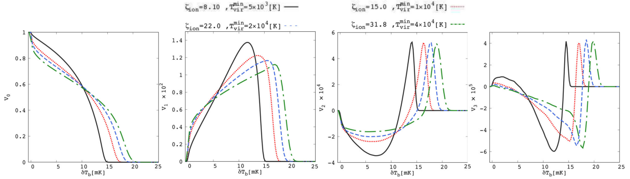
Figure 4.7: The impact of varying the astrophysical parameterisation for a fixed neutral fraction ( x_{H\text{I}} \approx 0.5 ) and redshift ( z = 8.6 ). The coloured curves highlight the impact of varying either the ionising efficiency \zeta or the minimum halo mass for star-forming galaxies, T_{\text{vir}} for the four Minkowski functionals. Reproduced from [222]. Copyright of OUP Copyright 2019.
