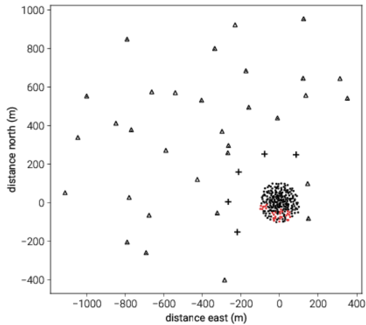
Figure 9.5: LEDA antenna layout: the dense core is surrounded by 32 dipoles in order to provide an exceptionally good instantaneous uv coverage (from [16]).
