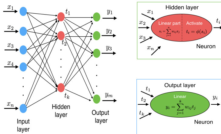
Figure 4.9: An example architecture of an artificial neural network. Reproduced from [195]. Copyright of OUP Copyright 2019.
