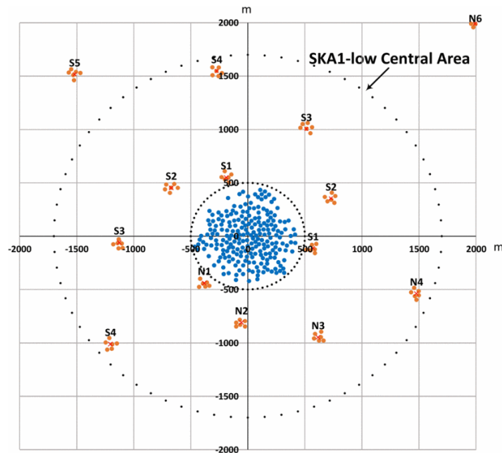
Figure 9.1: SKA1-low core layout, showing the station positions in the inner few km, which are most sensitive to the 21-cm signal ([13], [55]).
