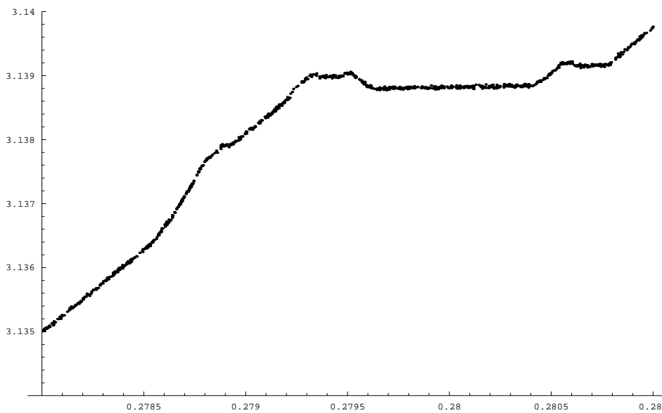
FIGURE 7. The entropy of the map T_\alpha at 989 uniformly distributed values of \alpha from 0.278 to 0.281. The estimated error is less than 4 \cdot 10^{-5} .
