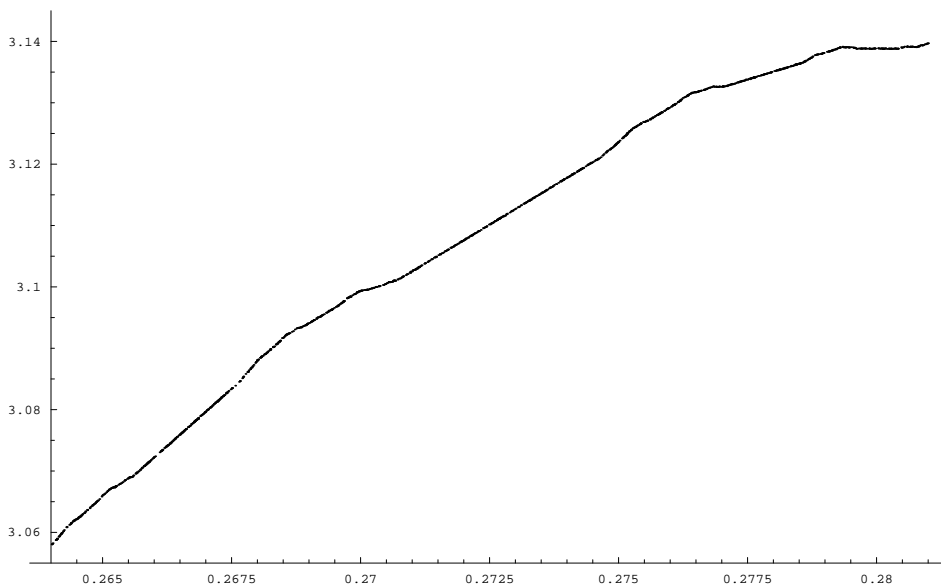
FIGURE 6. The entropy of the map T_\alpha at 1600 uniformly distributed values of \alpha from 0.265 to 0.281. The estimated error is less than 1.5 \cdot 10^{-4} .
