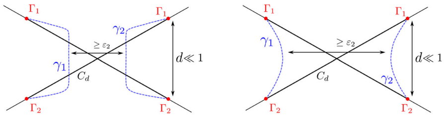
Fig. 10 Two possible critical points \gamma of \text{Area}_s in dimension 2 with \partial\gamma = \Gamma_1 \cup \Gamma_2 are shown with dashed lines and the cone C_d defined in (3.7) is shown with crossed lines. On the right, \gamma does not intersect with C_d except at their boundaries \Gamma_1 and \Gamma_2 . In both figures, two distinct connected components \gamma_1 and \gamma_2 of \gamma are placed at mutually positive distance of at least \varepsilon_2 > 0
