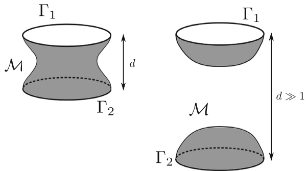
Fig. 2 Possible critical points of \text{Area}_s when N \geq 3 in Theorems 1.2 and 1.4 on the left and in Theorem 1.5 on the right
