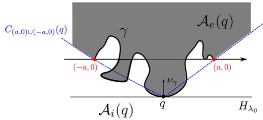
Fig. 3 The situation in dimension 2 in which the critical point \mathcal{M} = \gamma is a C^{1,\alpha} curve with \partial\gamma = \Gamma_0 = \{(a, 0), (-a, 0)\} . The set \mathcal{A}_e(q) is shown in dark gray, the set \mathcal{A}_i(q) in white. The dashed lines represent the boundary of the cone C_{(a,0)\cup(-a,0)}(q)
