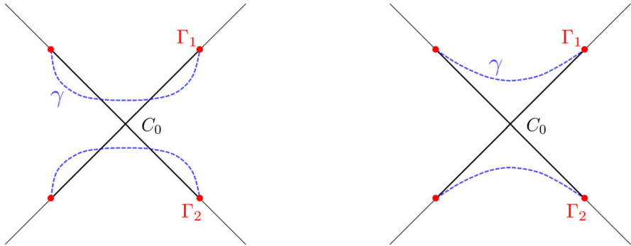
Fig. 6 Possible minimizers \gamma of \text{Area}_s in dimension 2 with \partial\gamma = \Gamma_1 \cup \Gamma_2 is shown with dashed lines. On the right, \gamma does not intersect with C_0 except at their boundaries \Gamma_1 and \Gamma_2
