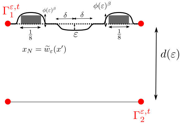
Fig. 8 The barrier \mathcal{M}^{\varepsilon,t} = \mathcal{M}_1^{\varepsilon,t} \cup \mathcal{M}_2^{\varepsilon,t} associated with a function \tilde{w}_\varepsilon in dimension 2. The graph of \tilde{w}_\varepsilon in \{|x'| < 1\} is depicted with black lines and the cylinders in dark gray
