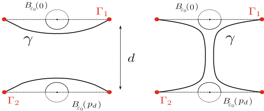
Fig. 1 Two possible situations in dimension 2 in Lemma 1.3 in which the “interior” or “exterior” of the critical point \mathcal{M} = \gamma with \partial\mathcal{M} = \Gamma_1 \cup \Gamma_2 contains two half-balls
