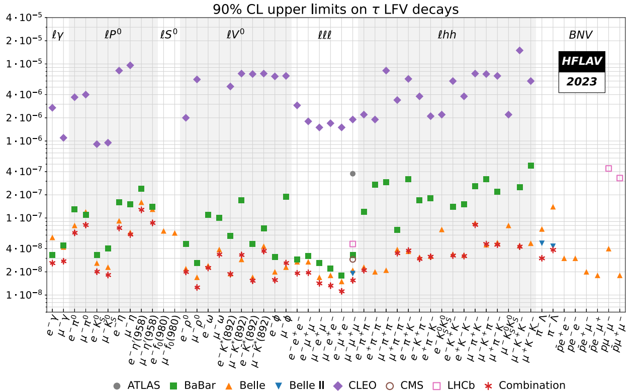
FIG. 68. Tau lepton-flavor-violating branching fraction upper limits and combinations. In order to appreciate the physics reach improvement over time, the plot includes also the CLEO upper limits reported by PDG 2022 [302].
