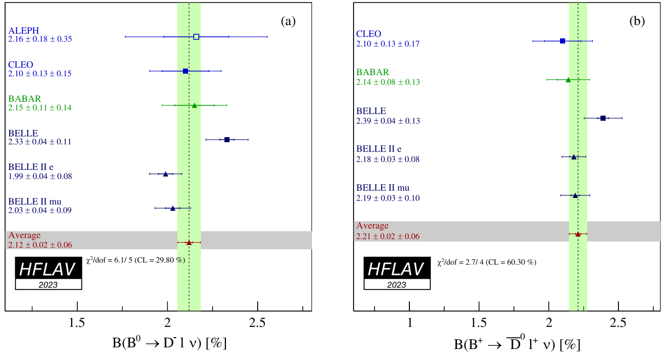
FIG. 14. Branching fractions of exclusive semileptonic B decays: (a) \bar{B}^0 \rightarrow D^+ \ell^- \bar{\nu}_\ell (Table 30) and (b) B^- \rightarrow D^0 \ell^- \bar{\nu}_\ell (Table 31).
