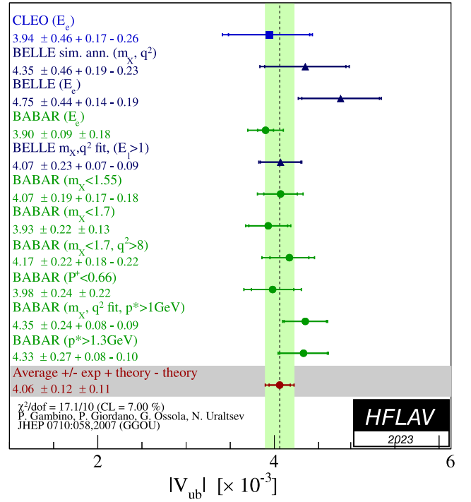
FIG. 25. Measurements of |V_{ub}| from inclusive semileptonic decays and their average based on the GGOU prescription. The labels indicate the variables and selections used to define the signal regions in the different analyses.
