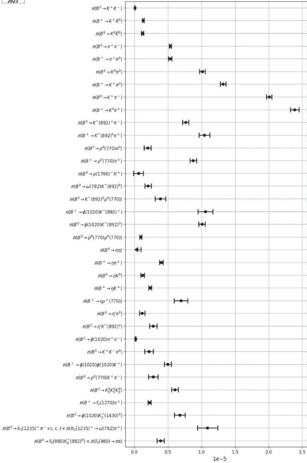
FIG. 29. A selection of high-precision measurements of Branching Fractions of B -meson decays into charmless mesonic final states.
