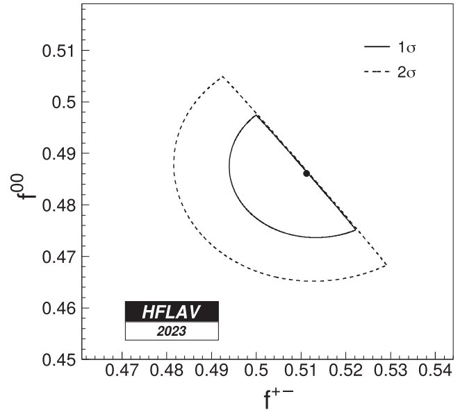
FIG. 4. The f^{00} and f^{+-} plane with the HFLAV fit results. The dot shows the central values, the solid and dashed curves show the 1\sigma (68% CL) and 2\sigma (95% CL) contours, respectively.
