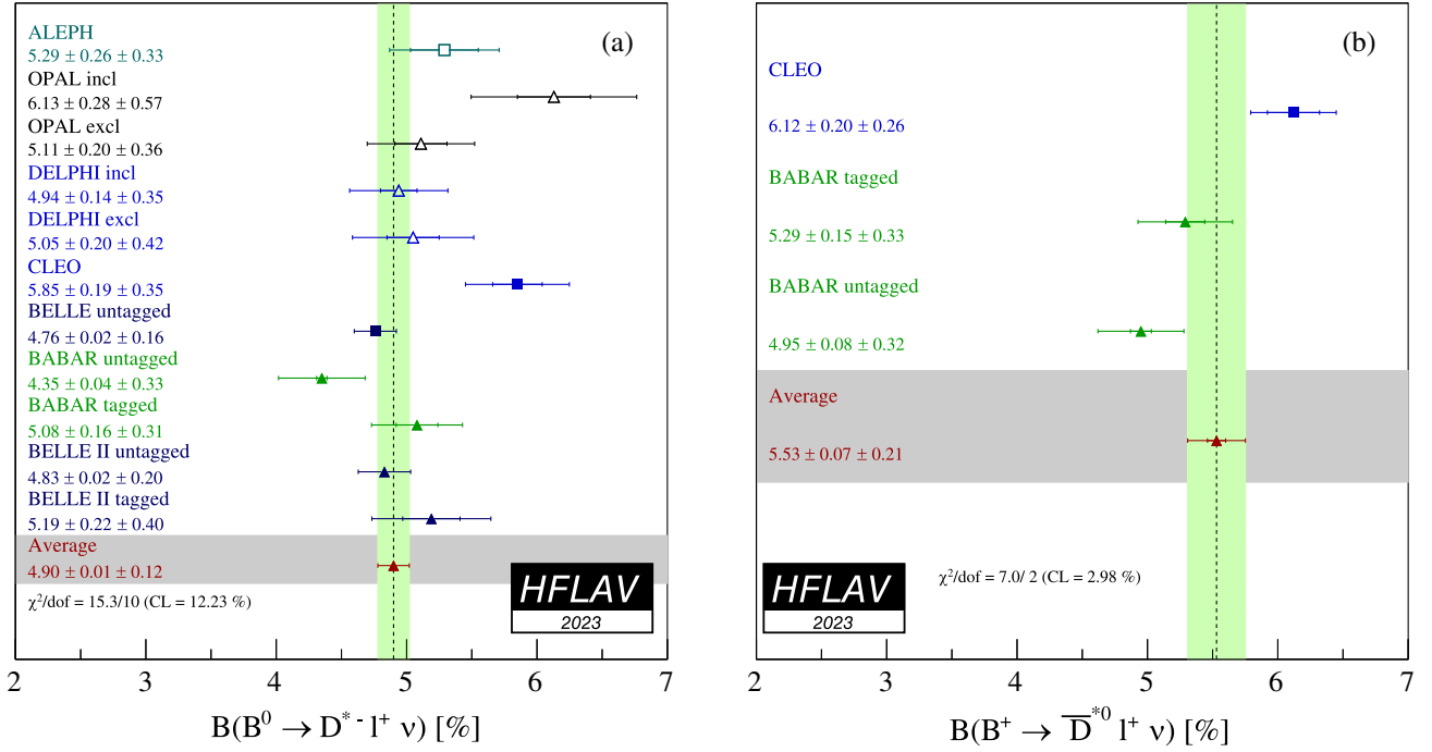
FIG. 11. Branching fractions of exclusive semileptonic B decays: (a) \bar{B}^0 \rightarrow D^{*+} \ell^- \bar{\nu}_\ell (Table 23) and (b) B^- \rightarrow D^{*0} \ell^- \bar{\nu}_\ell (Table 24).
