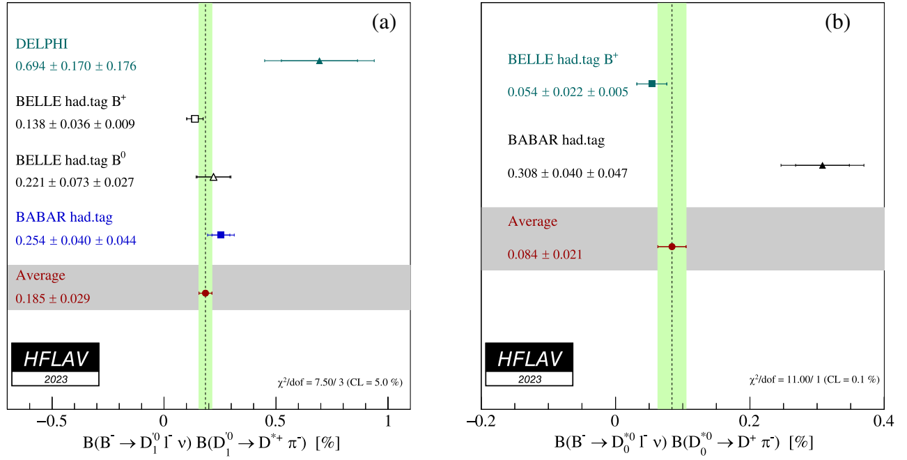
FIG. 18. Rescaled individual measurements and their averages for (a) B(B^- \rightarrow D_1^0 \ell^- \bar{\nu}_\ell) \times B(D_1^0 \rightarrow D^{*+} \pi^-) and (b) B(B^- \rightarrow D_0^{*0} \ell^- \bar{\nu}_\ell) \times B(D_0^{*0} \rightarrow D^+ \pi^-) .
