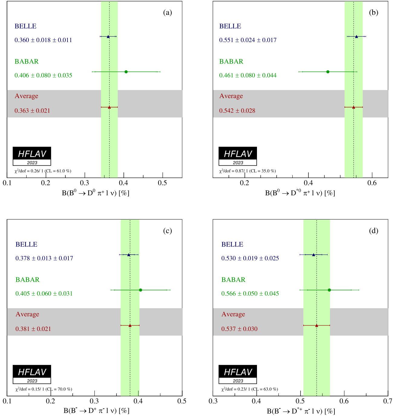
FIG. 16. Average branching fraction of exclusive semileptonic B decays (a) \bar{B}^0 \rightarrow D^0 \pi^+ \ell^- \bar{\nu}_\ell , (b) \bar{B}^0 \rightarrow D^{*0} \pi^+ \ell^- \bar{\nu}_\ell , (c) B^- \rightarrow D^+ \pi^- \ell^- \bar{\nu}_\ell , and (d) B^- \rightarrow D^{*+} \pi^- \ell^- \bar{\nu}_\ell . The corresponding individual results are also shown.
