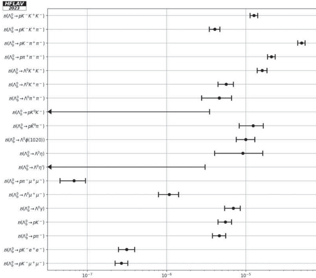
FIG. 32. Branching fractions of charmless \Lambda_b^0 decays.
