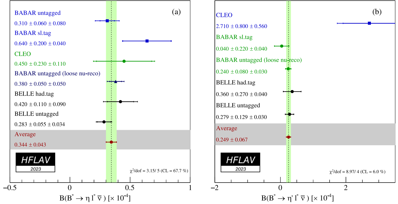
FIG. 23. (a) Summary of exclusive determinations of \mathcal{B}(B^+ \rightarrow \eta \ell^+ \nu) and their average. (b) Summary of exclusive determinations of \mathcal{B}(B^+ \rightarrow \eta' \ell^+ \nu) and their average.
