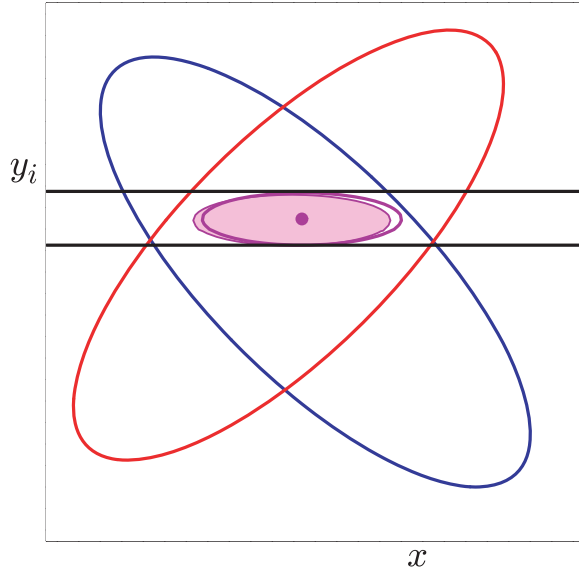
FIG. 3. Illustration of the combination of two hypothetical measurements of x using the method described in the text. The ellipses represent the unconstrained likelihoods of each measurement, and the horizontal band represents the latest knowledge about y_i that is used to adjust the individual measurements. The filled small ellipse shows the result of the exact method using \mathcal{L}_{\text{comb}} , and the hollow small ellipse and dot show the result of the approximate method using \chi^2_{\text{comb}} .
