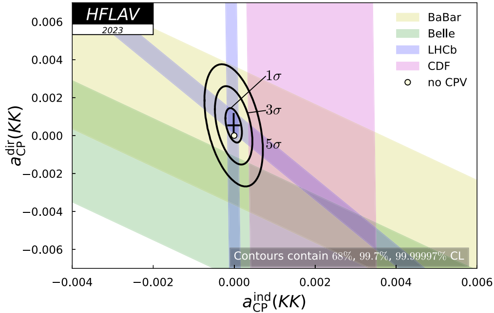
FIG. 48. Plot of data and the fit result for a_{CP}^{\text{dir}}(KK) and a_{CP}^{\text{ind}}(KK) . Individual measurements are plotted as bands showing their \pm 1\sigma range. The no- CPV point (0,0) is shown as a filled circle, and the best fit value is indicated by a cross showing the one-dimensional uncertainties. Two-dimensional 1\sigma (68.3% CL), 3\sigma (99.7% CL), and 5\sigma (99.99997% CL) regions are plotted as ellipses.
