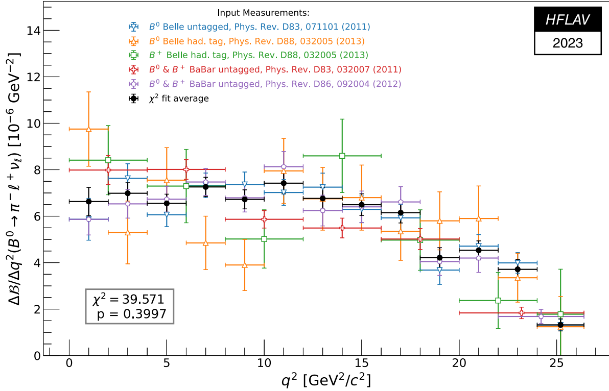
FIG. 19. The B \rightarrow \pi \ell \nu q^2 spectrum measurements and the average spectrum obtained from the likelihood combination (shown in black).
