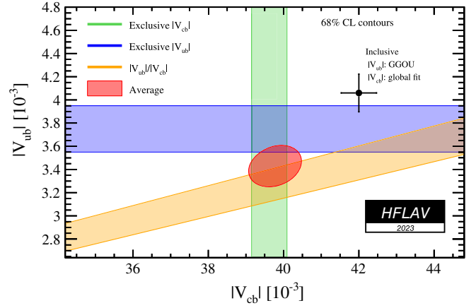
FIG. 26. Combined average on |V_{ub}| and |V_{cb}| including the LHCb measurements of |V_{ub}|/|V_{cb}| from \Lambda_b^0 \rightarrow p\mu^-\bar{\nu}_\mu and \bar{B}_s^0 \rightarrow K\mu^-\bar{\nu}_\mu decays, the exclusive |V_{ub}| measurement from \bar{B} \rightarrow \pi\ell^-\bar{\nu}_\ell , and the |V_{cb}| average from \bar{B} \rightarrow D\ell^-\bar{\nu}_\ell , \bar{B} \rightarrow D^*\ell^-\bar{\nu}_\ell and \bar{B}_s^0 \rightarrow D_s^{(*)}\mu^-\bar{\nu}_\mu measurements. The point with the error bars corresponds to the inclusive |V_{cb}| from Ref. [61], and the inclusive |V_{ub}| from GGOU calculation (Sec. VID 3).
