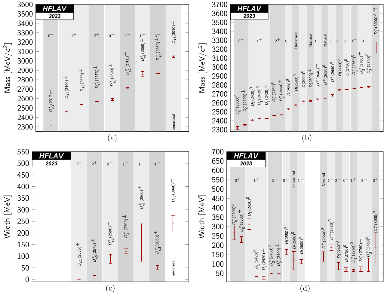
FIG. 58. (a) Average masses for excited D_s mesons; (b) average masses for excited D mesons; (c) average widths for excited D_s mesons; (d) average widths for excited D mesons. The vertical shaded regions distinguish between different spin-parity states.
