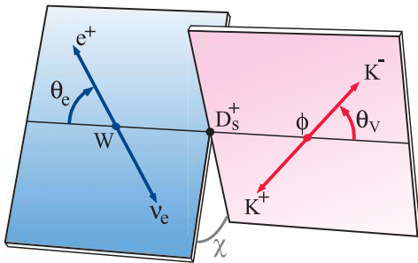
FIG. 51. Decay angles \theta_V , \theta_\ell and \chi . Note that the angle \chi between the decay planes is defined in the D -meson reference frame, whereas the angles \theta_V and \theta_\ell are defined in the V meson and W reference frames, respectively.
