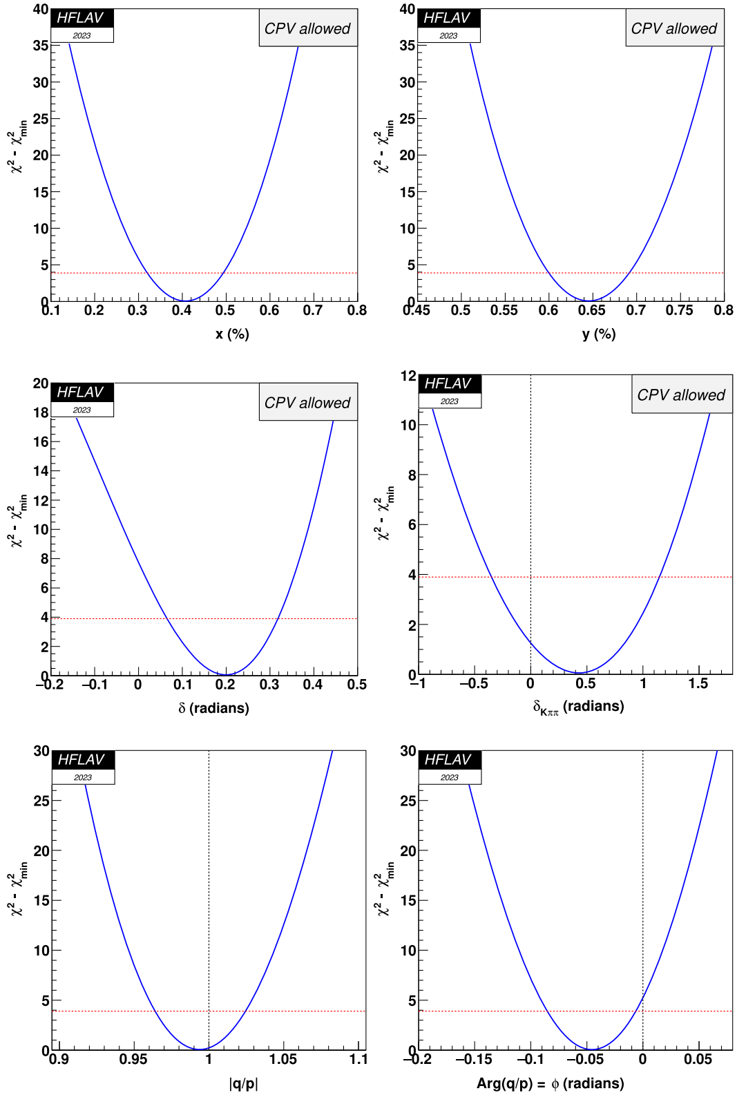
FIG. 46. The function \Delta\chi^2 = \chi^2 - \chi_{\min}^2 for parameters x , y , \delta , \delta_{K\pi\pi} , |q/p| , and \phi , from Fit #3. The points where \Delta\chi^2 = 3.84 (denoted by dashed horizontal lines) determine 95% CL intervals.
