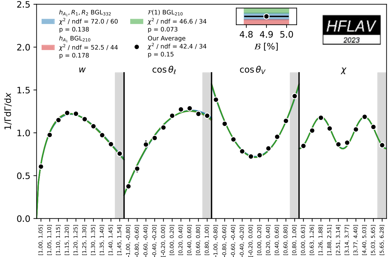
FIG. 13. The fitted \bar{B} \rightarrow D^* \ell^- \bar{\nu}_\ell differential decay rate from our averaged normalized differential distribution and our isospin average of the \bar{B} \rightarrow D^* \ell^- \bar{\nu}_\ell branching fraction. We find consistent fitted shapes in all three considered scenarios.
