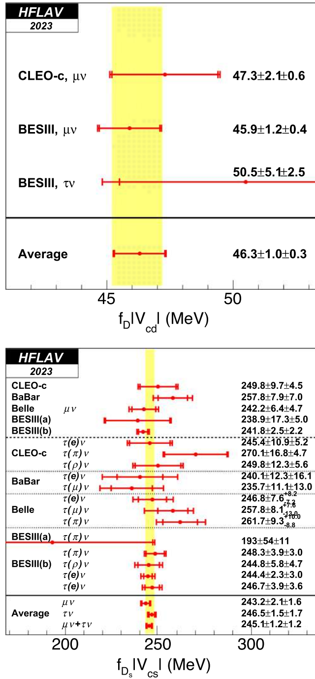
FIG. 52. WA values for f_D|V_{cd}| (top) and f_{D_s}|V_{cs}| (bottom). For each point, the first errors are statistical and the second errors are systematic. BESIII(a) represents results based on 0.48 \text{ fb}^{-1} of data recorded at \sqrt{s} = 4.009 \text{ GeV} [1310], and BESIII(b) represents results based on 7.33 (or 6.32 ) \text{fb}^{-1} of data recorded at \sqrt{s} = 4.128\text{--}4.226 \text{ GeV} [1304,1305,1307,1308].
