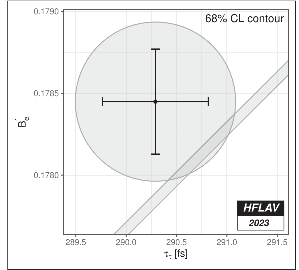
FIG. 66. Test of the universality of the couplings of the lighter leptons e and \mu , assumed to be the same, and of the \tau lepton. The plot shows values and uncertainties of the \tau lifetime and of \mathcal{B}'_e , a determination of the electronic \tau branching fractions obtained from the direct measurements of the electronic and the muonic \tau branching fractions. The contour delimits the 68% CL region. The oblique band shows the Standard Model prediction of \mathcal{B}'_e as a function of the \tau lifetime, and its width is mainly determined by the uncertainty on the \tau mass.
