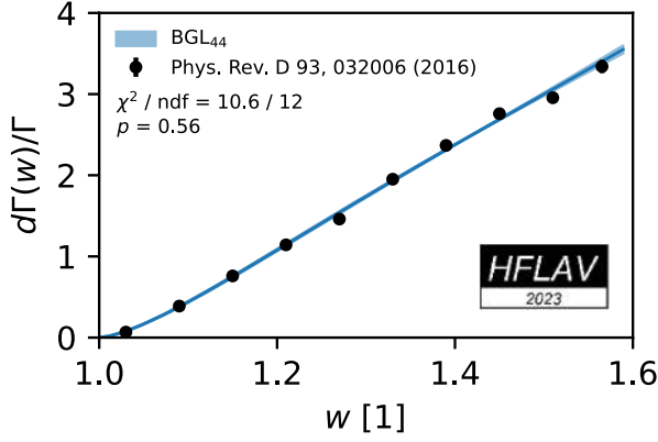
FIG. 15. The fitted \bar{B} \rightarrow D\ell^-\bar{\nu}_\ell differential decay rate and our isospin average of the \bar{B} \rightarrow D\ell^-\bar{\nu}_\ell branching fraction.
