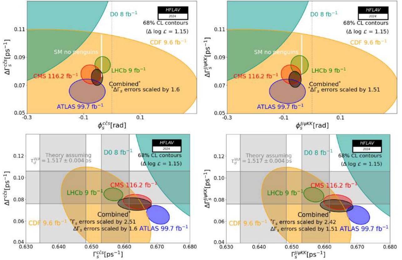
FIG. 9. Regions at 68% CL shown in the (\phi_s^{ccs}, \Delta\Gamma_s) plane on the top and in the (\Gamma_s, \Delta\Gamma_s) plane on the bottom, for individual experiments and their combination. The left plots are obtained from all CDF [208], D0 [209], ATLAS [210–212], CMS [213,214] and LHCb [110,215–219,258,260,261] measurements of B_s^0 \rightarrow J/\psi K^+ K^- , B_s^0 \rightarrow \psi(2S) K^+ K^- , B_s^0 \rightarrow J/\psi \pi^+ \pi^- and B_s^0 \rightarrow D_s^+ D_s^- decays, while the right plots are obtained from B_s^0 \rightarrow J/\psi K^+ K^- measurements only [208–215,218,219]. The expectations within the Standard Model neglecting penguin contributions [47,204,205] are shown as white rectangles in the top plots. The \Gamma_s theory value in the bottom plots is calculated from Ref. [47] assuming the experimental world average for the B^0 lifetime, 1.517 \pm 0.004 \text{ ps} . The two solutions in \Gamma_s are due to the two different sets of inputs to the theory calculation of \tau(B_s^0)/\tau(B^0) according to Ref. [62] (toward lower \Gamma_s values) and Ref. [63] (toward higher \Gamma_s values).
