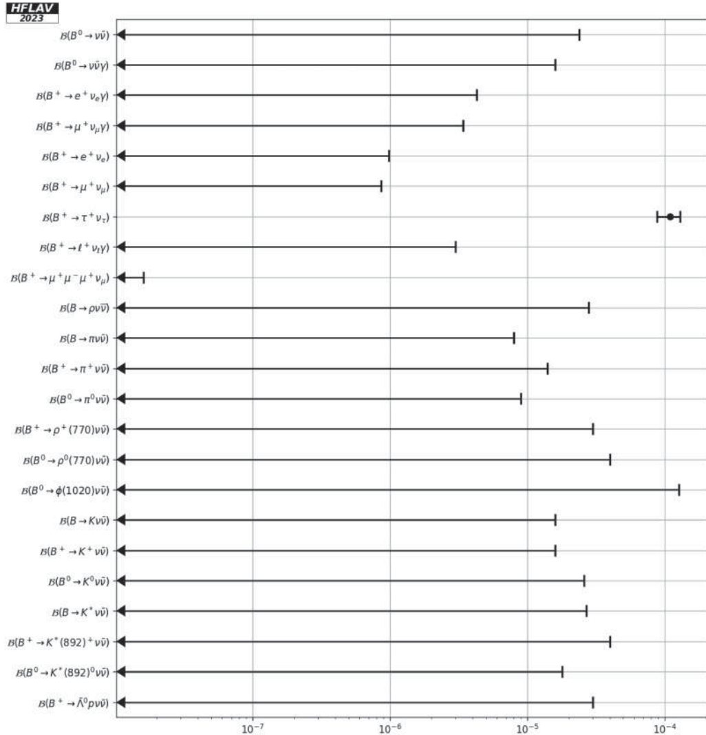
FIG. 40. Branching fractions of charmless B decays with neutrinos.
