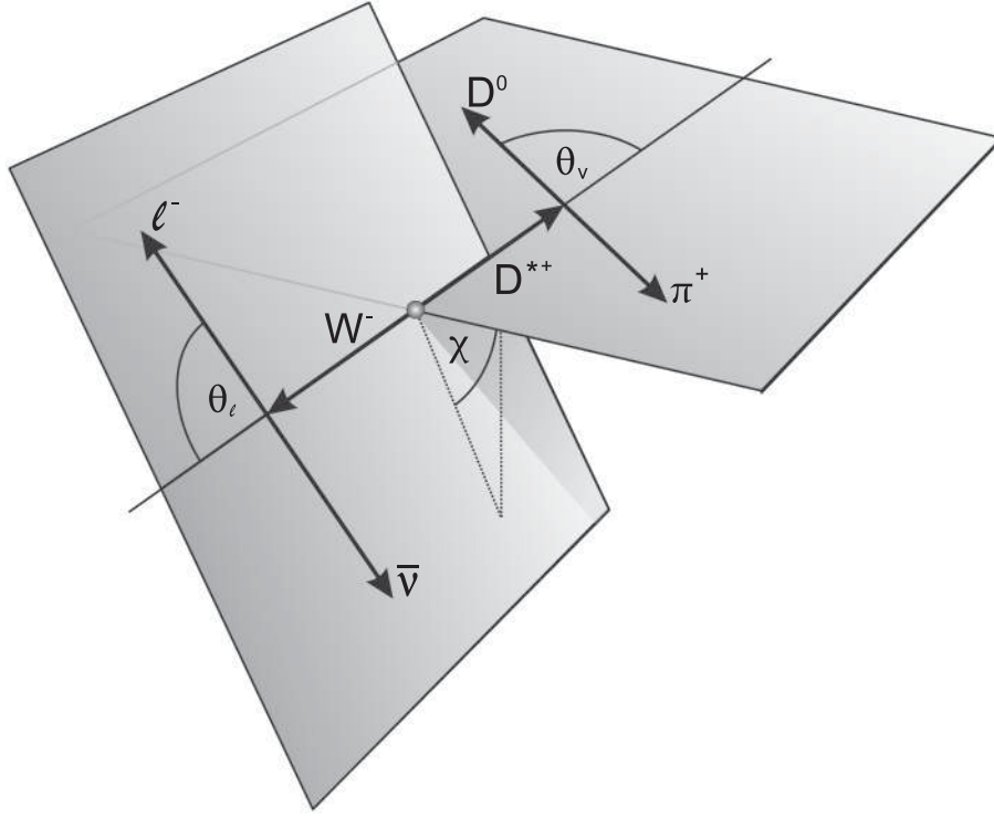
FIG. 10. Sketch of the helicity angles \theta_\ell , \theta_V and \chi in the decay \bar{B} \rightarrow D^* \ell^- \bar{\nu}_\ell .
