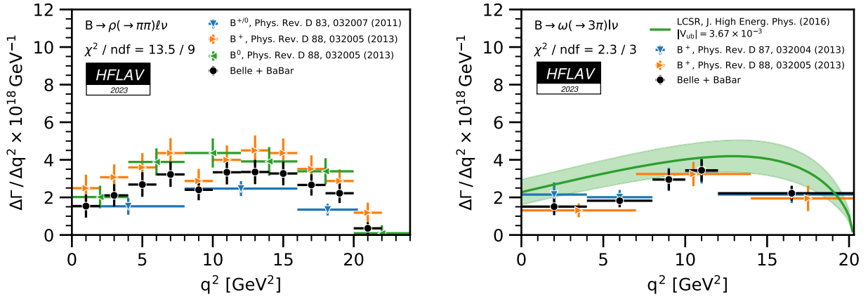
FIG. 22. The averaged q^2 spectrum of the measurements listed in the text for the \rho (left) and \omega (right) final state on top of the latest Belle and BABAR measurements. The isospin transformation is applied to the B^0 \rightarrow \rho^- \ell^+ \nu measurements. In the right figure we also show the model (green band) which was used to split the bins in the averaging procedure.
