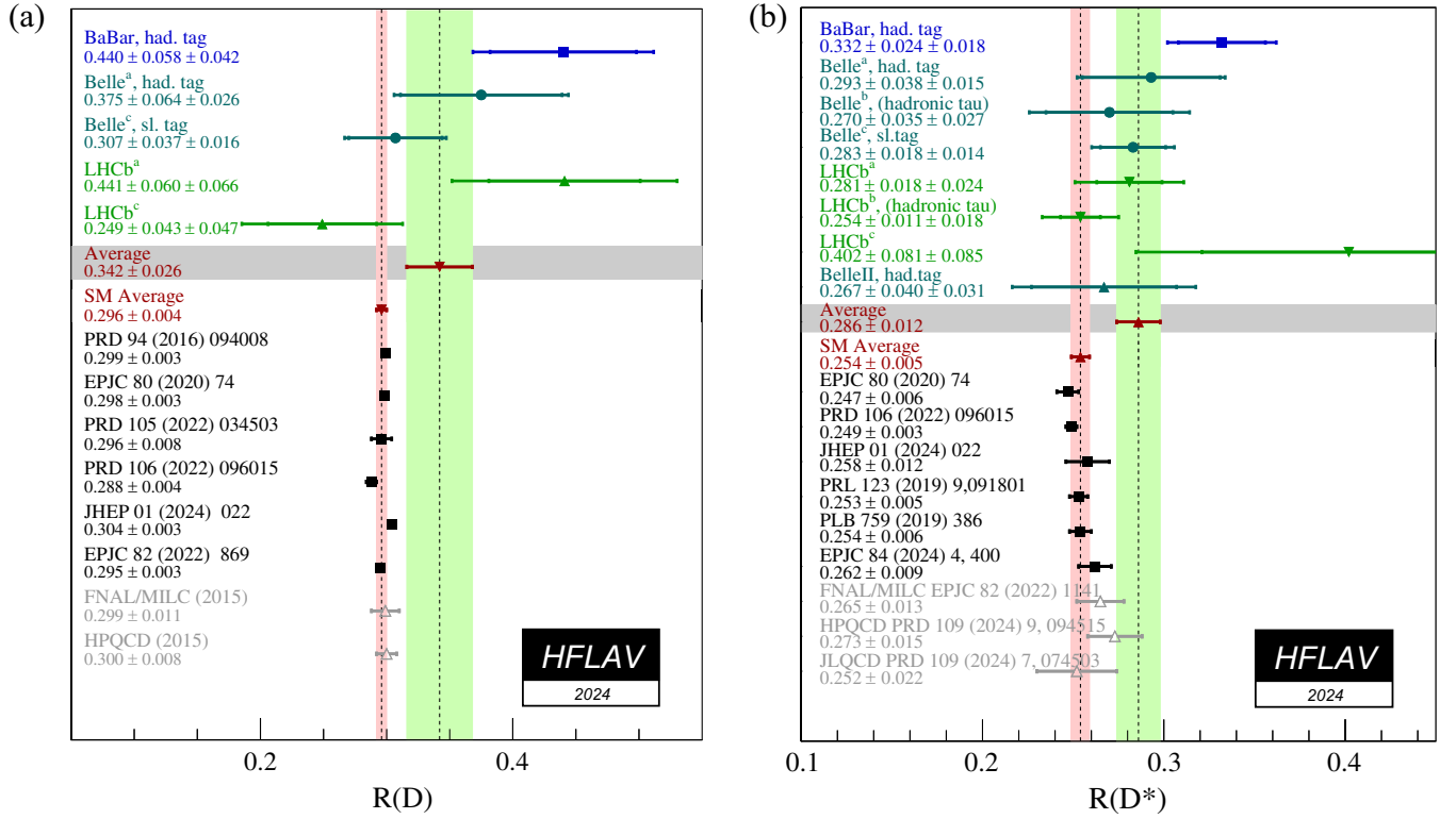
FIG. 28. (a) Measurements of \mathcal{R}(D) and (b) \mathcal{R}(D^*) . The green (right) vertical bands are the averages obtained from the combined fit. The red (left) vertical bands are the averages of the theoretical predictions obtained as explained in the text. The theory predictions represented in gray, are based on LQCD only and are shown for comparison but not included in the SM averages.
