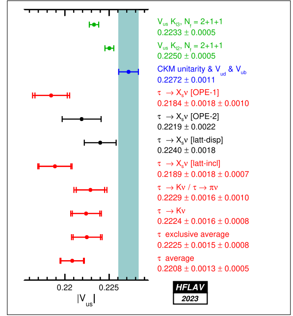
FIG. 67. |V_{us}| determinations. The values of |V_{us}|_{K\ell 3} , |V_{us}|_{K\ell 2} and the expected |V_{us}| from the CKM matrix unitarity are taken from Ref. [1589]. The other reported |V_{us}| values are documented in the text. When two uncertainties are reported, the first one accounts for the uncertainties of the HFLAV-Tau fit results, and the second one accounts for the uncertainties of the theory and the other inputs that are used for the |V_{us}| determinations.
