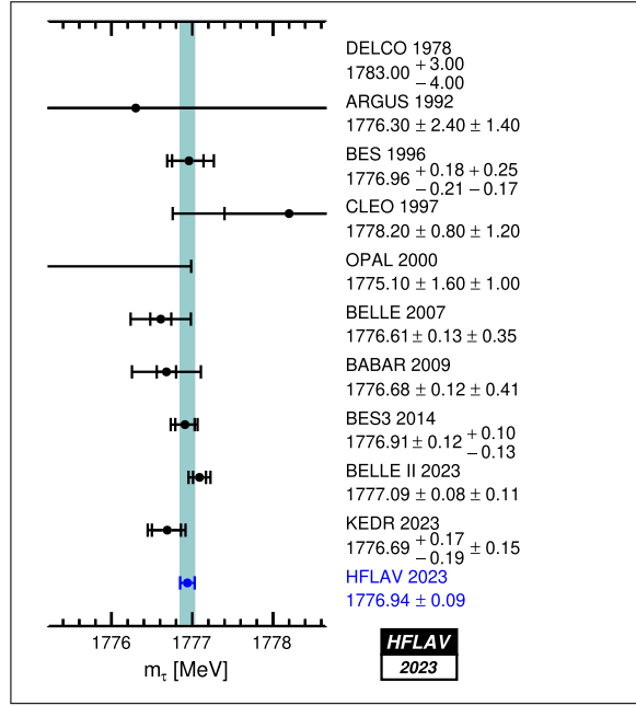
FIG. 64. \tau mass measurements and their average.
