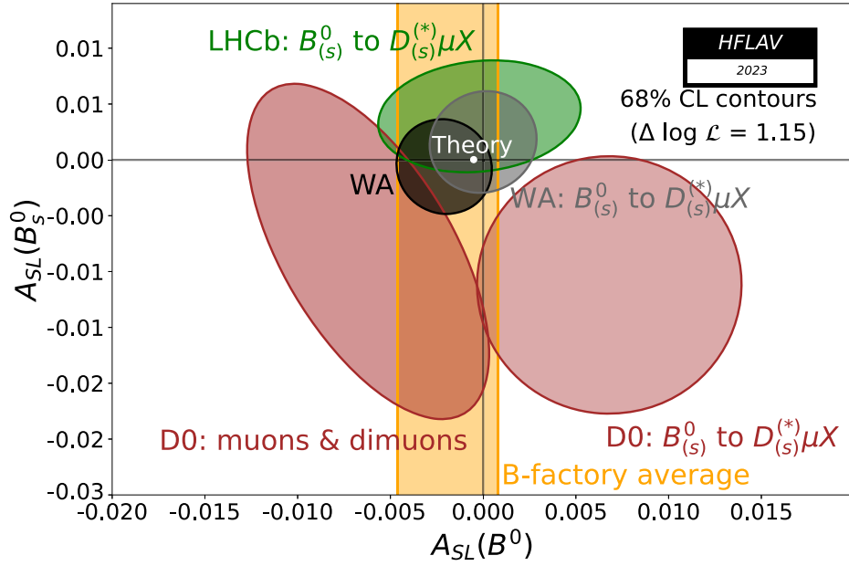
FIG. 8. Measurements of \mathcal{A}_{\text{SL}}^d and \mathcal{A}_{\text{SL}}^s listed in Table 19 ( B -factory average as the orange band, D0 measurements as the brown ellipses, LHCb measurements as the green ellipse) together with their two-dimensional average (black ellipse). The gray ellipse is showing the average from D0 and LHCb results using only untagged B_{(s)}^0 \rightarrow D_{(s)}^{(*)-} \mu^+ \nu X decays. The white point close to (0,0) is the Standard Model prediction of Ref. [47]. The prediction and the experimental world average are consistent with each other at the level of 0.5\sigma .
