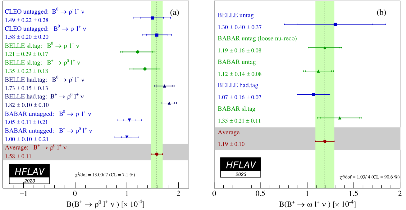
FIG. 21. (a) Summary of exclusive determinations of \mathcal{B}(B^+ \rightarrow \rho^0 \ell^+ \nu) and their average. Measurements of B^0 \rightarrow \rho^- \ell^+ \nu branching fractions have been scaled by 0.5\tau_{B^+}/\tau_{B^0} in accordance with isospin symmetry. (b) Summary of exclusive determinations of B^+ \rightarrow \omega \ell^+ \nu and their average.
