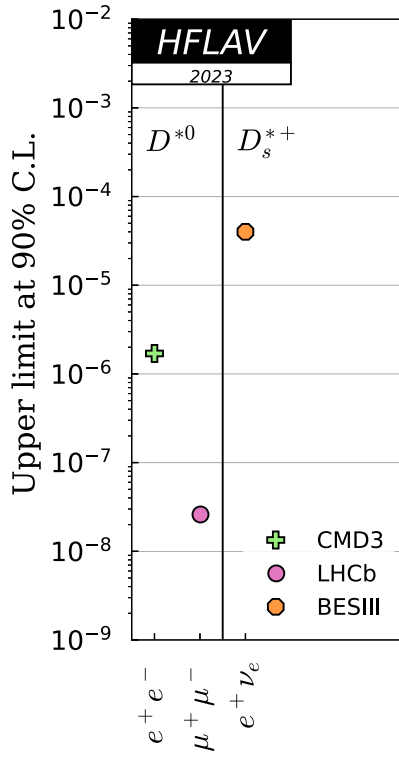
FIG. 62. Upper limits at 90% CL for D^{*0} and D_s^{*+} decay branching fractions.
