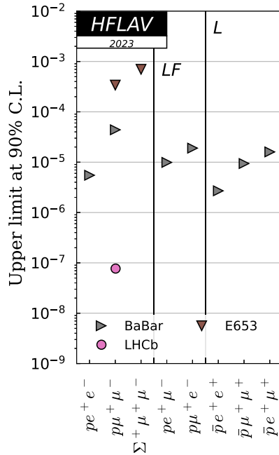
FIG. 63. Upper limits at 90% CL for \Lambda_c^+ decay branching fractions. Shown are flavor-changing neutral current decays, lepton-flavor-changing (LF) decays, and lepton-number-changing (L) decays.
