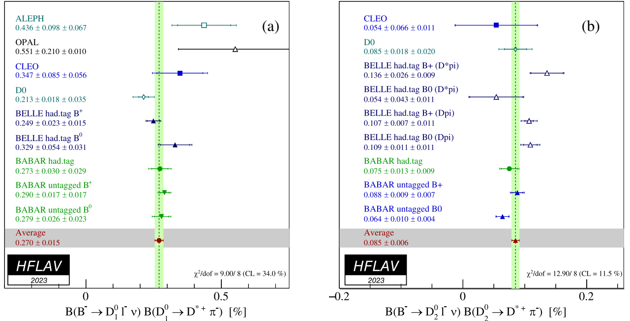
FIG. 17. Rescaled individual measurements and their averages for (a) \mathcal{B}(B^- \rightarrow D_1^0 \ell^- \bar{\nu}_\ell) \times \mathcal{B}(D_1^0 \rightarrow D^{*+} \pi^-) and (b) \mathcal{B}(B^- \rightarrow D_2^0 \ell^- \bar{\nu}_\ell) \times \mathcal{B}(D_2^0 \rightarrow D^{*+} \pi^-) .
