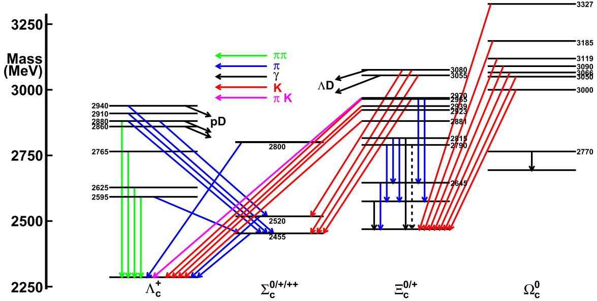
FIG. 59. Level diagram for multiplets and transitions for excited charm baryons.
