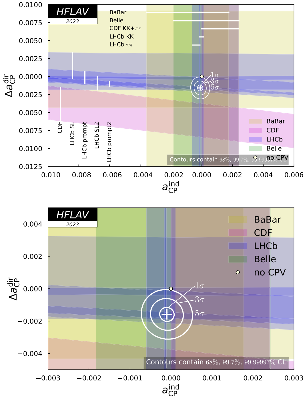
FIG. 47. Top: plot of all data and the fit result for \Delta a_{CP}^{dir} and a_{CP}^{ind} . Individual measurements are plotted as bands showing their \pm 1\sigma range. The no-CPV point (0,0) is shown as a filled circle, and the best fit value is indicated by a cross showing the one-dimensional uncertainties. Two-dimensional 1\sigma (68.3% CL), 3\sigma (99.7% CL), and 5\sigma (99.99997% CL) regions are plotted as ellipses. Bottom: zoom of the same plot, highlighting the best fit region.
