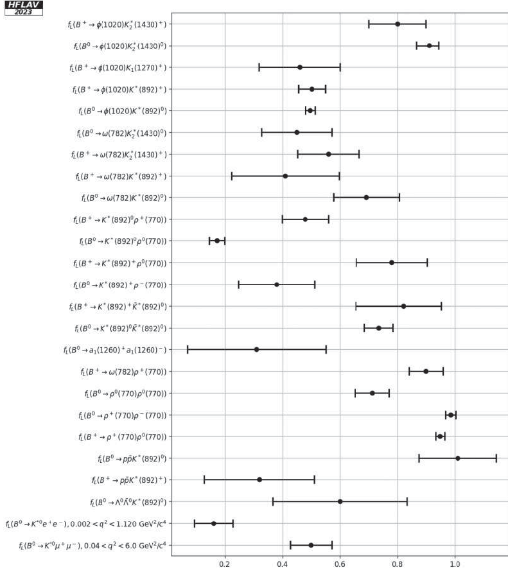
FIG. 42. Longitudinal polarization fraction in charmless B decays.
