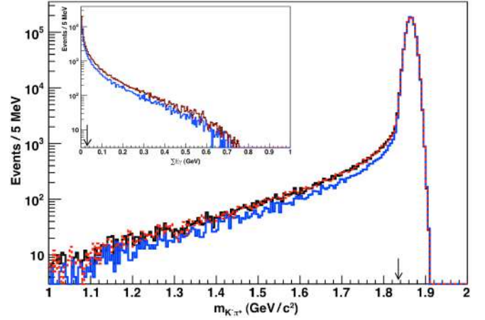
FIG. 54. The K\pi invariant mass distribution for equally-sized samples of D^0 \rightarrow K^- \pi^+ (n\gamma) decays. The three curves correspond to three different configurations of PHOTOS for modeling FSR: version 2.02 without interference (blue/gray), version 2.02 with interference (red dashed) and version 2.15 with interference (black). The true invariant mass has been smeared with a typical experimental resolution of 10 \text{ MeV}/c^2 . Inset: The corresponding spectrum of total energy radiated per event. The arrow indicates the \sum E_\gamma value that begins to shift kinematic quantities outside of the range typically accepted in a measurement.
