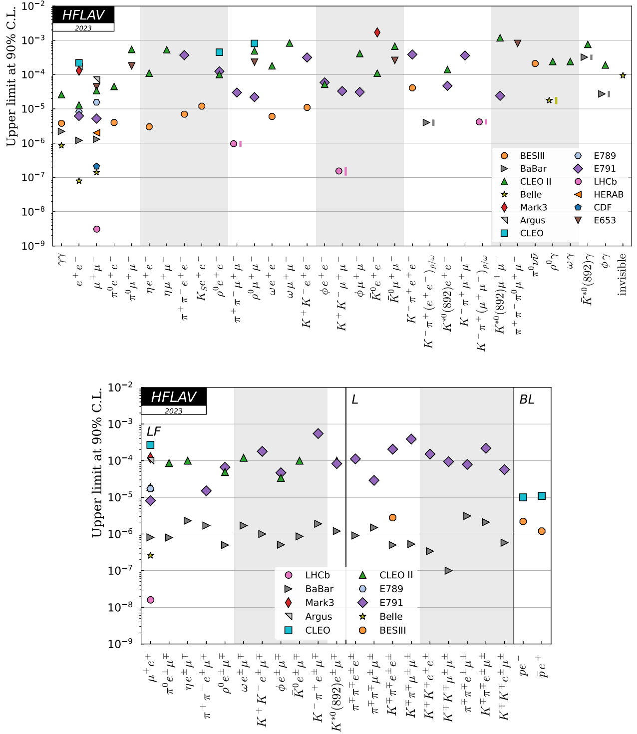
FIG. 60. Upper limits at 90% CL for D^0 decay branching fractions. The top plot shows flavor-changing neutral current and radiative decays, and the bottom plot shows lepton-flavor-changing (LF), lepton-number-changing (L), and both baryon- and lepton-number-changing (BL) decays.
