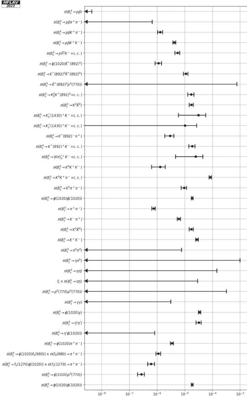
FIG. 34. Branching fractions of charmless nonleptonic B_s^0 decays.
