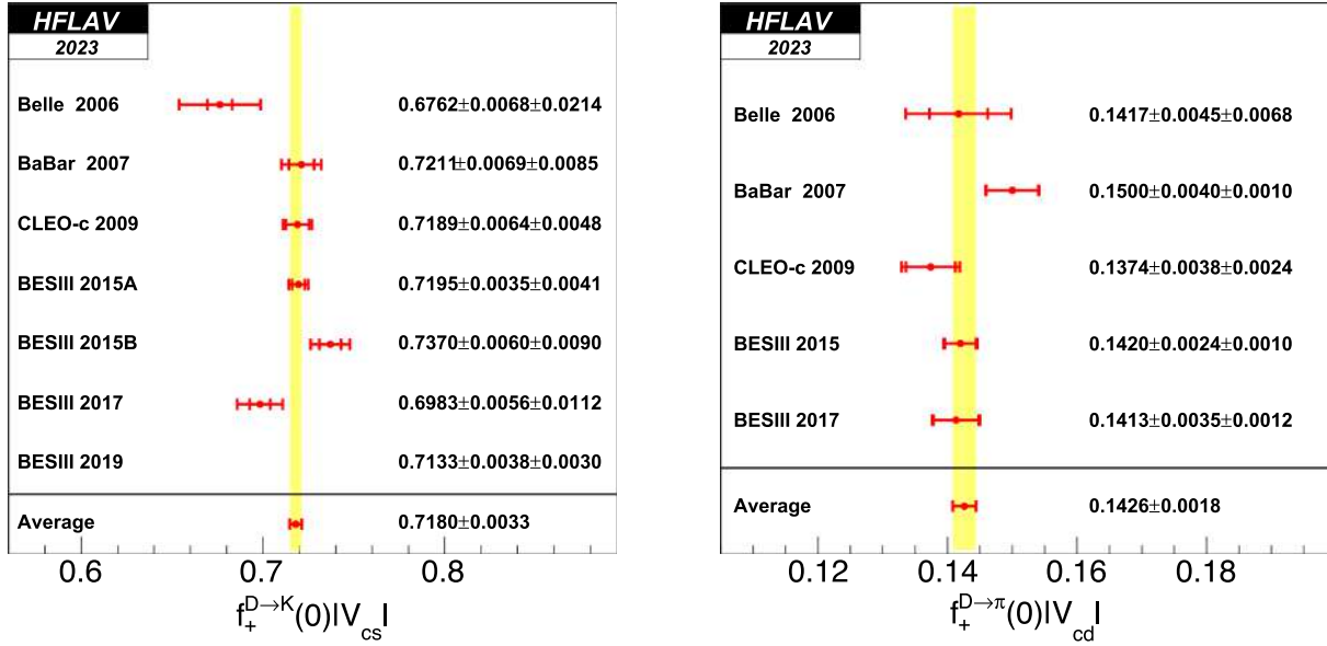
FIG. 49. Comparison of the experimental results of f_+^{D \rightarrow K}(0)|V_{cs}| and f_+^{D \rightarrow \pi}(0)|V_{cd}| .
