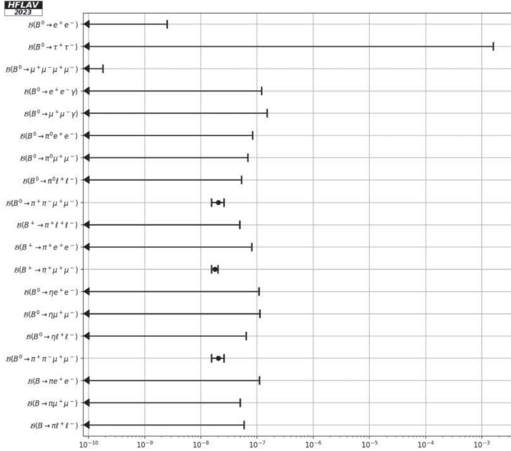
FIG. 36. Branching fractions of B^+ and B^0 decays of the type b \rightarrow u \ell^+ \ell^- , purely leptonic and leptonic radiative.
