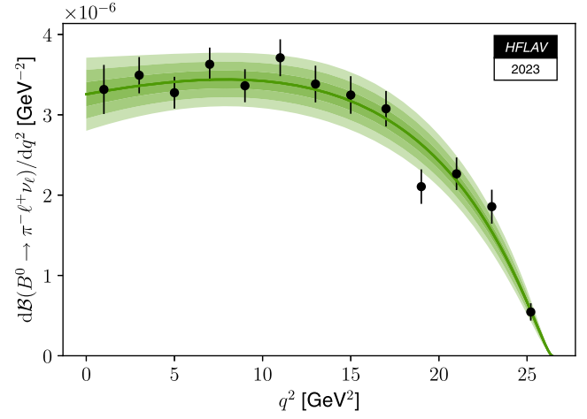
FIG. 20. Fit of the BCL parametrization to the averaged q^2 spectrum from BABAR and Belle and the LQCD calculations. The error bands represent the 1\sigma (dark green), 2\sigma (green), and 3\sigma (light green) uncertainties of the fitted spectrum.
