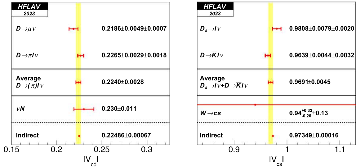
FIG. 53. Comparison of magnitudes of CKM matrix elements |V_{cd}| (left) and |V_{cs}| (right), as determined from leptonic and semileptonic D_{(s)} decays. Also listed are results from neutrino scattering, from W decays, and from a global fit of the CKM matrix assuming unitarity [1315].
