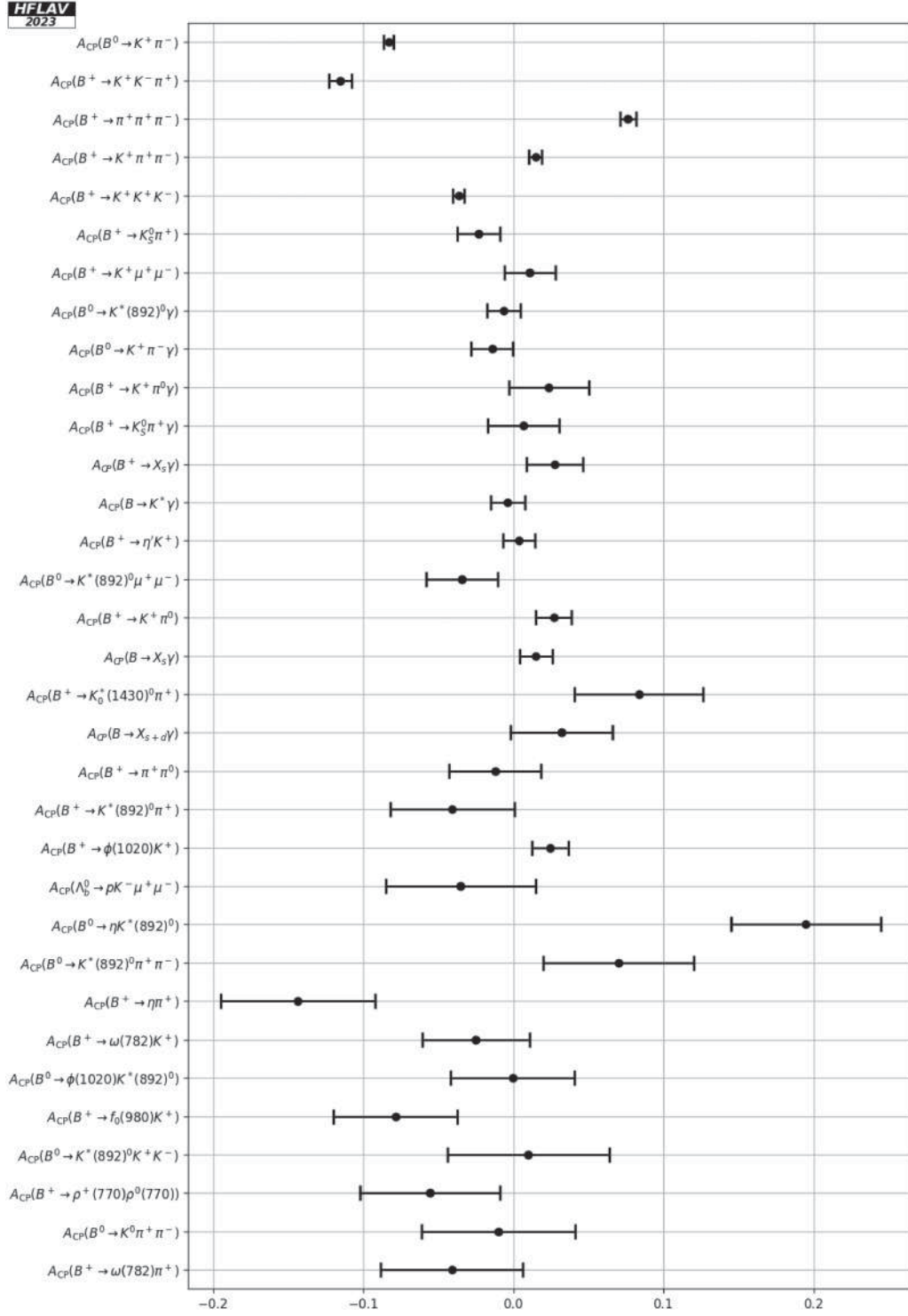
FIG. 41. A selection among the most precise direct CP asymmetries ( A_{CP} ) measured in charmless B^+ and B^0 decay modes.
