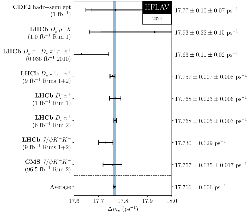
FIG. 7. Measurements of \Delta m_s , together with their average.
