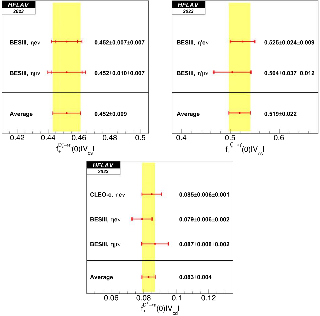
FIG. 50. Comparison of the experimental results of f_+^{D_s^+ \rightarrow \eta}(0)|V_{cs}| , f_+^{D_s^+ \rightarrow \eta'}(0)|V_{cs}| and f_+^{D^+ \rightarrow \eta}(0)|V_{cd}| .
