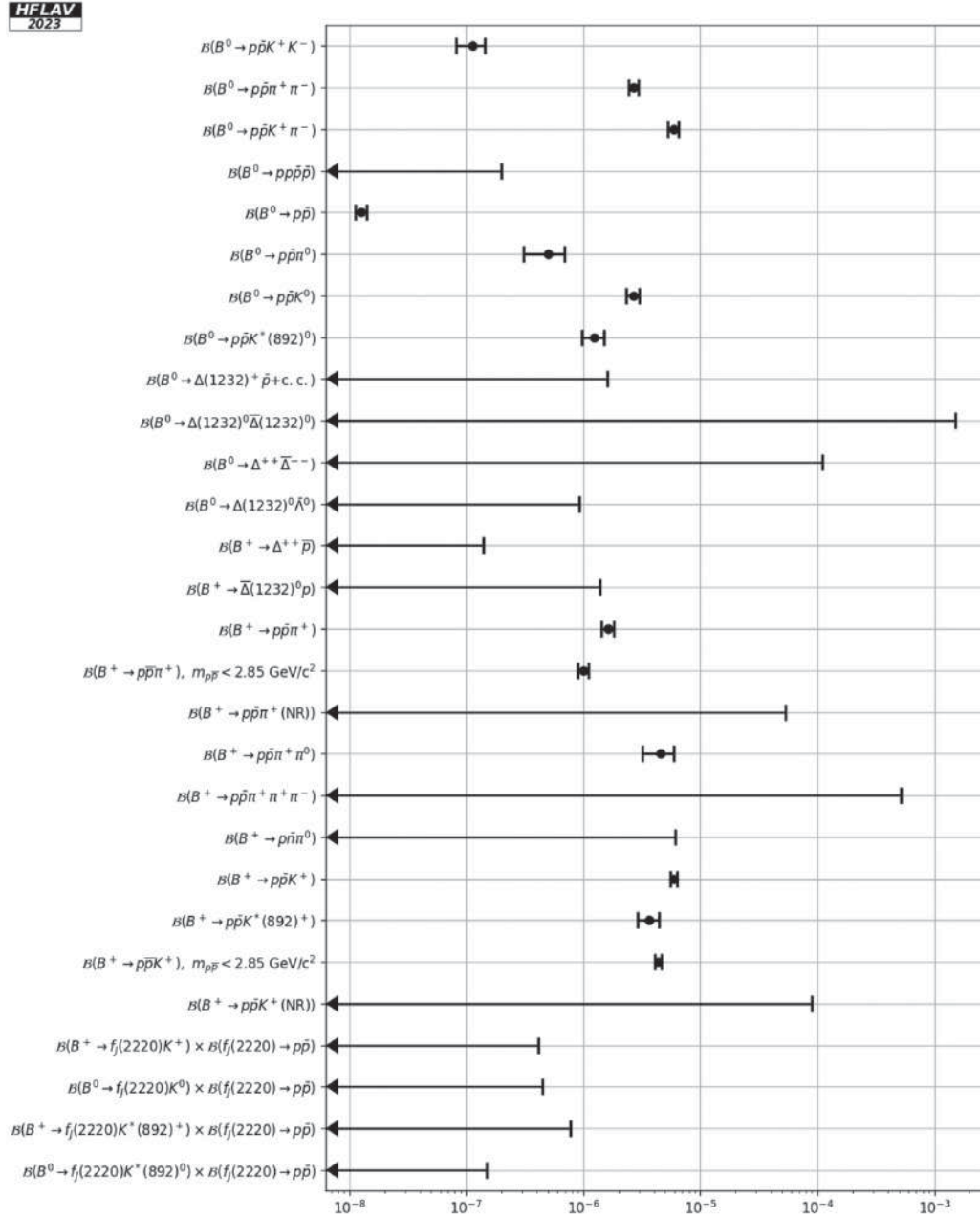
FIG. 30. Branching fractions of charmless B^+ and B^0 decays into nonstrange baryons.
