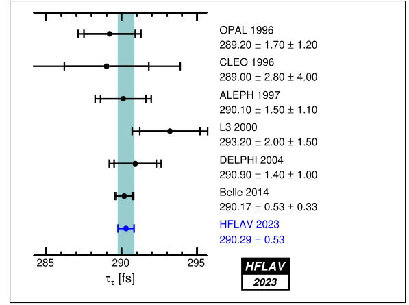
FIG. 65. \tau lifetime measurements and their average.
