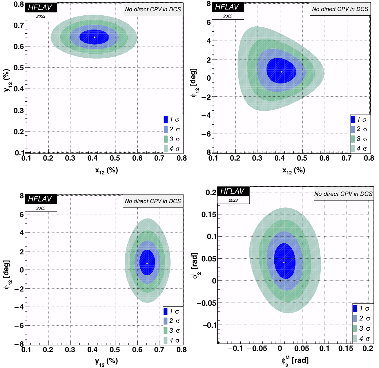
FIG. 44. Two-dimensional contours for parameters (x_{12}, y_{12}) (top left), (x_{12}, \phi_{12}) (top right), and (y_{12}, \phi_{12}) (bottom left), resulting from Fit #1. Contours for (\phi_2^M, \phi_2^\Gamma) resulting from Fit #2 are shown in the bottom right.
