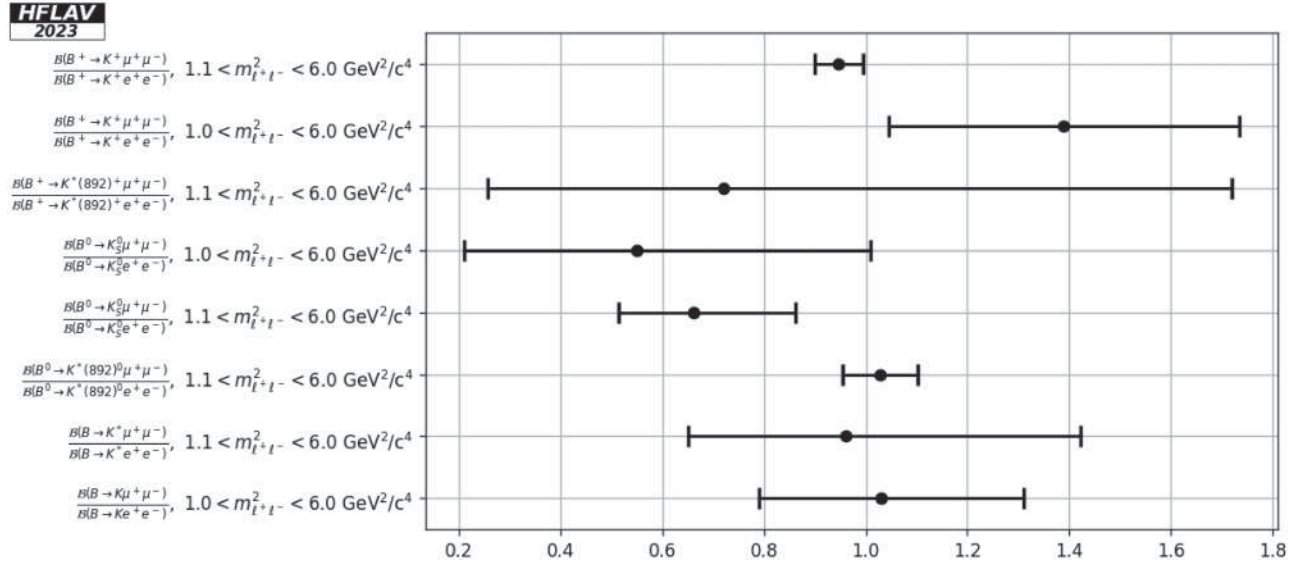
FIG. 37. Compilation of R_K^{(*)} ratios in the low dilepton invariant-mass region. These are ratios between branching fractions of B -meson decays to K^{(*)} \mu^+ \mu^- and K^{(*)} e^+ e^- , which provide information on lepton universality.
