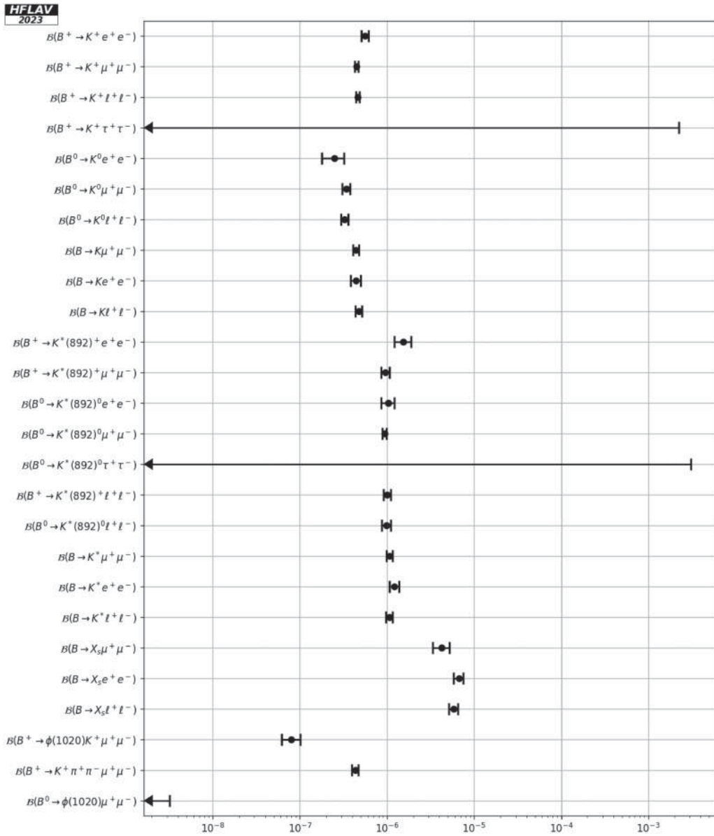
FIG. 35. Branching fractions of B^+ and B^0 decays of the type b \rightarrow s \ell^+ \ell^- .
