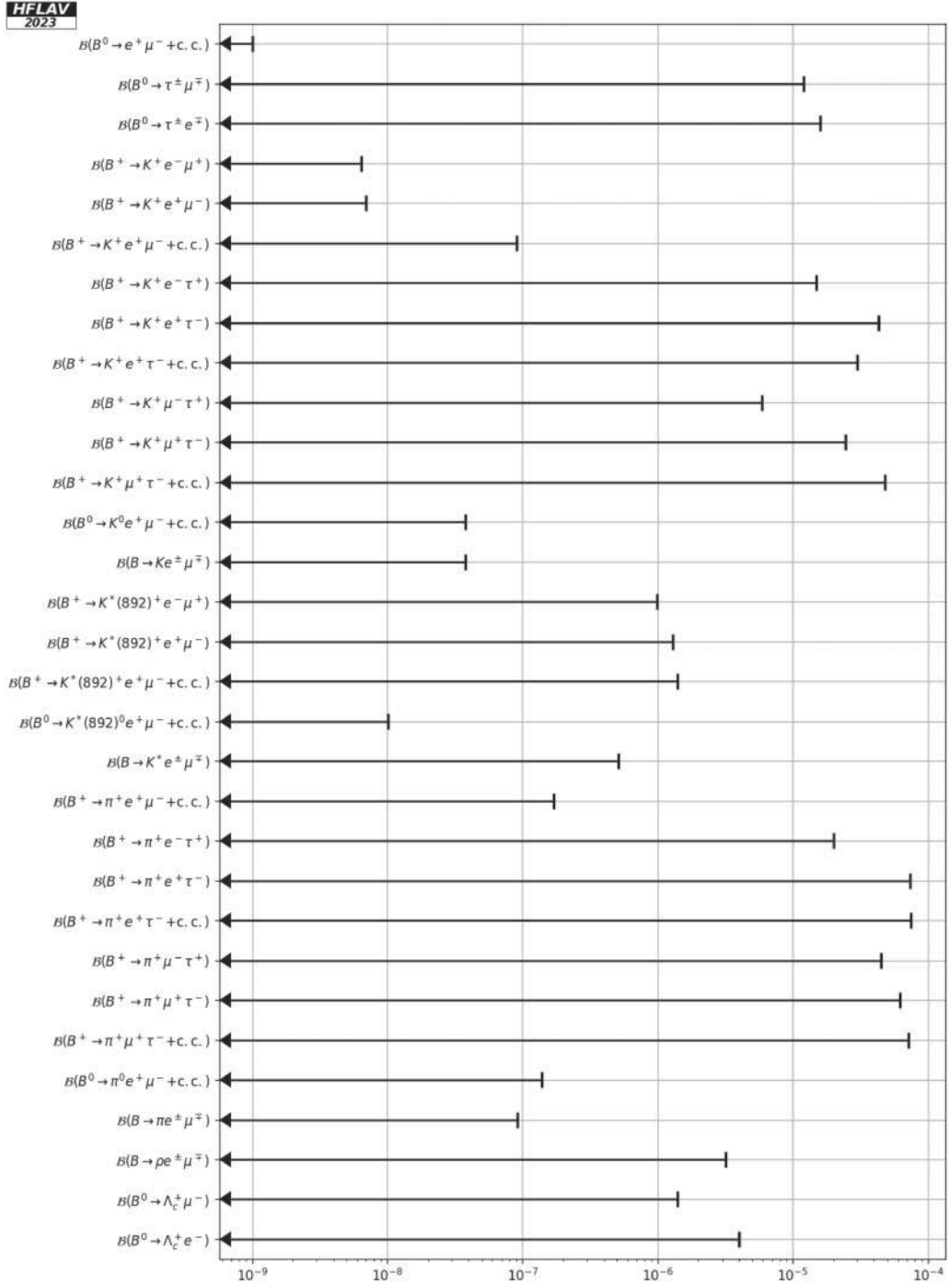
FIG. 38. Limits on branching fractions of lepton-flavor-violating B^+ and B^0 decays.
