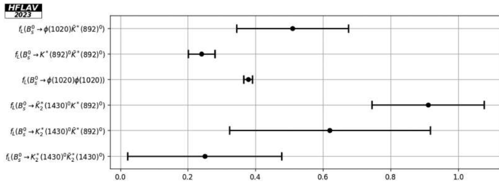
FIG. 43. Longitudinal polarization fraction in charmless B_s^0 decays.
