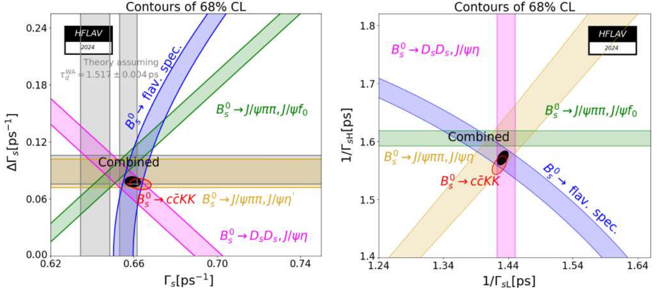
FIG. 6. Contours of 68% CL shown in the (\Gamma_s, \Delta\Gamma_s) plane on the left and in the (1/\Gamma_{sL}, 1/\Gamma_{sH}) plane on the right. The average of all B_s^0 \rightarrow J/\psi K^+ K^- and B_s^0 \rightarrow \psi(2S) K^+ K^- results are shown as the red contour, where \Gamma_s and \Delta\Gamma_s are scaled by factors 2.51 and 1.60. The constraints given by the effective lifetime measurements of B_s^0 to flavor-specific, pure CP -odd and pure CP -even final states are shown as the blue, green and purple bands, respectively. The constraint on \Delta\Gamma_s given by the measurement of the lifetime difference between B_s^0 \rightarrow J/\psi \pi^+ \pi^- and B_s^0 \rightarrow J/\psi \eta' is given by the golden bands. The average taking all constraints into account is shown as the dark-filled contour. The light-gray bands are theory predictions. The horizontal band is \Delta\Gamma_s = +0.091 \pm 0.015 \text{ ps}^{-1} [47] that assumes no new physics in B_s^0 mixing. The vertical \Gamma_s bands are calculated from the two solutions in Ref. [47] assuming the experimental world average for the B^0 lifetime, 1.517 \pm 0.004 \text{ ps} . They are due to the two different sets of inputs to the theory calculation of \tau(B_s^0)/\tau(B^0) according to Ref. [62] (toward lower \Gamma_s values) and Ref. [63] (toward higher \Gamma_s values).
