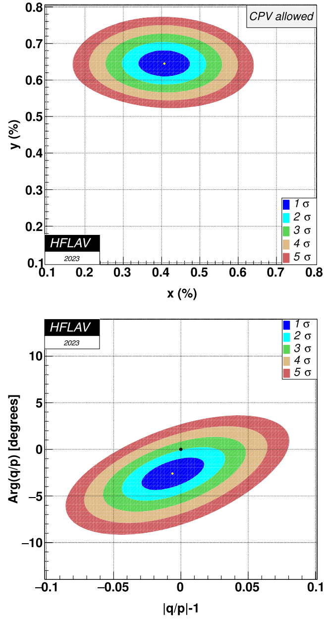
FIG. 45. Two-dimensional contours for parameters (x, y) (upper) and (|q/p| - 1, \phi) (lower), allowing for CPV (Fit #3).
