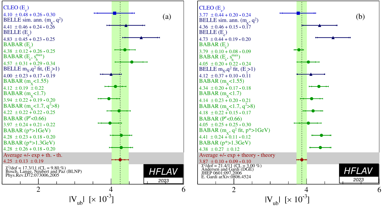
FIG. 24. Measurements of |V_{ub}| from inclusive semileptonic decays and their average based on the BLNP (a) and DGE (b) prescription. The labels indicate the variables and selections used to define the signal regions in the different analyses.
