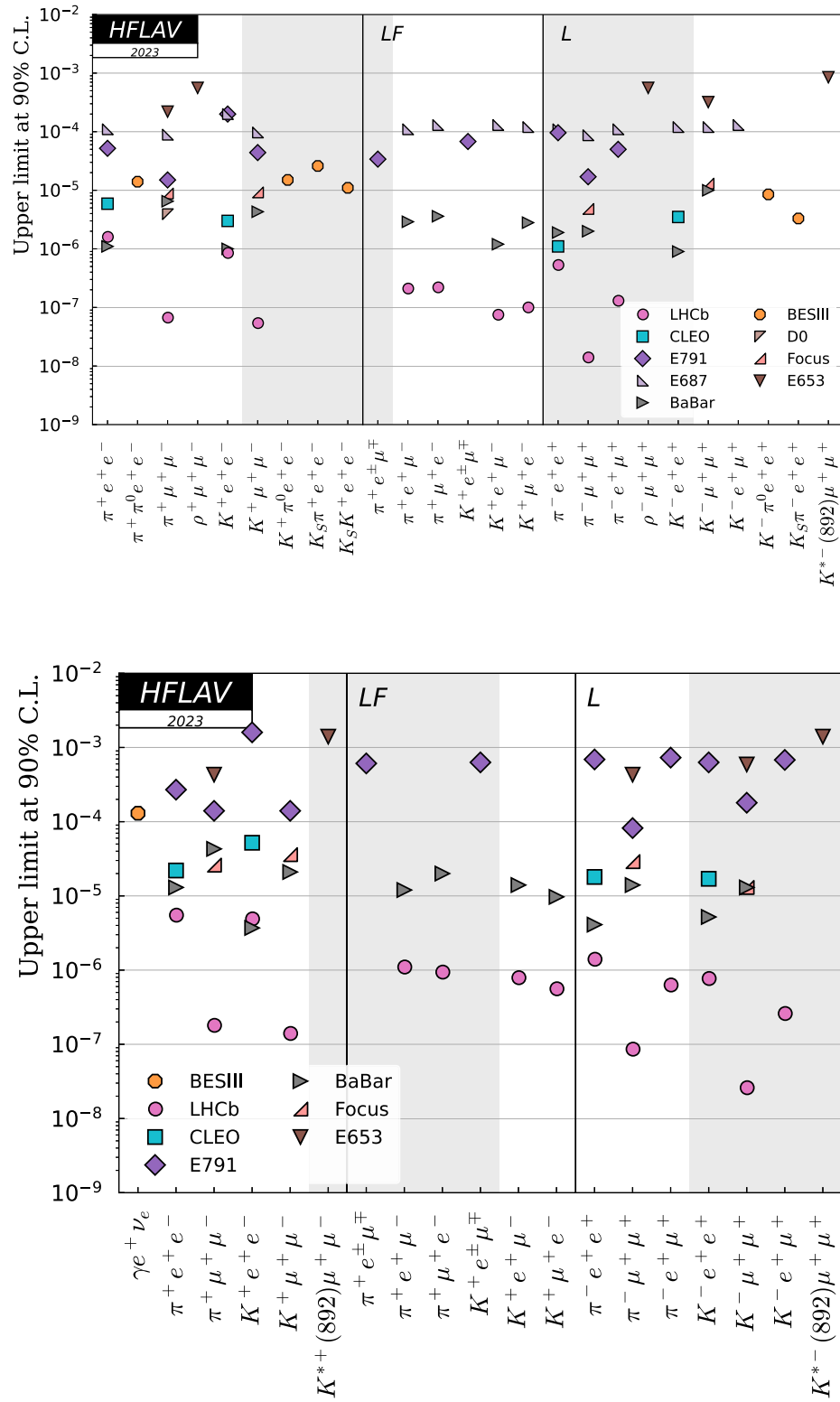
FIG. 61. Upper limits at 90% CL for D^+ (top) and D_s^+ (bottom) decay branching fractions. Each plot shows flavor-changing neutral current and rare decays, lepton-flavor-changing decays (LF), and lepton-number-changing (L) decays.
