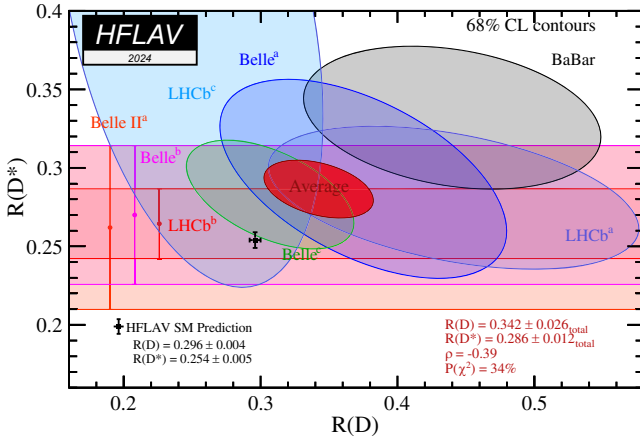
FIG. 27. Measurements of \mathcal{R}(D) and \mathcal{R}(D^*) listed in Table 53 and their two-dimensional average. The measurements from the same experiment are identified by the unique superscript characters as defined in the text and in Table. 53. Contours correspond to 68% CL (i.e. \Delta\chi^2 = 2.3 ). The black point with error bars, is the arithmetic average of the SM prediction for \mathcal{R}(D^*) and \mathcal{R}(D) reported in Table 52. More information is given in the text. An average of these predictions and the experimental average deviate from each other by about 3.14\sigma .
