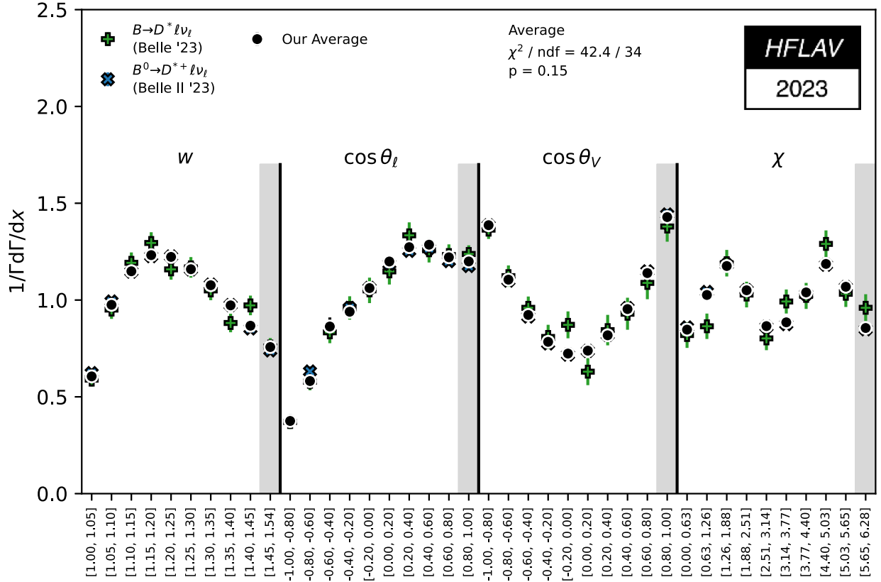
FIG. 12. The averaged normalized \bar{B} \rightarrow D^* \ell^- \bar{\nu}_\ell spectrum (black data points) together with the individual measurements by Belle [280] and Belle II [276] collaborations. The gray bands indicate the omitted data point in the average (see text).
