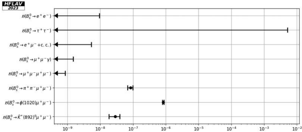
FIG. 33. Branching fractions of charmless leptonic B_s^0 decays.
