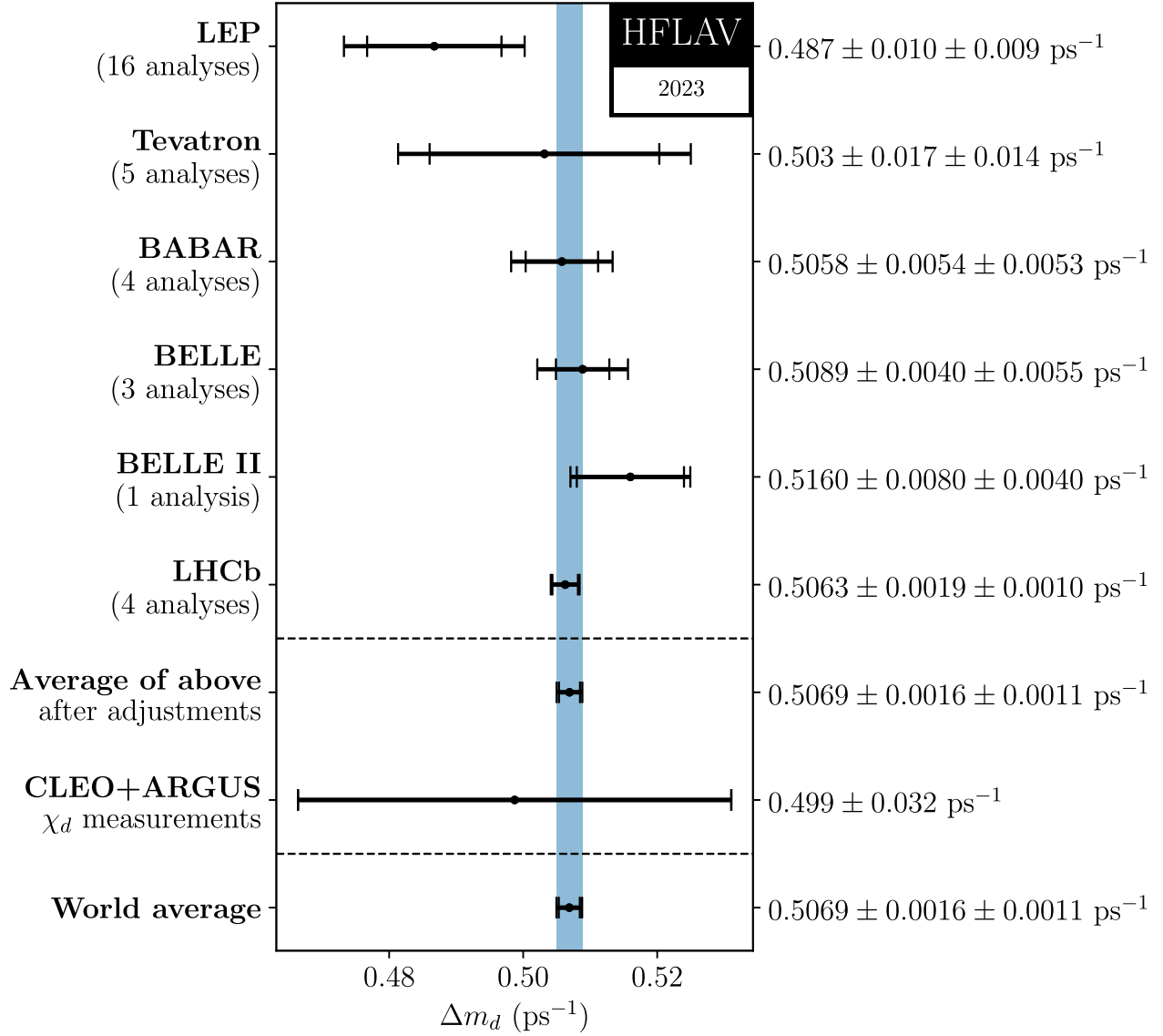
FIG. 5. The B^0 - \bar{B}^0 oscillation frequency \Delta m_d as measured by the different experiments. The LEP, Tevatron, BABAR , Belle, Belle II and LHCb averages are computed from the individual results listed in Table 14 without performing any adjustments. The time-integrated measurements of \chi_d from the symmetric B factory experiments ARGUS and CLEO are converted to a \Delta m_d value using \tau(B^0) = 1.517 \pm 0.004 ps. The two global averages are obtained after adjustments of all the individual \Delta m_d results of Table 14 (see text).
