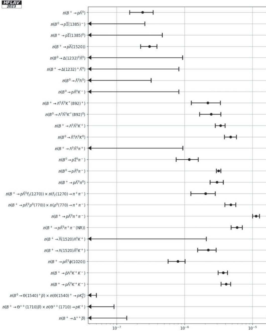
FIG. 31. Branching fractions of charmless B^+ and B^0 decays into strange baryons.
