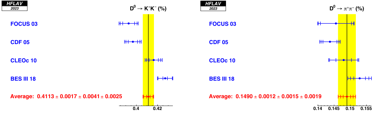
FIG. 57. The \mathcal{B}(D^0 \rightarrow K^+ K^-) (left) and \mathcal{B}(D^0 \rightarrow \pi^+ \pi^-) (right) values obtained either from absolute measurements or by scaling the measured branching ratios with the \mathcal{B}(D^0 \rightarrow K^- \pi^+) branching fraction average obtained here. For the measurements (blue points), the error bars correspond to the statistical, systematic and either the K\pi normalization uncertainties or, in case of an absolute measurement, the FSR modeling uncertainty. The average obtained here (red point, yellow band) lists the statistical, systematics excluding FSR, and the FSR systematic. For the measurements related to \mathcal{B}(D^0 \rightarrow K^+ K^-) [ \mathcal{B}(D^0 \rightarrow \pi^+ \pi^-) ] only, the partial \chi^2 is 15.7 [6.0] in the final fit.
