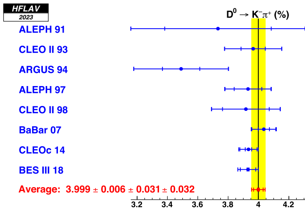
FIG. 56. Comparison of measurements of \mathcal{B}(D^0 \rightarrow K^- \pi^+) (blue) with the average branching fraction obtained here (red and yellow band). For these measurements only, the partial \chi^2 is 4.9 in the final fit.
