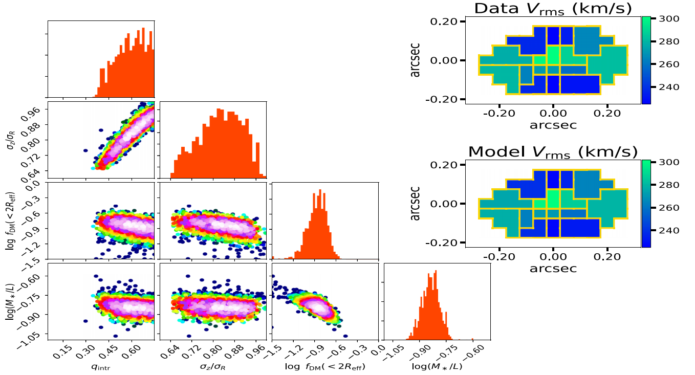
Figure F3. Fiducial recovery test for \log(M_*/L) . The tested input value is \log(M_*/L)_{\text{test},\text{in}} = -0.85 and the test output is \log(M_*/L)_{\text{test},\text{out}} = -0.86 \pm 0.04 . We have (\sigma_z/\sigma_R)_{\text{test},\text{out}} = 0.89 \pm 0.09 (in agreement with the input value of 0.85), q_{\text{test},\text{out}} = 0.66 \pm 0.11 (in agreement with the input value of 0.62), and (\log f_{\text{DM}, < 2R_{\text{eff}}})_{\text{test},\text{out}} = -0.85 \pm 0.14 (in agreement with the input value of -0.84 ). In this plot, we denote \log(M_*/L) \equiv \log[(M_*/L) / (M_\odot/L_\odot)] .
