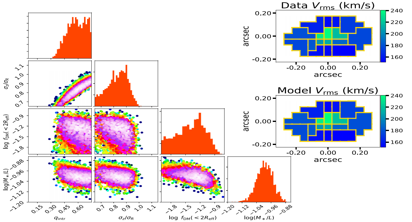
Figure F4. First fiducial model recovery test for \log f_{\text{DM}, < 2R_{\text{eff}}} . The tested input value is (\log f_{\text{DM}, < 2R_{\text{eff}}})_{\text{test},\text{in}} = -1.25 and the test output is (\log f_{\text{DM}, < 2R_{\text{eff}}})_{\text{test},\text{out}} = -1.22 \pm 0.32 . We have (\sigma_z/\sigma_R)_{\text{test},\text{out}} = 0.835 \pm 0.084 (in agreement with the input value of 0.85), q_{\text{test},\text{out}} = 0.59 \pm 0.11 (in agreement with the input value of 0.62), and \log(M_*/L)_{\text{test},\text{out}} = -1.008 \pm 0.044 (in agreement with the input value of -1.01 ). In this plot, we denote \log(M_*/L) \equiv \log[(M_*/L) / (M_\odot/L_\odot)] .
