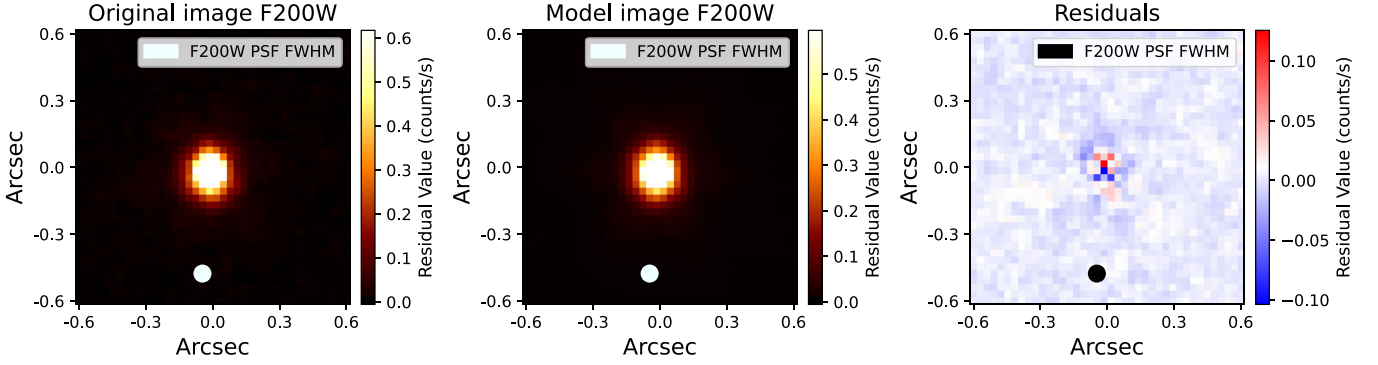
Figure 3. The original image in the NIRCam F200W band (a 40 \times 40 pixels zoom-in around the brightest pixel; the NIRCam photometry pixel scale is 0.03 arcsec per pixel) is shown in the left panel. Results of the PySERSIC fitting procedure of the original image are displayed in the middle panel. The panel on the right-hand side illustrates the residuals from the fit i.e. \text{res} = \text{original} - \text{model} . On each of these images, we display the FWHM size (0.065 arcsec) of the PSF of the NIRCam instrument in the F200W band.
