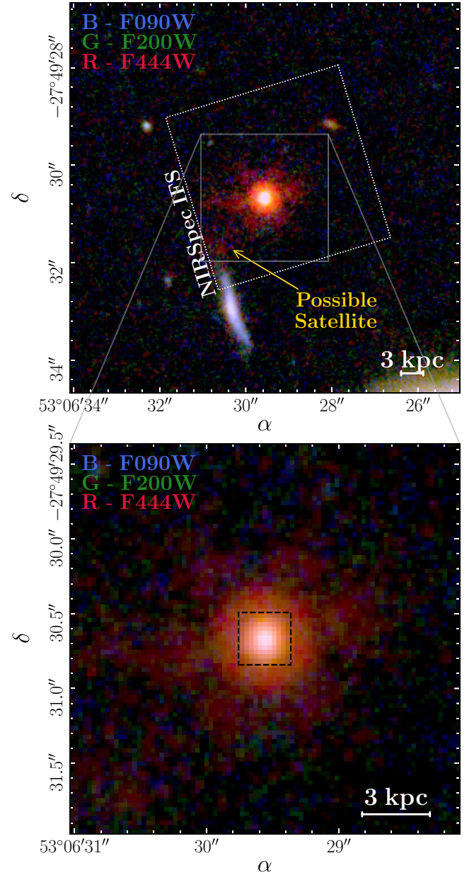
Figure 1. Top panel: composite image of GS-9209 obtained by the superposition of F090W, F200W, and F444W NIRCам photometry images. The dotted line is the effective FoV of our NIRSpec observations. A possible satellite is indicated. Bottom panel: zoomed-in portion of the same image, where we highlight the 0.35 \text{ arcsec} \times 0.35 \text{ arcsec} aperture used for measuring the integrated stellar velocity dispersion \sigma_* .
