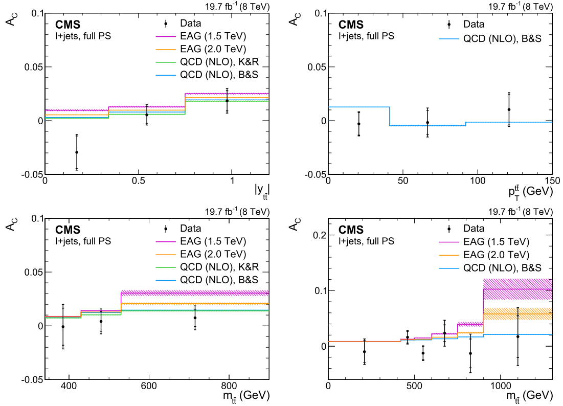
Fig. 5. Corrected asymmetry as a function of |y_{t\bar{t}}| (upper left), p_{T}^{t\bar{t}} (upper right), and m_{t\bar{t}} (lower left and lower right). The latter is shown in two different binnings. All results correspond to the full phase space . The measured values are compared to NLO predictions for the SM based on calculations by Kühn and Rodrigo (K&R) [10] and Bernreuther and Si (B&S) [11,49], as well as to the predictions of a model featuring an effective axial-vector coupling of the gluon (EAG) [52,53]. The inner bars indicate the statistical uncertainties, while the outer bars represent the statistical and systematic uncertainties added in quadrature.
