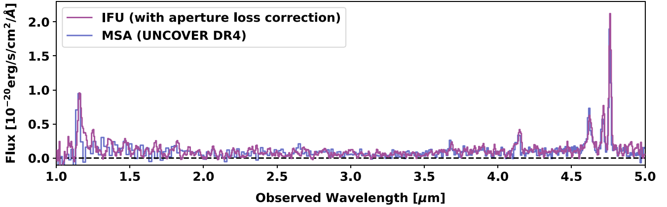
Figure A1. UNCOVER_20466 spectra from this work (pink) compared to NIRSpc MSA observations (S. H. Price et al. 2025, blue). All data have been corrected for gravitational magnification and slit or aperture loss.
