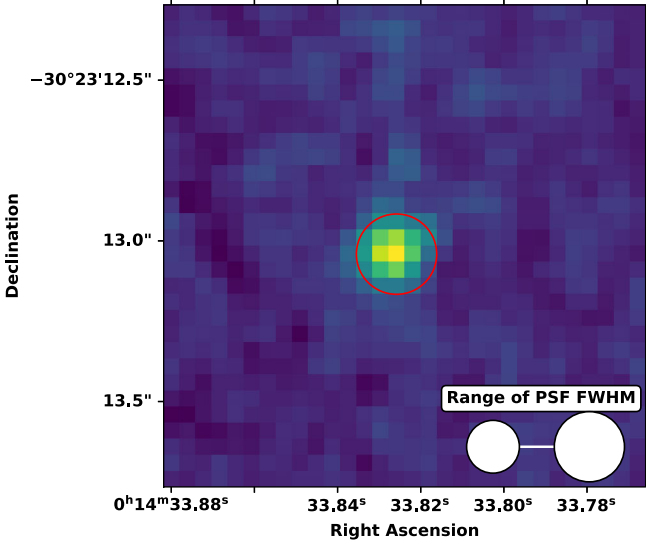
Figure 1. Flux map of [O III] \lambda 5007 in UNCOVER_20466, compared to adopted aperture (red circle) and PSF FWHM range of our data (white circles).
