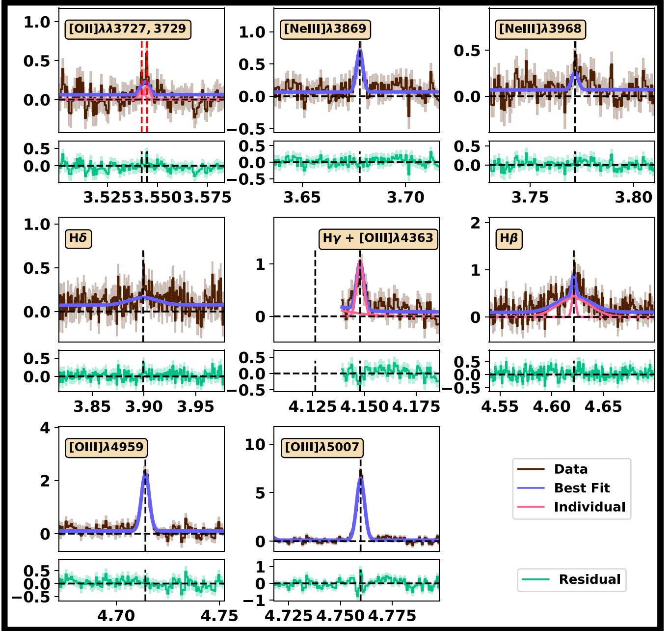
Figure 3. Spectrum extracted from NIRSpec IFU R2700 data cube (brown line) using a circular aperture of radius 0.125 arcsec. The best-fitting model (which was fit to the R100 and R2700 data simultaneously) is shown as blue lines. When two components or lines are overlapping, they are shown by pink lines. Model residuals are shown in the lower portion of each panel (green lines). The best-fitting centroid wavelengths of the narrow components of each line are shown by dashed vertical lines. We only show the wavelength range around emission lines of interest. Uncertainties ( 1\sigma ) for the extracted spectrum and residuals are shown by shaded regions.
