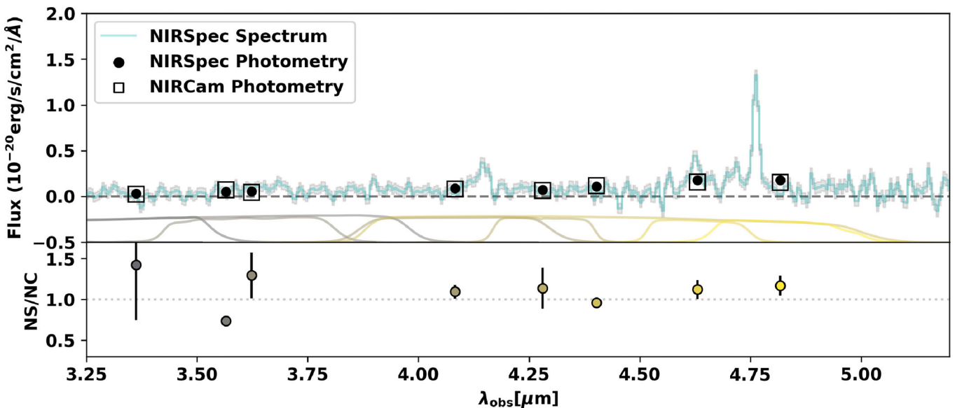
Figure D4. Comparison of the JWST /NIRSpec R100 spectrum and pseudo-photometry with JWST /NIRCам photometry (top panel). The pseudo-photometry was created using the throughput curves for each NIRCам filter, shown in the lower portion of the top panel. This results in ratio of NIRSpec to NIRCам photometric fluxes that are in broad agreement with the expected value from the empirical NIRSpec PSF (lower panel).
