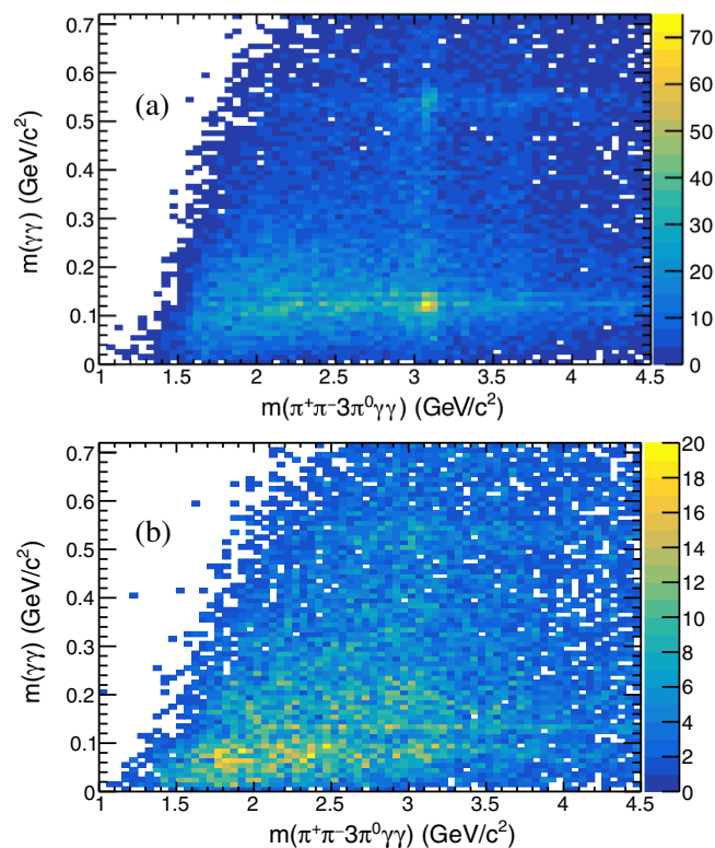
FIG. 2. (a) The fourth-photon-pair invariant mass m(\gamma\gamma) vs m(2\pi^3\pi^0\gamma\gamma) for (a) \chi^2_{2\pi^3\pi^0\gamma\gamma} < 70 and (b) 70 < \chi^2_{2\pi^3\pi^0\gamma\gamma} < 140 .
