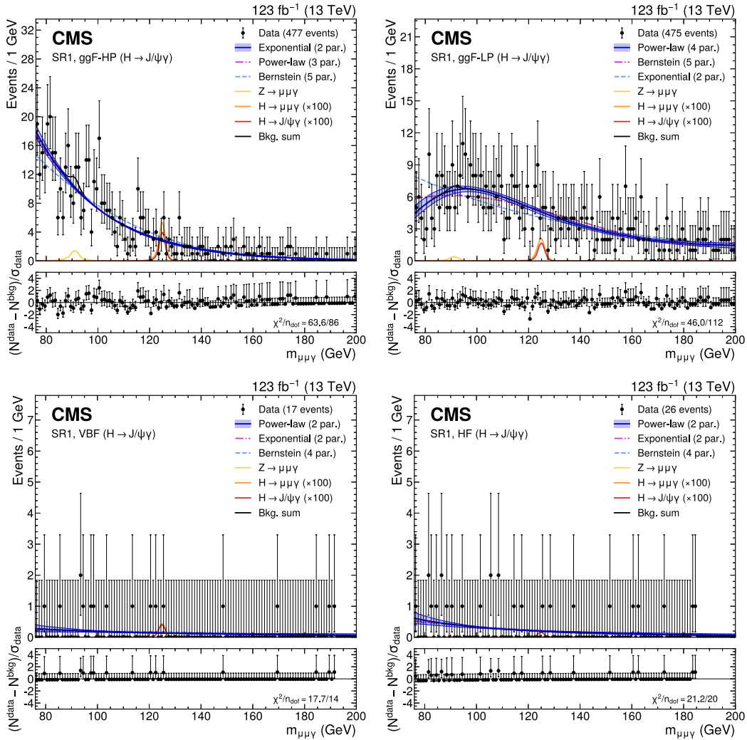
Fig. 2. The upper panels show the background-only fit using the power-law, exponential, and Bernstein polynomial functions with the optimal number of parameters determined with the F-test, and ranked according to the fit \chi^2 . The resonant background contributions are added with the normalization fixed to the SM expectation. The vertical error bars on the data points show the statistical uncertainty. The bottom panels show the pulls for the fit result for the model with lowest \chi^2 . Upper left: H \rightarrow J/\psi\gamma ggF-HP category. Upper right: H \rightarrow J/\psi\gamma ggF-LP category. Lower left: H \rightarrow J/\psi\gamma VBF category. Lower right: H \rightarrow J/\psi\gamma HF category.
