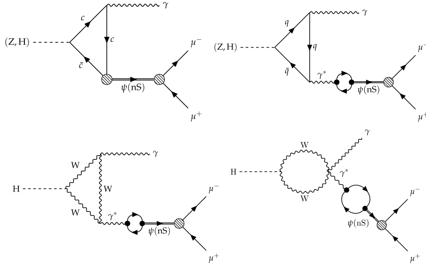
Fig. 1. Leading-order Feynman diagrams of Z and Higgs boson rare decays to J/\psi or \psi(2S) , and a photon, through the direct (upper top) and indirect (upper bottom, lower top, and lower bottom) processes. These four diagrams are considered as the signal of this analysis.
