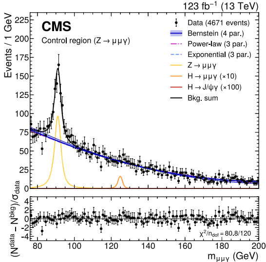
Fig. 4. The upper panel shows the results of the main background fit in the CR, using the power-law, exponential, and Bernstein polynomial functions with the optimal number of parameters determined with the F-test, and ranked according to the fit \chi^2 . The vertical error bars on the data points show the statistical uncertainty. The bottom panel shows the pulls for the fit result for the model with lowest \chi^2 .
