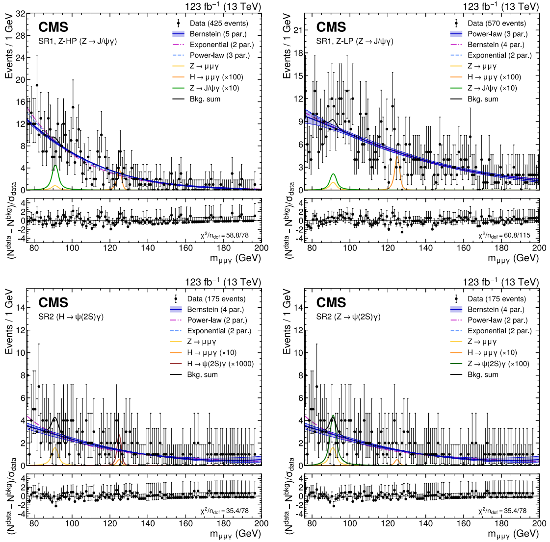
Fig. 3. The upper panels show the background-only fit using the power-law, exponential, and Bernstein polynomial functions with the optimal number of parameters determined with the F-test, and ranked according to the fit \chi^2 . The resonant background contributions are added with the normalization fixed to the SM expectation. The vertical error bars on the data points show the statistical uncertainty. The bottom panels show the pulls for the fit result for the model with lowest \chi^2 . Upper left: Z \rightarrow J/\psi\gamma HP category. Upper right: Z \rightarrow J/\psi\gamma LP category. Lower left: H \rightarrow \psi(2S)\gamma category. Lower right: Z \rightarrow \psi(2S)\gamma category.
