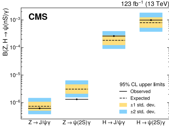
Fig. 5. Observed and expected (with \pm 1 , \pm 2 standard deviation bands) exclusion limits on the branching fraction of the (H, Z) \rightarrow \psi(nS)\gamma decays.
