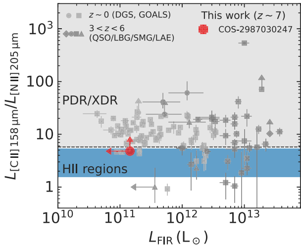
Figure 5. Luminosity ratio of [C II] 158 over [N II] 205 \mu\text{m} as a function of the FIR luminosity. Local galaxies shown are from GOALS (Díaz-Santos et al. 2017) and DGS (Cormier et al. 2015, 2019); constraints on high-redshift galaxies (Decarli et al. 2014; Pavese et al. 2016, 2019) and SMGs as part of the SPT survey (Cunningham et al. 2020) are included as well (see Section 5.1 for details). LBGs are indicated with circles, SMGs with squares, LAEs with upward facing triangles, and the quasar (QSO) as a diamond. The luminosity ratio expected for [C II] emission originating in H II regions for typical physical conditions (solar metallicity and \log_{10} U < -3 , n_{\text{H}} < 10^2 \text{ cm}^{-3} ; see Section 5.1) is shown as the blue shaded area. A dashed line demarcates L_{[\text{C II}]} / L_{[\text{N II}]} \simeq 6 , the minimum value found across a large range of PDR models (grey shaded area; a similar neutral medium can be created in the presence of X-ray-dominated region (XDRs) or shocked gas, see e.g. Decarli et al. 2014). For COS-2987030247, the 3\sigma upper limit on [N II] is fully consistent with [C II] production in a PDR-like medium.
