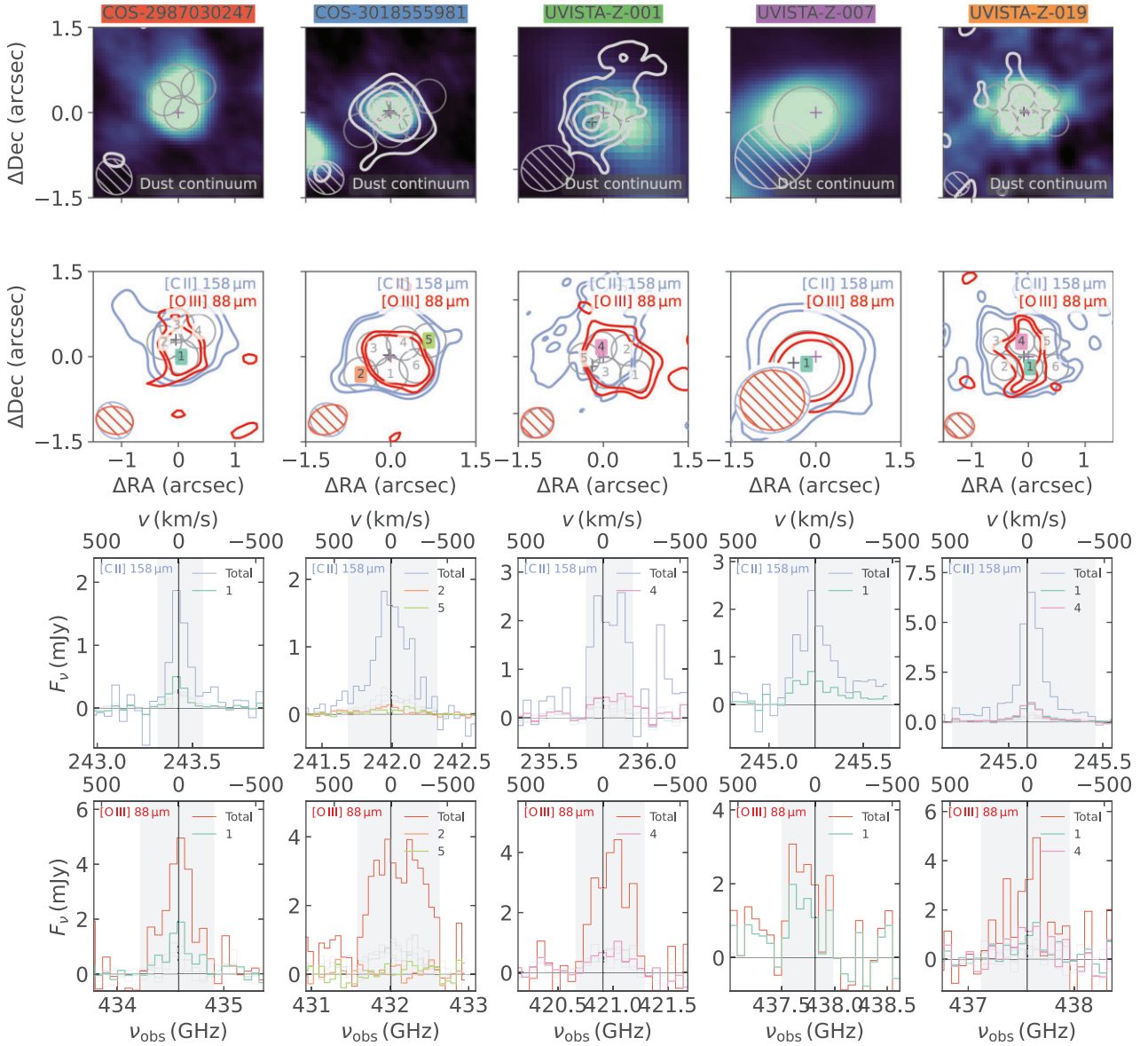
Figure A1. Beam placement for spatially resolved analysis. The top row of images shows the UV continuum with contours of the \sim 160\text{-}\mu\text{m} dust continuum (starting from 2\sigma and going up in steps of 1\sigma for COS-2987030247 and UVISTA-Z-019, else 2\sigma ). The peaks of the UV and dust continua (if detected) are indicated with a black and purple cross, respectively. Contours (at 2\sigma and 3\sigma ) of the [C II] 158- and [O III] 88- \mu\text{m} lines are shown in the second row (and again the UV and dust peaks). The last two rows contain their spectra, both integrated over the entire 2\sigma region (in the same colour as their contours) as well as for the individual regions. For each source, one or several regions are highlighted in the spectra and correspondingly by their number in the second row of images. The filled-in grey region indicates the spectral channels over which the spectra have been integrated.
