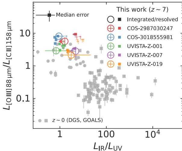
Figure 10. Sequence of the [O III] 88- to [C II] 158- \mu\text{m} ratio as a function of L_{\text{IR}}/L_{\text{UV}} . Global measurements of the DGS and GOALS samples are shown, as are the five z \sim 7 star-forming galaxies discussed in this work. Furthermore, spatially resolved ratios extracted from individual regions across all five sources (see Appendix B for details) are shown as squares (smaller squares if we can only set 2\sigma limits on both ratios). For clarity, error bars of the spatially resolved measurements are not shown; the median error of these points is indicated by the black square in the top left-hand panel.
