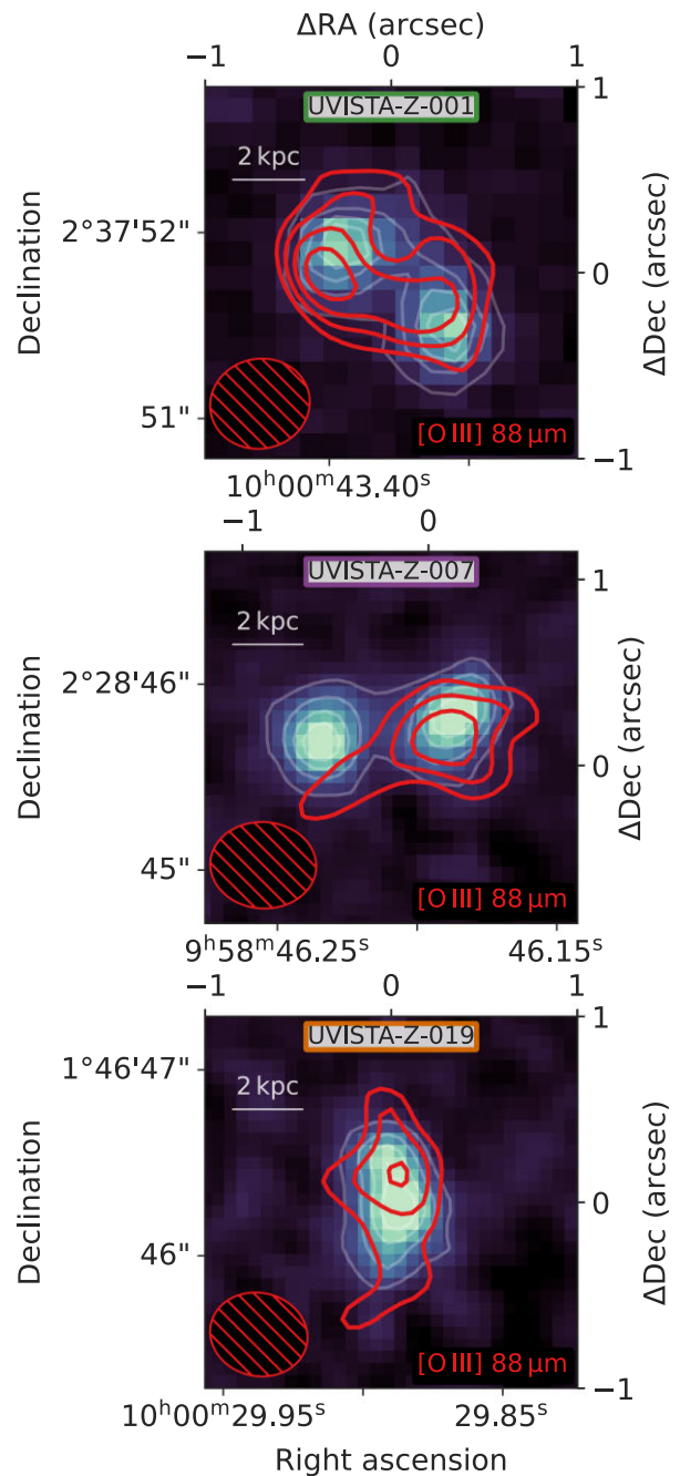
Figure 8. HST images of the rest-frame UV (in the JH_{140} band; Section 2.3) overlaid by contours of the [O III] 88- \mu m line (achieving an \sim 0.4 -arcsec resolution with natural weighting; see Table 2) of UVISTA-Z-001 (top panel), UVISTA-Z-007 (middle panel), and UVISTA-Z-019 (bottom panel). Red [O III] contours are drawn from 3\sigma and going up in steps of 1\sigma . The top left-hand panel indicates a physical scale of 2 kpc. Beam sizes for [O III] are indicated in the bottom left-hand panel.
