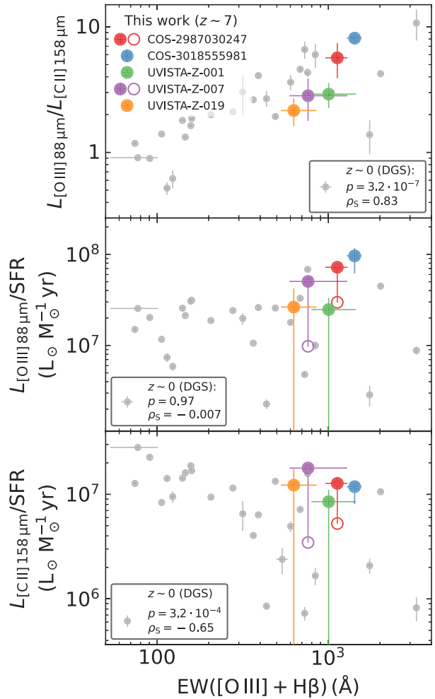
Figure 6. Ratios of the [O III] 88- and [C II] 158- \mu\text{m} luminosities with respect to each other (top panel) and with respect to the SFR (middle panel for [O III], bottom panel for [C II]) as a function of the EW of the optical [O III] and H\beta lines. If the measured SFR is an upper limit (due to a non-detection of the dust continuum), unobscured SFR measurements are shown with an open circle. Small grey circles are galaxies from DGS (see Section 5.2). The p -value, for a null hypothesis that the data are uncorrelated, and Spearman’s rank correlation coefficient ( \rho_s ) of these points measured in logarithmic space are indicated in each panel. Coloured circles show the five z \sim 7 galaxies considered in this work. There is a significant positive correlation between the [O III]/[C II] ratio and their optical EW among the DGS galaxies, which seems to derive mostly from a negative correlation between [C II]/SFR and the EW; however, the correlation of the [O III]/[C II] luminosity ratio is stronger than that of the (relative) [C II] luminosity on its own. Furthermore, it is unclear whether the same is true for the small sample of high-redshift galaxies.
