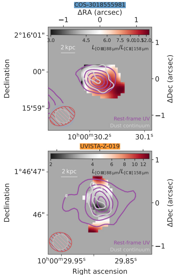
Figure 9. Line ratio maps of the [O III] 88- and [C II] 158- \mu\text{m} lines for COS-3018555981 (top panel) and UVISTA-Z-019 (bottom panel), where imaging parameters have been chosen to match beam sizes (see Table 2). Light grey contours are drawn for the dust continuum (at \sim 160 \mu\text{m} , with natural weighting scheme; Section 5.6 for details), starting from 3\sigma and going up in steps of 2\sigma . Purple contours are drawn for the HST imaging (Section 2.3) of the rest-frame UV (convolved to match the dust-continuum PSF), starting from 5\sigma and going up in steps of 5\sigma . Beam sizes are indicated in the bottom left (partially hiding a foreground source in the HST imaging of COS-3018555981); the top left-hand panel indicates a physical scale of 2 kpc. There is tentative evidence for spatial variation in the [O III]/[C II] ratio, including a gradient with the lowest [O III]/[C II] values seeming to align with the location of the dust emission in COS-3018555981.
