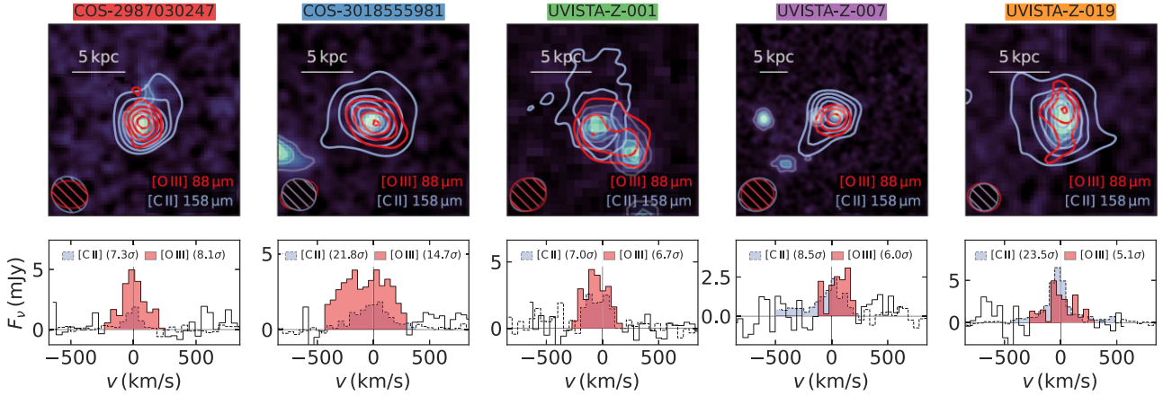
Figure 2. Detections of the [C II] 158- and [O III] 88- \mu\text{m} lines. Top row: contour images of the [C II] and [O III] lines overlaid on a background of HST rest-frame UV images (see Section 2.3). The line images have matched beam sizes (as listed in Table 2) and are produced by collapsing all channels within the FWHM of the line (as those of the S/N determination, which however use natural weighting without tapering; Section 3.3). Contours start at 3\sigma and increase in steps of 5\sigma for the [C II] contours in COS-3018555981 and UVISTA-Z-019, 3\sigma for the [O III] contours in COS-3018555981, 2\sigma for both lines in UVISTA-Z-001, and 1\sigma otherwise. Bottom row: S/N-weighted line spectra extracted from a 2\sigma region in a naturally weighted image integrated over the FWHM (cf. Section 3.3). Coloured channels, which were used to produce a subsequent moment-zero map for measuring the total line flux, indicate the line detection. The significance of each line detection is shown in the legend (also see Section 3.3 for details).
