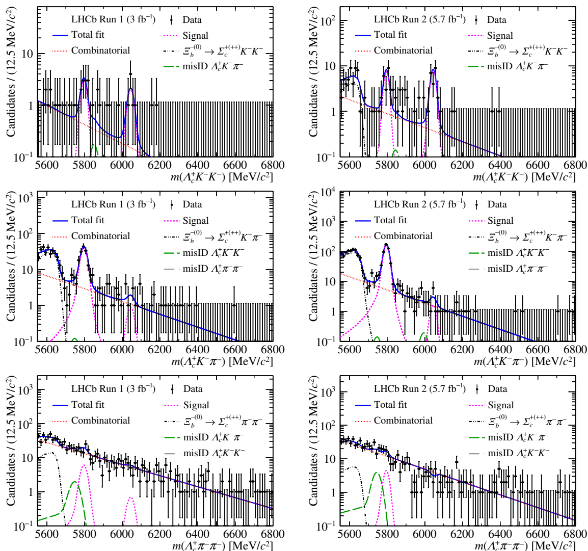
Figure 3. Mass distributions of the signal channels with results of the fit superimposed: (top) A_c^+ K^- K^- , (middle) A_c^+ K^- \pi^- and (bottom) A_c^+ \pi^- \pi^- final states for (left) Run 1 and (right) Run 2 (log scale). The different components in the fit are shown as indicated in the legends, where the signal components include independent contributions from \Xi_b^- and \Omega_b^- decays.
