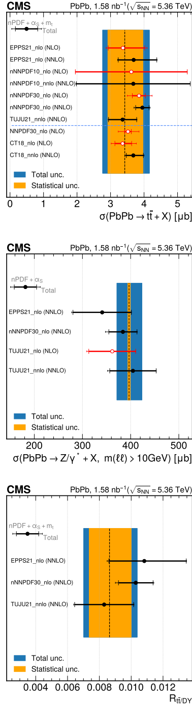
Figure 9. Experimental measurements (colored bands) of the t\bar{t} cross section (upper), DY cross section (middle), and R_{t\bar{t}/DY} ratio (lower) in inclusive PbPb collisions at \sqrt{s_{NN}} = 5.36 TeV compared with the corresponding NLO (red bars) or NNLO + NNLL (black bars) theoretical predictions obtained with the EPPS21_nlo, nNNPDF10_(n)lo, nNNPDF30_nlo, and TUJU21_(n)lo nPDF sets. The error bars represent the theoretical uncertainties, and the blue (orange) area shows the total (statistical) uncertainties of the measurements. In the upper plot a dashed line separates the theory predictions obtained with nuclear PDFs (above the line) from those with the proton PDFs (below the line).
