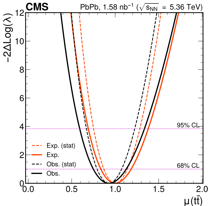
Figure 7. Scan of the profile likelihood as a function of the t\bar{t} signal strength. The expected (orange) and observed (black) scans are displayed with (solid curve) and without (dashed curve) accounting for systematic uncertainties. The horizontal dashed lines indicate the likelihood values used to extract the 68% and 95% CL intervals on the parameter of interest.
