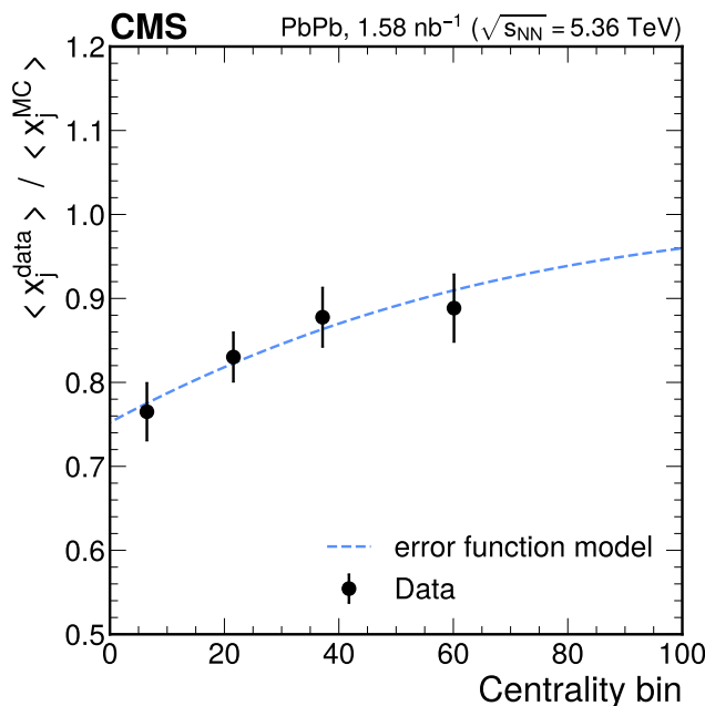
Figure 4. Ratio of the average \langle x_j \rangle detector-level distributions measured in data over simulation as a function of the collision centrality with a fit to an error function (blue dashed curve) superimposed.
