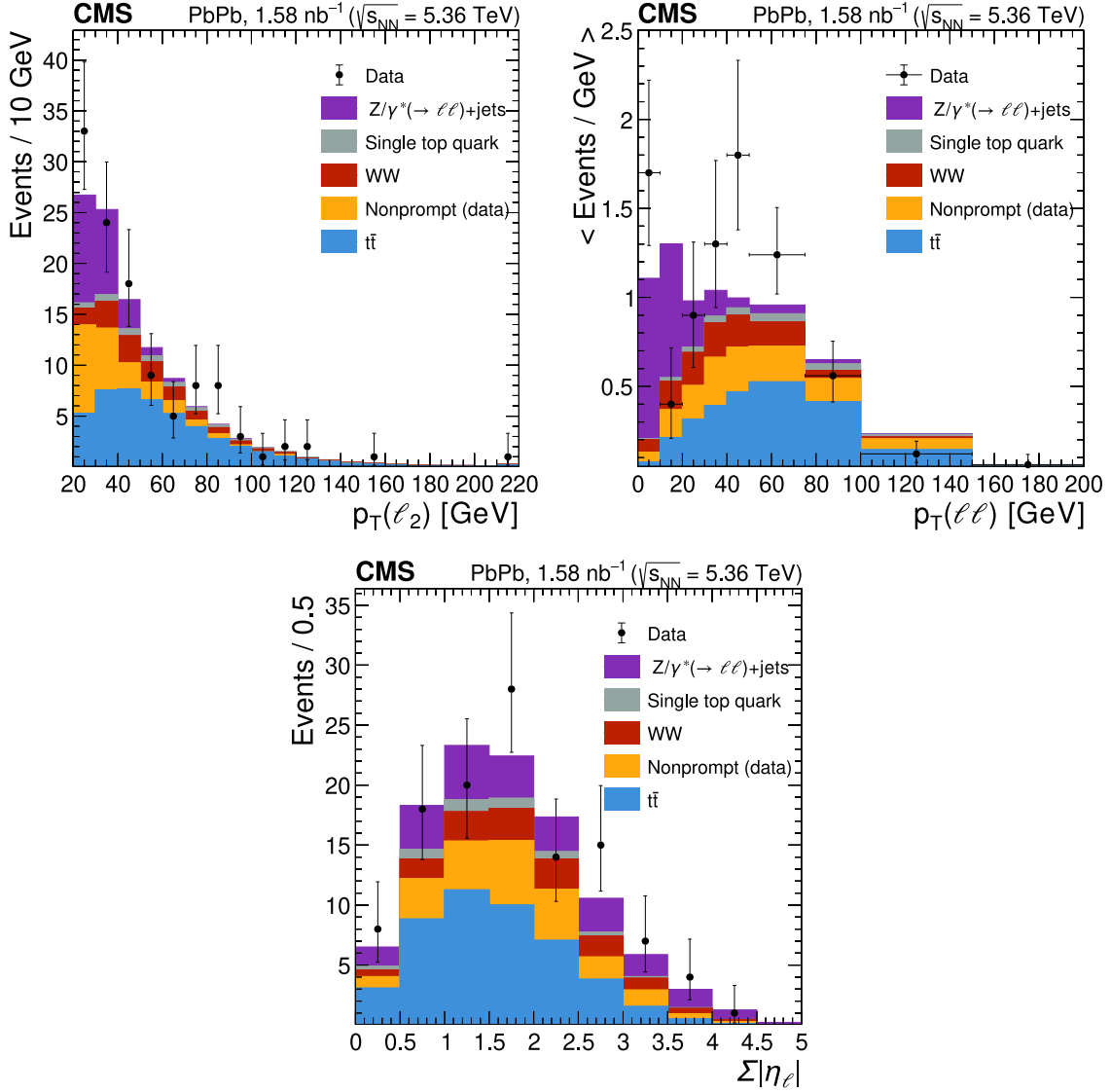
Figure 2. Distributions of p_T(\ell_2) (upper left), p_T(\ell\ell) (upper right), and \sum|\eta_\ell| (lower) variables in the different-flavor ( e^\mp\mu^\pm ) channel. The data (black markers with error bars representing statistical uncertainties) are overlaid on top of the stacked contributions from the expected t\bar{t} (blue), nonprompt (light orange), WW (red), single top quark (gray), and DY (violet) processes. The last bin includes the overflow entries.
