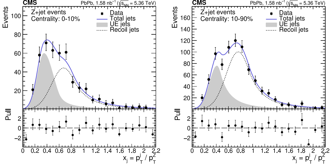
Figure 3. Distribution of the x_j = p_T(\text{jet})/p_T(Z) ratio in Z + jet events in the 0–10% (left) and 10–90% (right) PbPb centralities. The data (solid dots with error bars) are compared with the contributions from UE jets (gray histograms) and true recoil jets (black dashed curves) stacked. The blue curves show the sum of UE and recoil jet contributions.
