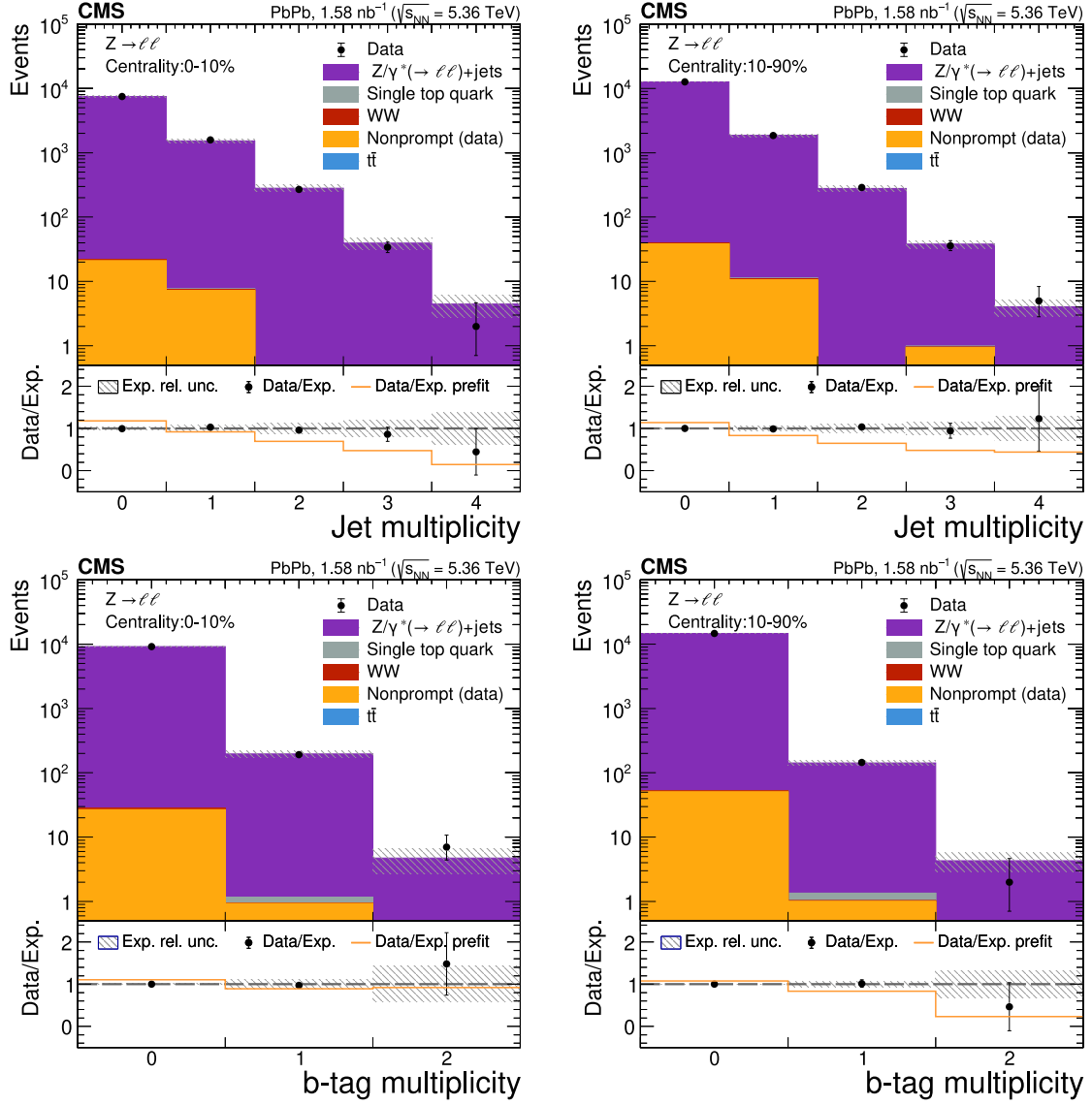
Figure 5. Multiplicities of inclusive (upper) and b-tagged (lower) jets in Z boson candidate events in the 0–10% (left) and 10–90% (right) centrality bins measured in the data (black markers) compared with the post-fit stacked model of the t\bar{t} (blue), nonprompt (light orange), WW (red), single top quark (gray), and DY (violet) contributions. The lower panels show the data-to-expectation ratios before (orange lines) and after (black markers) the fit. The hatched band represents the post-fit uncertainty of the model in each bin. The last bins include the overflow entries.
