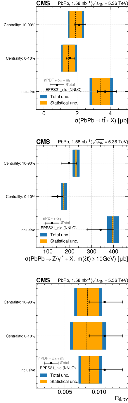
Figure 10. Experimental measurements (colored bands) of the t\bar{t} cross section (upper), DY cross section (middle), and R_{t\bar{t}/\text{DY}} ratio (lower) in semicentral (10–90%), central (0–10%), and inclusive PbPb collisions at \sqrt{s_{\text{NN}}} = 5.36 TeV compared with the corresponding NNLO + NNLL theoretical predictions (black markers with error bars) obtained with the EPPS21_nlo [23] nPDF set. The blue (orange) bands indicate the total (statistical) uncertainties of the measured observables, whereas the error bars represent the uncertainties in the theory calculations.
