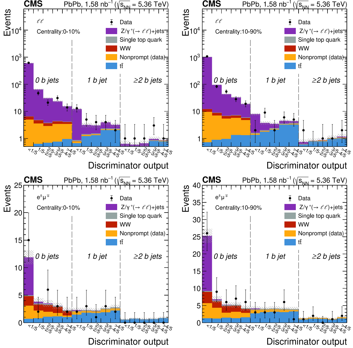
Figure 6. Distributions of the final BDT discriminator after the fit for the same-flavor \ell\ell (upper) and different-flavor e^+\mu^\pm (lower) channels. The discriminator output is shown for 0, 1, and \geq 2 b-tagged jet events. The left (right) figures correspond to events reconstructed in the 0–10% (10–90%) centrality bin. The data (black markers) are compared with the stacked histograms corresponding to the t\bar{t} signal (blue), and the nonprompt (light orange), WW (red), single top quark (gray), and DY (violet) background processes normalized to their post-fit expectations. The hatched gray bands show the total uncertainty in the predicted yields after the fit is performed.
