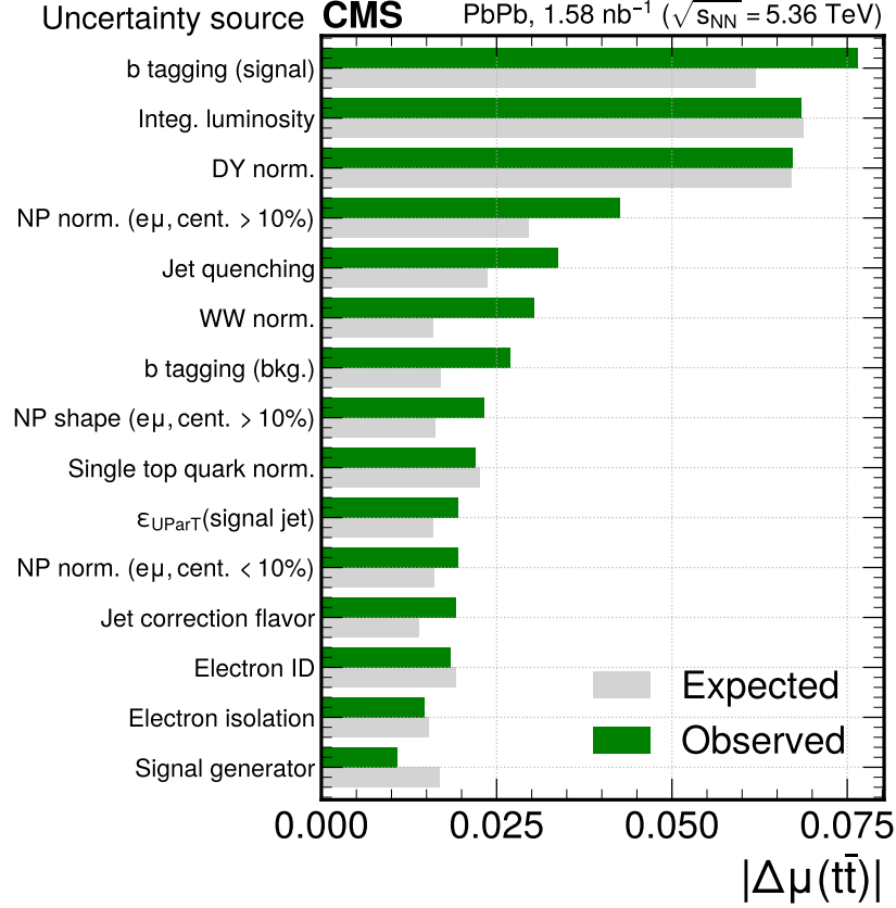
Figure 8. Impact of systematic uncertainties on the fitted t\bar{t} signal strength parameter. The systematic uncertainties are listed in decreasing order of their impact on the signal strength.
