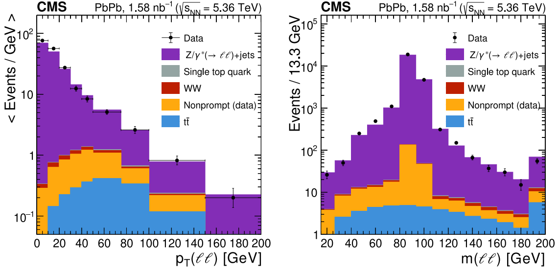
Figure 1. Distributions of dilepton p_T(\ell\ell) (left) and invariant mass m(\ell\ell) (right) variables in the same-flavor ( \ell\ell ) channels. The m(\ell\ell) distribution is shown before applying the veto of the Z boson resonant region. The data (black markers with error bars representing statistical uncertainties) are overlaid on top of the stacked contributions from the expected t\bar{t} (blue), nonprompt (light orange), WW (red), single top quark (gray), and DY (violet) processes. The last bin includes the overflow entries. In the left panel, the event counts are divided by the variable bin width.
