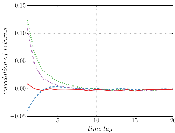
Fig. 7. The correlation function of returns for Microsoft, calculated with the proxy \hat{p}_t of the fundamental price defined in Eq. (23) (red solid), the alternative proxy \hat{p}'_t defined in Eq. (24) (violet dotted), the alternative proxy \hat{p}''_t defined in Eq. (25) (green dash-dotted), and the mid price x_t (blue dashed).
