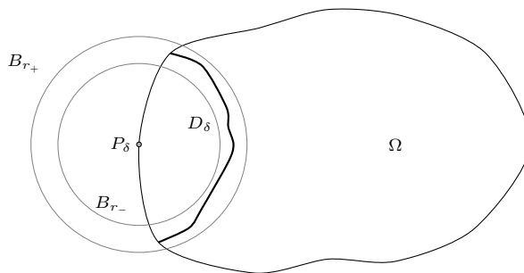
Fig. 1. The optimal set D_\delta , for \delta small, according to Theorem 1.1.
