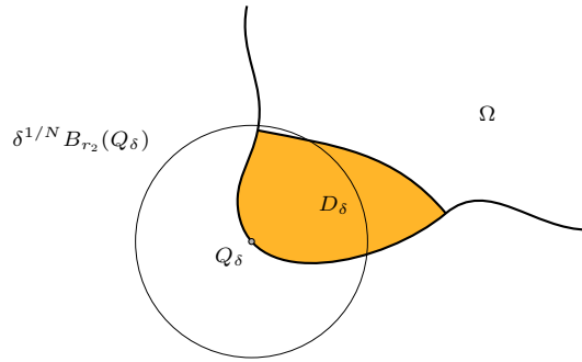
Fig. 2. The optimal set D_\delta , for \delta small, according to Theorems 1.2, 1.4.
