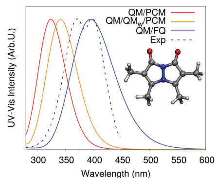
Fig. 6 Calculated QM/PCM, QM/QM w /PCM and QM/FQ UV-Vis spectra of bimeane in aqueous solution. The experimental spectrum, taken from ref. 39 is also reported. QM level: CAM-B3LYP/6-311+G**.
