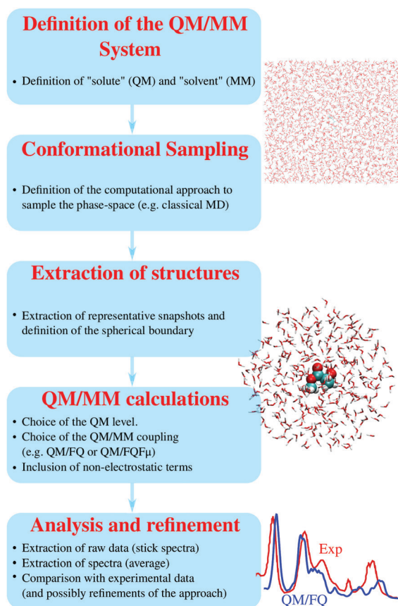
Fig. 3 Schematic view of the computational protocol.
