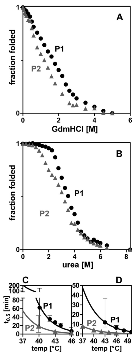
FIGURE 1. PAPS synthases differ in their protein stability. A and B, chemical unfolding of human PAPS synthases by guanidine hydrochloride ( GuaHCl ) and urea monitored by intrinsic tryptophan fluorescence. Irreversible unfolding proceeds via at least one intermediate. Midpoints of unfolding were at 1.70 and 1.19 M GdmHCl , as well as 3.50 and 3.11 M urea for PAPS synthases 1 and 2 (P1 and P2), respectively. C and D, loss-of-activity measurements of APS kinase and ATP sulfurylase domains, respectively. Proteins were incubated for increasing times at elevated temperatures. Subsequently, residual activity was measured under standard conditions. Error bars represent 95% confidence intervals.
