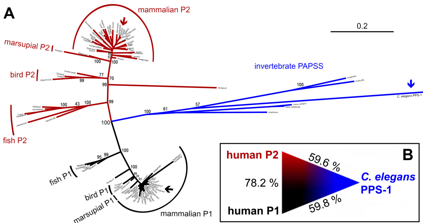
FIGURE 3. Relationship between the human PAPS synthases and their counterpart from C. elegans . A, un-rooted maximum likelihood phylogenetic tree of vertebrate and invertebrate sequences for bifunctional PAPS synthases. The three groups of proteins, PAPSS1-type (black), PAPSS2-type (red), and invertebrate PAPS synthases (blue) are clearly separated by a bootstrap of 100. PAPS synthases from man and worm are marked by arrows. B, amino acid identity between C. elegans PPS-1 and the two human PAPS synthase isoforms indicates that it is not possible to derive further phylogenetic relationships for these proteins.
