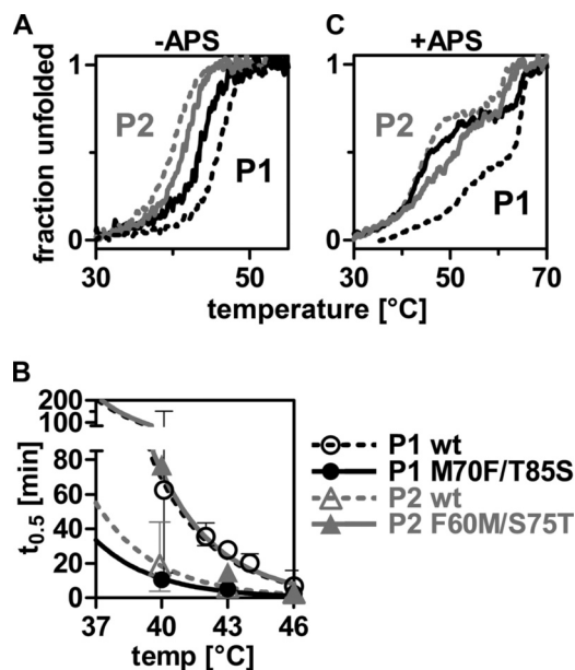
FIGURE 6. Characterization of the Met ⇌ Phe/Thr ⇌ Ser double mutants. A, thermal unfolding transitions monitored by CD spectroscopy at 225 nm. B, loss-of-activity measurement of the APS kinase activity of wild-type and mutant proteins. C, thermal unfolding transitions in presence of 50 \mu M APS. The legend applies to all three graphs.
