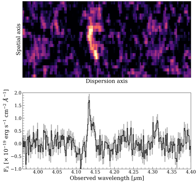
Fig. 3. Continuum-subtracted NIRCам F444W WFSS data of K20-ID7, zoomed-in over 3.95–4.40 \mu\text{m} , encompassing \text{Pa}\beta line emission. In the 2D slitless spectra (upper panel), the \text{Pa}\beta line emission is clearly spatially resolved perpendicular to the dispersion axis and extended along the parallel direction. This results in a double-peaked \text{Pa}\beta line profile in the total 1D spectrum (lower panel), a consequence of resolved spatial offsets combined with velocity gradients along the grism dispersion axis (discussed in Sect. 5).
