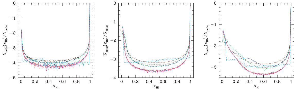
Figure 9. Test 1 (H II region expansion in a uniform gas at fixed temperature): fraction of cells with a given neutral fraction, x_{\text{HI}} = 1 - x at times t = 10 Myr (left-hand panel); 100 Myr (middle panel) and 500 Myr (right-hand panel).
