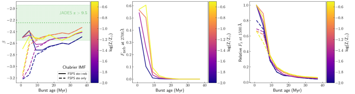
Figure 9. Left: \beta measured from synthetic spectra generated using FSPS with a Chabrier IMF as a function of age for a single burst of star formation with \log(U) = -2.0 . Solid lines show measurements from spectra containing both stellar and nebular emission, and dashed line containing only stellar emission. The colour bar represents metallicities in units of \log(Z_{*}/Z_{\odot}) . The dotted line is the median observed \beta for z > 9.5 galaxies in our sample, and the shaded region represents the 1\sigma dispersion. Middle: fraction of nebular continuum measured at 2700\text{ \AA} , which leads to an overall reddening of the measured UV slope, as a function of burst age, colour-coded by metallicity. We find that at low burst ages, nebular emission can contribute up to 60 per cent of the flux in the redder part of the wavelength range where \beta is measured, thereby reddening the measured \beta -values. Right: the relative F_{\lambda} measured at 1500\text{ \AA} from the model predictions, normalized at the maximum flux recorded in the stellar + nebular models at zero age. The nebular continuum for this particular IMF can provide a boost of up to 50 per cent to the UV luminosity at young ages. Overall, we find that redder \beta -values can also be achieved at burst ages > 30 Myr, but this is unlikely to be the case at z > 9.5 when galaxies are in the process of rapidly assembling their stellar masses through intense star formation.
