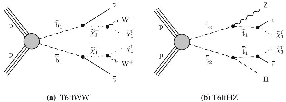
Fig. 2 Diagrams illustrating the simplified RPC SUSY models with squark production considered in this analysis
