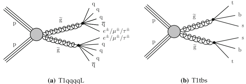
Fig. 3 Diagrams illustrating the two simplified RPV SUSY models considered in this analysis
