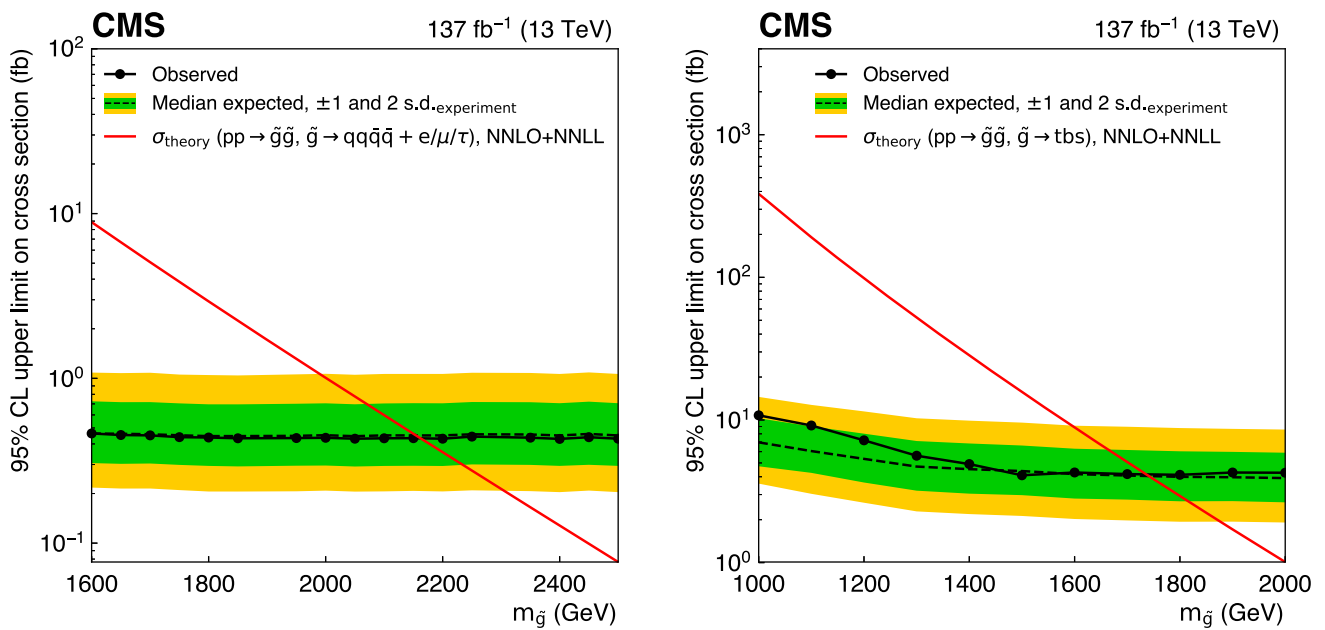
Fig. 12 Upper limits at 95% CL on the cross section for RPV gluino pair production with each gluino decaying into four quarks and one lepton (T1qqqL, left), and each gluino decaying into a top, bottom, and strange quarks (T1tbs, right)
