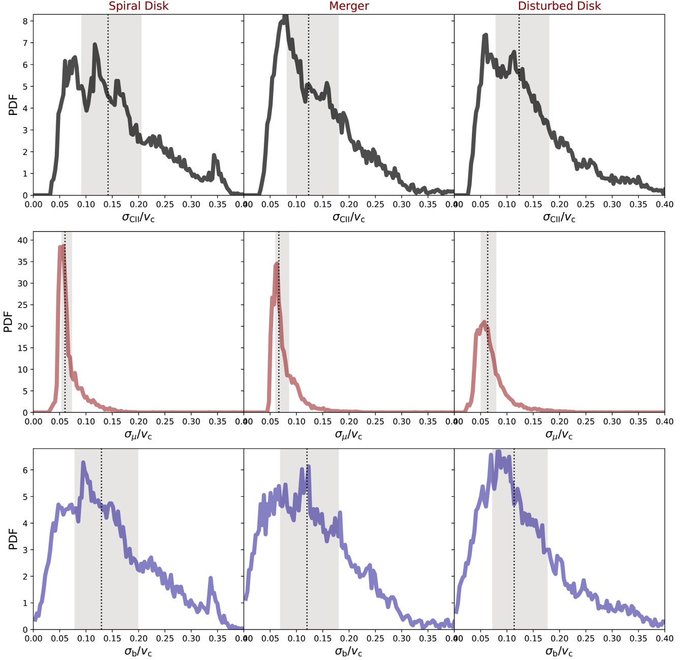
Figure 4. PDFs of the different velocity dispersion components for three evolutionary stages of Freesia. From top to bottom, we show the total velocity dispersion, \sigma_{[\text{C II}]} = (\sigma_{\mu}^2 + \sigma_b^2)^{1/2} , from Fig. 2; small-scale velocity dispersion, \sigma_{\mu} , due to stellar feedback from Fig. 5; the large-scale velocity dispersion, \sigma_b , due to bulk motions from Fig. 6. See Table 2 for a summary of the definitions. The vertical dotted line denotes the mean value; the grey-shaded area represents the width of the distribution which is the difference between 25th and 75th percentile of the distribution.
