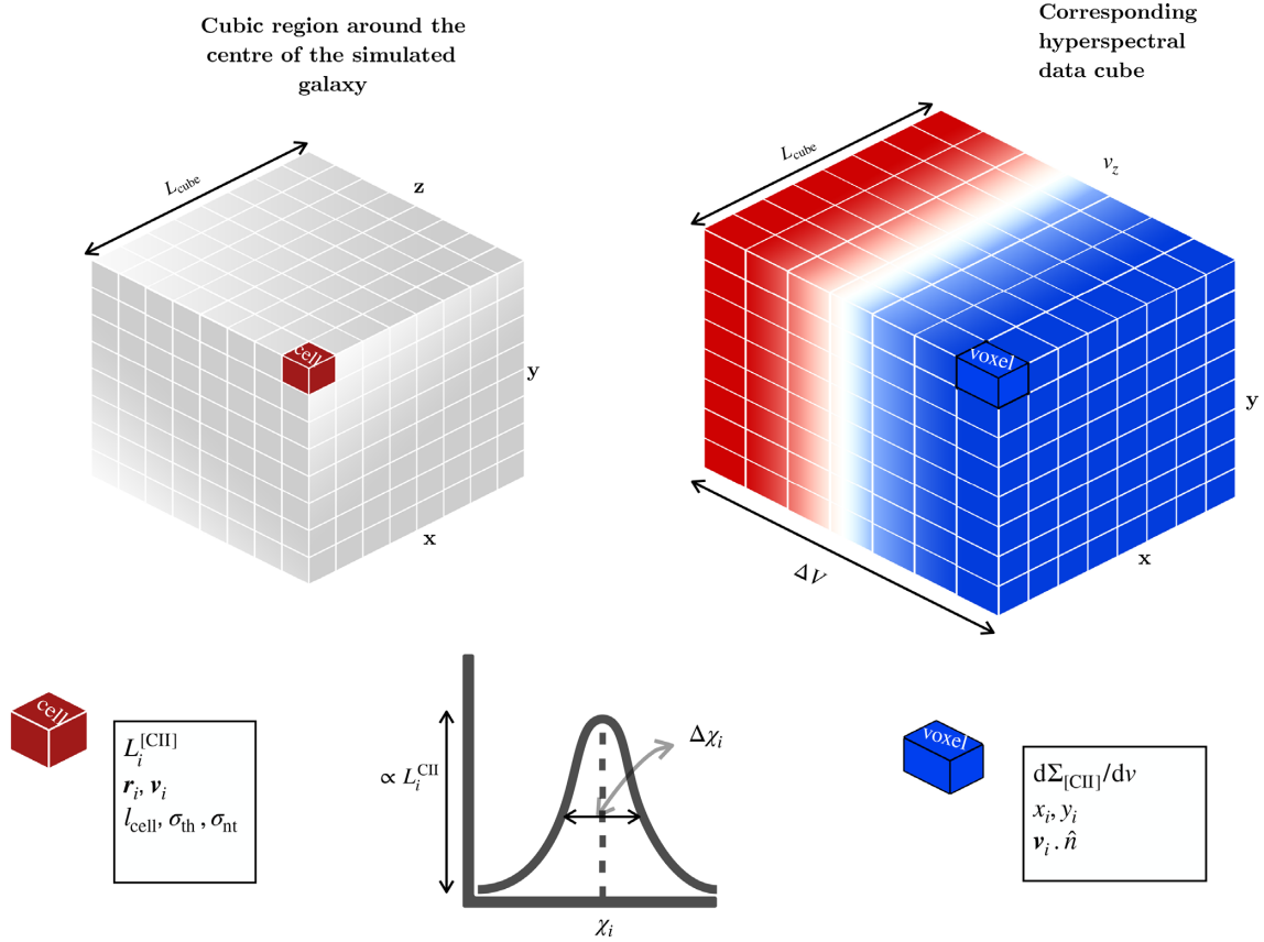
Figure 1. Sketch of the model used in this work to obtain hyperspectral data cubes from a simulation box. Having the information on the [C II] luminosity ( L_i^{[CII]} ), positions, and velocities of the gas particles along with the cell size ( l_{\text{cell}} ), thermal ( \sigma_{\text{th}} ), and non-thermal ( \sigma_{\text{nt}} ) line broadenings in a simulated cube, one can construct the hyperspectral data cubes with two spatial and one spectral dimensions. The mapping from the simulated box to the hyperspectral cube is done with three Gaussian filters in each dimension. The simulation box is represented as a uniformly binned space only for visualization purposes. See Section 3.2 for the details.
