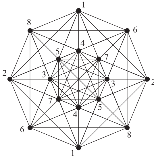
Figure 10. The chosen colouring for P^5 .
