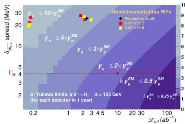
Fig. 137 Upper limit contours (at 95% CL) on the electron Yukawa y_e (coloured bands) in the collision-energy spread \delta\sqrt{s} vs. integrated luminosity \mathcal{L}_{\text{int}} plane. The red star over the \delta\sqrt{s} = \Gamma_H = 4.1 MeV red-dashed line indicates the reference point assumed in the physics simulation analysis [32]. The black cross indicates the previously achieved working point with self-consistent parametric monochromatisation [839,842]. The red and yellow squares indicate the monochromatisation points based on simulations of the ‘GHC V22 Z’ and ‘GHC V22 t\bar{t} ’ optics, respectively (see text for details) [843]
