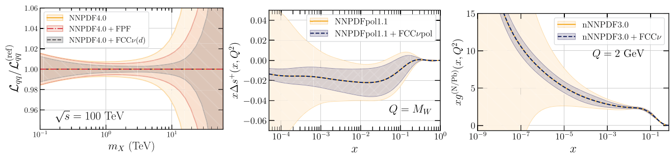
Fig. 47 Projected constraints from the FPF@FCC experiments on the unpolarised (left) and polarised (middle) PDFs, and on the nuclear PDFs of lead nuclei (right)
