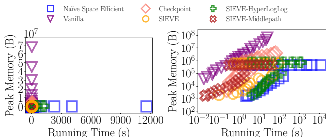
Figure 1: Peak memory vs. runtime with growing path length or state-space size; shown in both linear and log scale.
