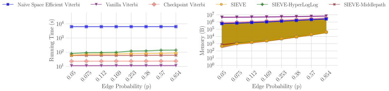
Figure 5: Syntentic data: runtime and memory usage vs. probability of edge existence (log-log scale), K = T = 500 .
