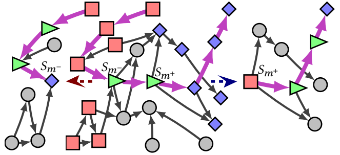
Figure 3: An acyclic HMM, Viterbi path (thick arrows), median pairs (triangles), predecessors (squares) and successors (diamonds) across two levels of the recursion in SIEVE.
