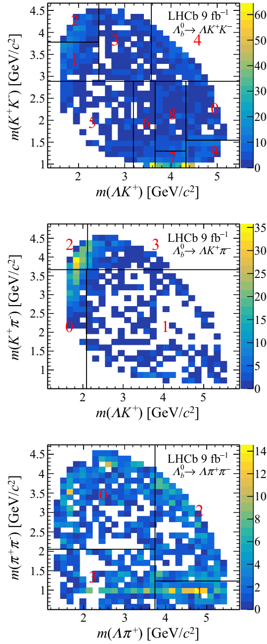
FIG. 4. Two-dimensional mass distributions for (top) \Lambda_b^0 \rightarrow \Lambda K^+ K^- , (middle) \Lambda_b^0 \rightarrow \Lambda K^+ \pi^- , and (bottom) \Lambda_b^0 \rightarrow \Lambda \pi^+ \pi^- decays in data. The boundaries for the adaptive binning scheme are drawn as solid lines.
