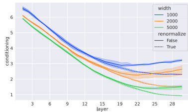
(1b) Mean log-conditioning of G^{m;\theta} for 500 examples at varying widths (colored differently); shaded regions denote 95% confidence intervals.
