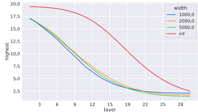
(1d) Normalized highest eigenvalue for ReLU networks of different widths with renormalization. To make the graph more clear only the mean is reported.
