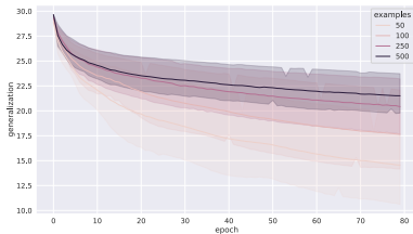
(4b) Generalization bounds for ReLU networks trained under MSE.
