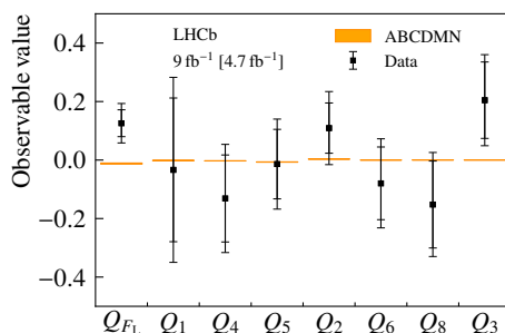
Figure 13. LFU observables Q_i calculated using the P -basis angular observables of the muon and electron modes in the large q^2 region. The overlapping error bars show statistical and total uncertainties. The SM predictions (orange boxes) are based on ref. [14].
