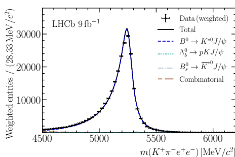
Figure 23. Distribution of the B^0 invariant mass of the control-mode candidates and the result of the fits.
