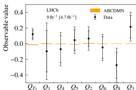
Figure 4. LFU observables Q_i calculated using the P -basis angular observables of the muon and electron modes. The overlapping error bars show statistical and total uncertainties. The SM predictions (orange boxes) are based on ref. [14].
