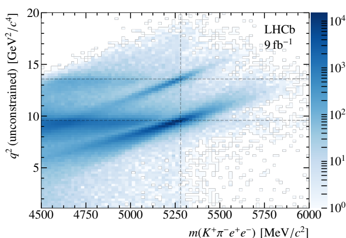
Figure 17. Distribution of the unconstrained q^2 and B^0 invariant mass of signal candidates in data. Signal decays lie in a vertical band close to the known B^0 mass (vertical dashed line) [41]. The decays B^0 \rightarrow K^{*0} J/\psi (\rightarrow e^+ e^-) and B^0 \rightarrow K^{*0} \psi(2S) (\rightarrow e^+ e^-) have an invariant mass close to that of the B^0 meson, and q^2 values close to the square of the known J/\psi and \psi(2S) masses, respectively (horizontal dashed lines). They are visible as diagonal bands. The two horizontal bands contain combinatorial background comprised of genuine J/\psi or \psi(2S) mesons combined with random kaon and pion tracks.
