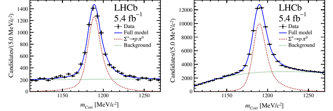
FIG. 6. Distribution of the corrected invariant mass of (left) p\pi^0 TOS candidates with the result of an extended maximum-likelihood fit also shown and (right) corresponding figure for the TIS candidates.
