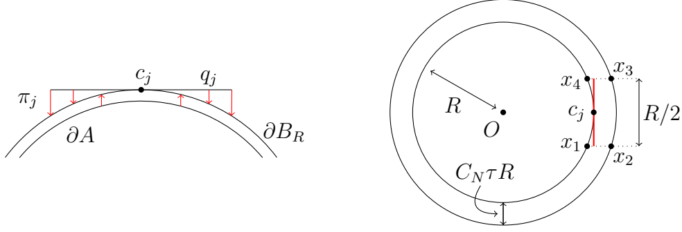
Figure 2.3: The image on the left represents the map \pi_j with the red arrows, the cube q_j that is the horizontal segment. On the right, the cube q_j is represented by the red vertical segment, while the points x_1, x_2, x_3, x_4 denote the corners (since the figure is in 2D) of the outer part of what we call “curved slab” A \cap D_j .
