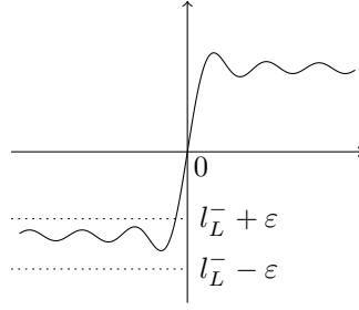
Figure 1.4: Picture of f_\delta when f is odd, showing that the contribution on one side can be very tiny compared to the contribution around 0.
