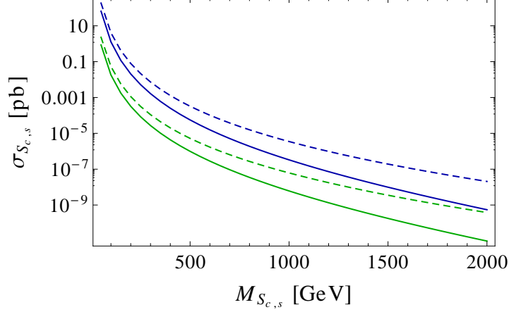
Figure 3: The production cross sections of the lightest flavons S_c (in green) and S_s (in blue) at the LHC with \sqrt{s} = 8 TeV (solid) or 14 TeV (dashed) for different values of their mass.
