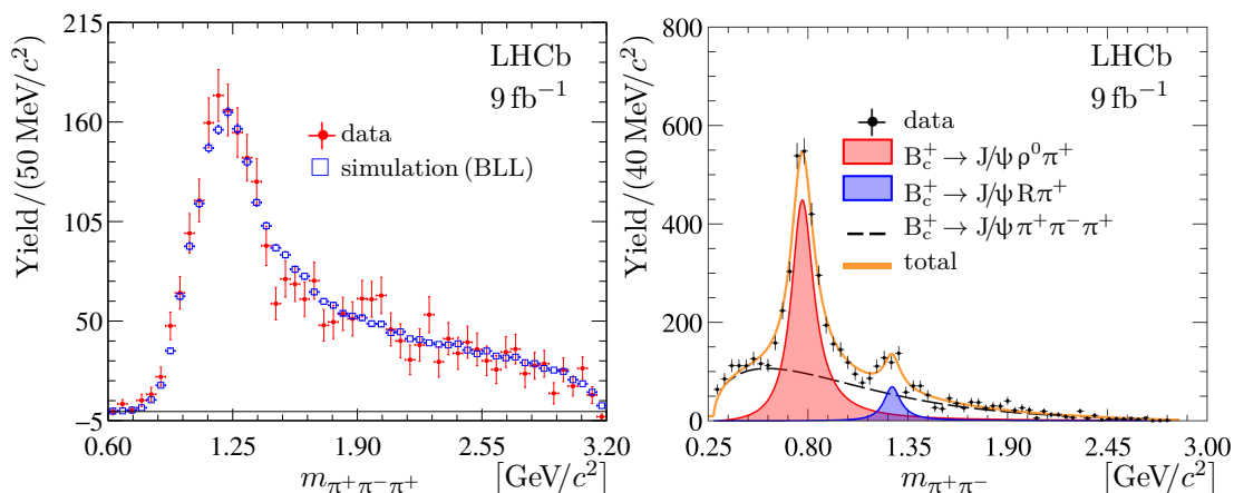
Figure 3. Background-subtracted (left) \pi^+\pi^-\pi^+ and (right) \pi^+\pi^- mass distributions for selected B_c^+ \rightarrow J/\psi \pi^+ \pi^- \pi^+ candidates. In the left plot the expectation from simulation for the B_c^+ \rightarrow J/\psi a_1(1260)^+ decays with BLL model [26, 28, 43] is overlaid.
