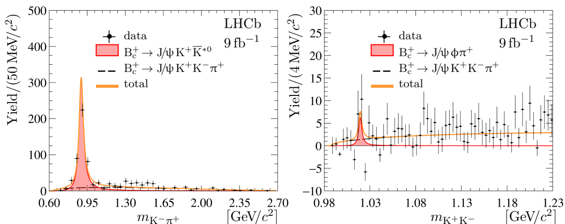
Figure 4. Background-subtracted (left) K^-\pi^+ and (right) K^+K^- mass distributions for selected B_c^+ \rightarrow J/\psi K^+ K^- \pi^+ candidates. The K^+K^- mass spectrum is fitted in the full accessible K^+K^- mass region, m_{K^+K^-} < 2.923 \text{ GeV}/c^2 . For better visibility, only a low-mass part of the spectrum is shown.
