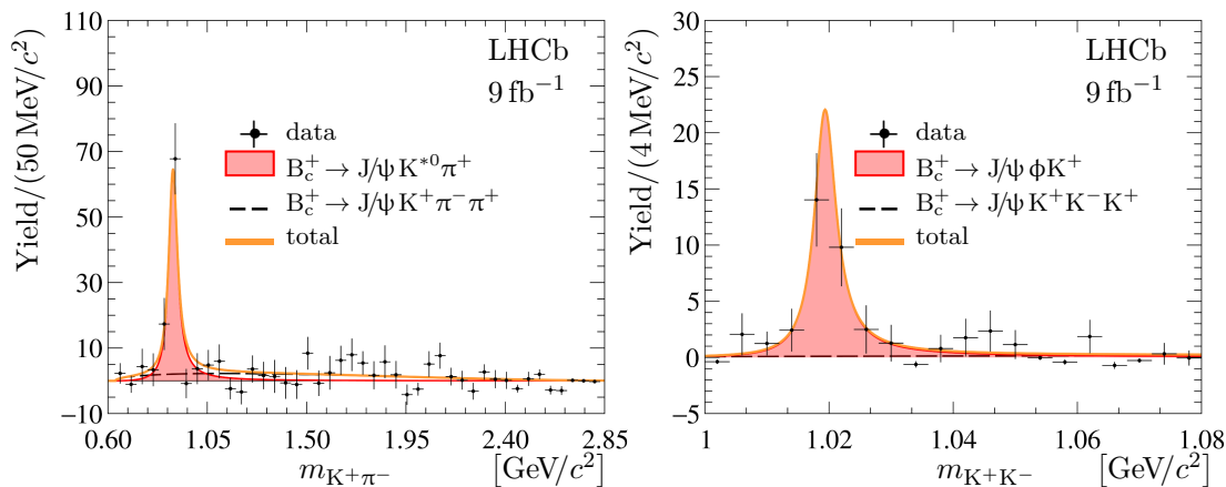
Figure 5. Background-subtracted mass distributions of (left) K^+\pi^- pairs for the selected B_c^+ \rightarrow J/\psi K^+\pi^-\pi^+ candidates and (right) K^+K^- combinations for the selected B_c^+ \rightarrow J/\psi K^+K^-K^+ candidates. The K^+K^- mass spectrum is fitted in the full accessible K^+K^- mass region, m_{K^+K^-} < 2.2 \text{ GeV}/c^2 . For better visibility, only a low-mass part of the spectrum is shown.
