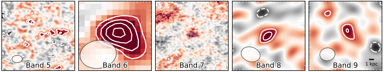
Figure 1. The dust continuum of MACS0416-Y1 in all (tentatively) detected Bands, namely 5, 6, 7, 8, and 9 – covering rest-frame wavelengths 160 to 45 \mu\text{m} . For Band 9, the 0.5 arcsec uv -tapered dust continuum is shown. The poststamps are 3 arcsec \times 3 arcsec, with the background image showing the continuum overlaid, together with white contours indicating the 2, 3, 4, 5 \sigma emission. The beam is shown in the bottom-left corner, and the scalebar is shown in the bottom-right corner in the right-hand side poststamp.
