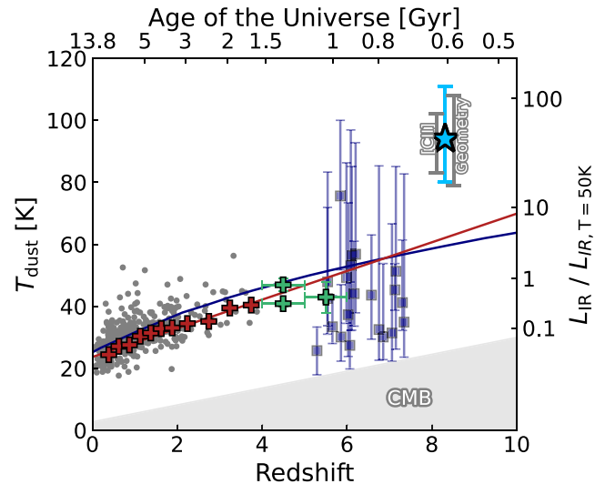
Figure 4. Dust temperature of galaxies and samples as a function of redshift. The dust temperature estimate for Y1 is shown in light blue , and is compared to previous estimates based on [C II] (L. Sommovigo et al. 2021) and on a clumpy dust distribution geometric estimate (Y. Fudamoto et al. 2023) in grey. Dust temperatures obtained for lower-redshift sources at z < 4 are shown in grey points (C. Schreiber et al. 2018), and for higher-redshift galaxies in blue squares (A. L. Faisst et al. 2020; Y. Harikane et al. 2020; Y. Sugahara et al. 2022; J. Witstok et al. 2023a; H. S. B. Algera et al. 2024a, b). Dust temperature evolution based on stacked SEDs is shown in red and green pluses , which are shown to increase linearly with redshift up to z = 6 (M. Béthermin et al. 2015; C. Schreiber et al. 2018; M. Béthermin et al. 2020). The best-fit from C. Schreiber et al. (2018) is shown in a red line , while the average physically motivated dust temperature relation from L. Sommovigo et al. (2022a) is shown in a blue line . Prior to the Band 9 data, only lower limits were available on Y1. The other axis indicates the change in infrared luminosity compared to 50 K, indicating the strong dependence of infrared luminosity on dust temperature, and the greyed-out region indicates the CMB temperature at a given redshift.
