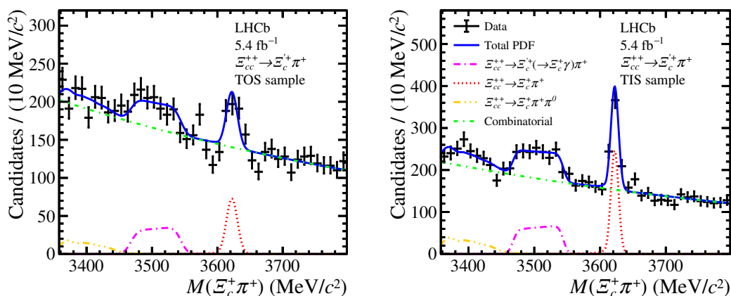
Figure 2. Invariant-mass distribution of the \Xi_{cc}^{++} candidates from the (left) TOS and (right) TIS samples, with the results of the fit overlaid. The \Xi_{cc}^{++} \rightarrow \Xi_c'^+ \pi^+ component is shown as a purple dashed line, the \Xi_{cc}^{++} \rightarrow \Xi_c^+ \pi^+ component as a red dotted line, the \Xi_{cc}^{++} \rightarrow \Xi_c^+ \pi^+ \pi^0 component as a yellow dashed line and the combinatorial component as a green dashed line.
