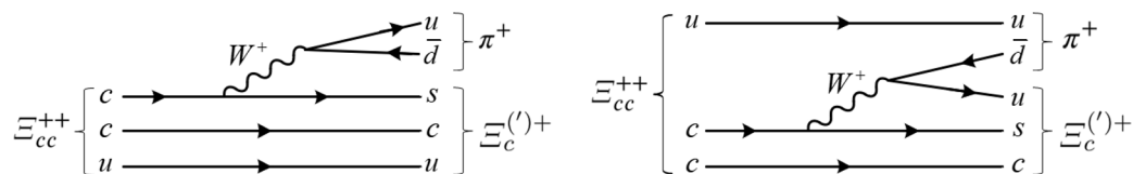
Figure 1. (Left) external and (right) internal W -emission diagrams of the \Xi_{cc}^{++} \rightarrow \Xi_c^{(')+} \pi^+ decay.
