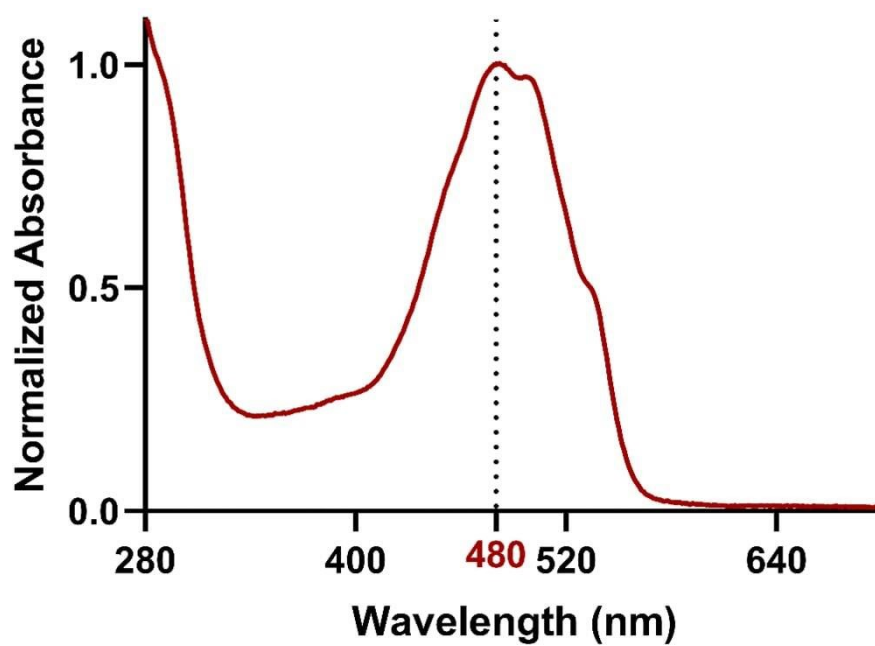
Figure S2: Absorption spectrum of PGA-DOX NGs in H 2 O showing DOX absorbance around 480 nm.
