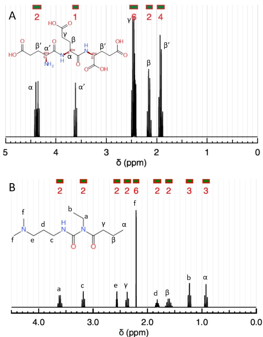
Figure S1: ^1\text{H-NMR} simulated spectra for polyglutamic acid (A) and for the EDC-derived N-Acylisourea (B). Spectra have been predicted using the Nmrdb.org web tool 25,26 with a frequency of 300 MHz. In the insets, the structure of the effectively simulated molecules, with corresponding letters between the structure and the peaks indicating the position of the hydrogen atom responsible for each NMR peak. For (A), only a tripeptide has been simulated, so we expect to see in the PGA spectra mostly the peaks arising from the “central” glutamic acid ( \alpha , \beta , \gamma ); the peak arising from hydrogens close to the C- or N-terminal with significantly different shifts are also shown ( \alpha' , \beta' ). In the structure in (B) the \alpha position corresponds to the \alpha -carbon on the “protein” backbone, so we should not expect to see in the experimental spectra the peaks \alpha and most probably \beta shown here, but rather the ones in panel (A).
