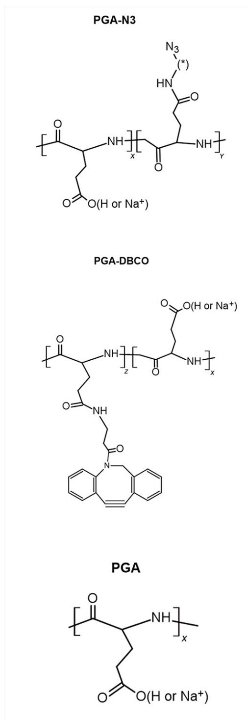
Chart S1: structure of the polymers used for the syntheses
