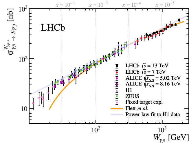
Figure 10: Results for the J/\psi photoproduction cross-section as a function of the photon-proton energy W_{\gamma p} from different experiments listed in Table 3. The LHCb results at \sqrt{s} = 13 TeV are estimated with the NLO [45] calculation. Also shown are the NLO theoretical descriptions given by Flett et al. [45], as well as a power-law description of the H1 data. The top axis shows the values of x reached for a given photon-proton energy.
