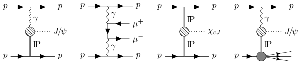
Figure 1: Feynman diagrams for signal and background processes. From left to right: signal CEP J/\psi photoproduction, where \mathbb{P} stands for a colourless superposition of gluons, sometimes referred to as a pomeron; continuum dimuon production; exclusive \chi_c ( J = 0, 1, 2 ) production via double pomeron exchange; inelastic pp collision where a proton dissociates.
