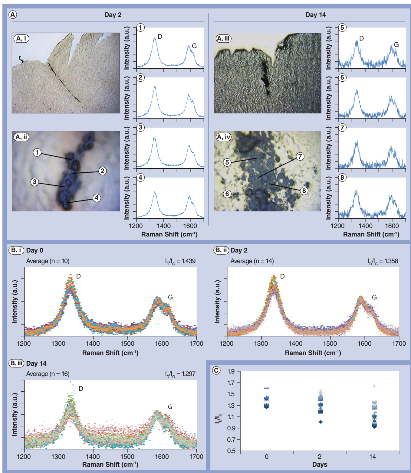
Figure 4. Raman spectroscopy of brain tissue sections 2 and 14 days after stereotactic administration of chemically functionalized-multiwalled carbon nanotubes. (A) Raman spectra of 20- \mu m thick brain sections, 2 days (left) and 14 days (right) postinjection. Spectra presented are representative data, corresponding to locations 1–8 (Aii & Aiv) indicated in the optical microscopy images. (B) Collated Raman spectra as acquired from the starting material before injection (0 days) (B, i) and from brain sections at 2 days (B, ii) and 14 days postinjection (B, iii). The intensity ratio between D and G bands ( I_D/I_G ) indicated was calculated from the average intensities of D and G bands at each time point (n = 10, n = 14 and n = 16 spectra used for each time point, respectively). Average intensity of G band was normalized to 1. (C) I_D/I_G band ratio calculated from Raman spectra in each region of interest in the section. An overall reduction in I_D/I_G ratio was observed with time suggesting dramatic changes in the carbon structure of the nanotubes inside the brain. I_D/I_G : Intensity ratio between D and G bands.
