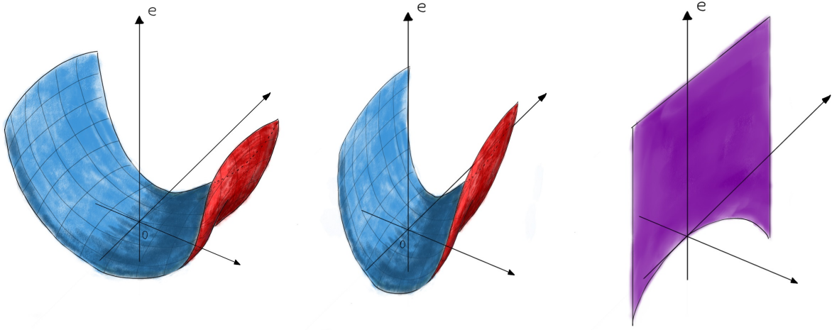
Figure 6.1: The image shows why a sequence of quadrics having only one eigenvalue diverging cannot converge to a full plane.
