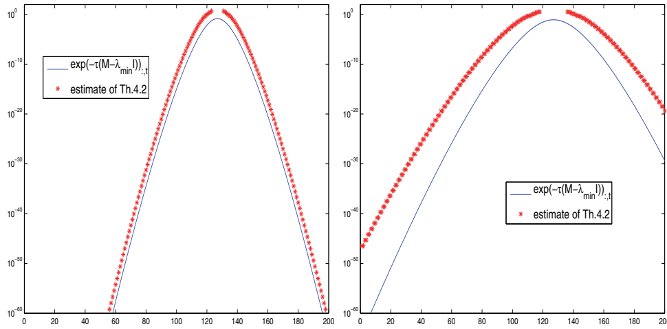
FIG. 1. Example 4.3. Bounds for |\exp(-\tau(M - \lambda_{\min}I))_{:,t}| , t = 127 , using Theorem 4.2. M of size n = 200 and \tau = 4 . Left: M = \text{tridiag}(-1, 4, -1) . Right: M = \text{pentadiag}(-0.5, -1, 4, -1, -0.5) . Logarithmic scale.
