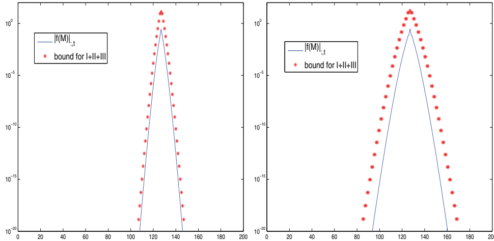
FIG. 3. Estimates for |M^{-1}(I - \exp(-M))_{:,t}| , t = 127 , using I+II and the upper bound for III . Size n = 200 , log-scale. Left: M = \text{tridiag}(-1, 4, -1) . Right: M = \text{pentadiag}(-0.5, -1, 4, -1, -0.5) .
