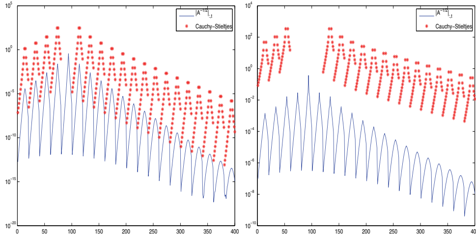
FIG. 7. Example 6.5. True decay and estimates for |A_{:,t}^{-\frac{1}{2}}| , t = 94 , A = M \otimes I + I \otimes M of size n = 400 . Left: M = \text{tridiag}(-1, 4, -1) . Right: M = \text{pentadiag}(-0.5, -1, 4, -1, -0.5) .
