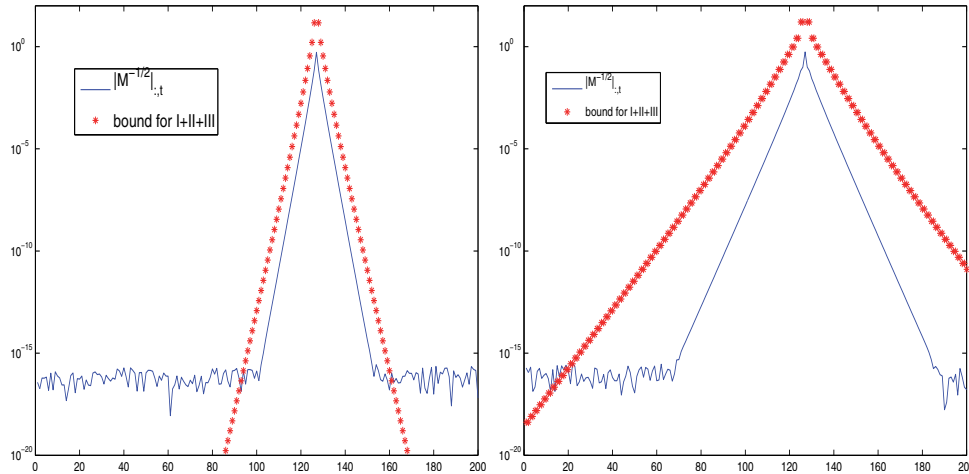
FIG. 2. Estimates for |M_{:,t}^{-1/2}| , t = 127 , using I+II and the upper bound for III . Size n = 200 , log-scale. Left: M = \text{tridiag}(-1, 4, -1) . Right: M = \text{pentadiag}(-0.5, -1, 4, -1, -0.5) .
