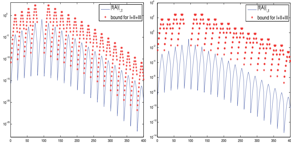
FIG. 6. Example 6.4. True decay and estimates for |f(A)_{:,t}| , t = 94 , A = M \otimes I + I \otimes M of size n = 400 . Left: M = \text{tridiag}(-1, 4, -1) . Right: M = \text{pentadiag}(-0.5, -1, 4, -1, -0.5) .
