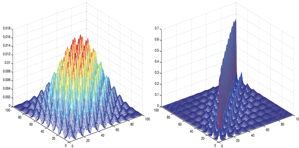
FIG. 5. Three-dimensional decay plots for [f(\mathcal{A})]_{ij} where \mathcal{A} is the 5-point finite difference discretization of the negative Laplacian on the unit square on a 10 \times 10 uniform grid with zero Dirichlet boundary conditions. Left: f(\mathcal{A}) = \exp(-5\mathcal{A}) . Right: f(\mathcal{A}) = \mathcal{A}^{-1/2} .
