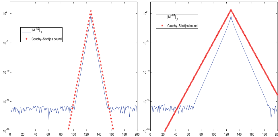
FIG. 4. Estimates for |M_{:,t}^{-1/2}| , t = 127 , using (4.3), size n = 200 , log-scale. Left: M = \text{tridiag}(-1, 4, -1) . Right: M = \text{pentadiag}(-0.5, -1, 4, -1, -0.5) .
