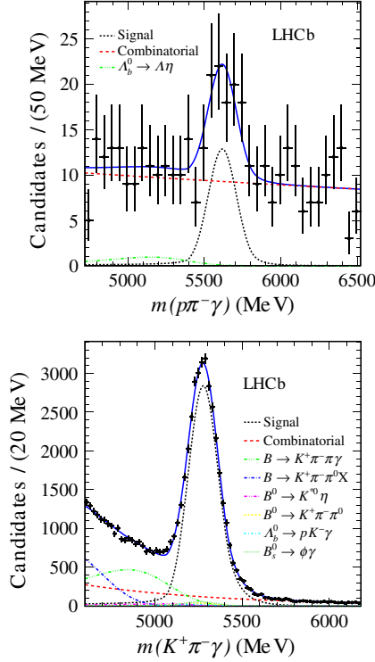
FIG. 1. Simultaneous fit to the (top) \Lambda_b^0 \rightarrow \Lambda\gamma and (bottom) B^0 \rightarrow K^{*0}\gamma invariant-mass distributions of selected candidates. The data are represented by black dots and the result of the fit by a solid blue curve while individual contributions are represented in different line styles (see legend).
