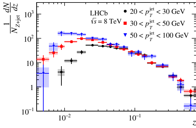
FIG. 1. Distributions of the longitudinal momentum fraction of the hadron with respect to the jet in three bins of jet p_T . The bars (boxes) show the statistical (systematic) uncertainties.
