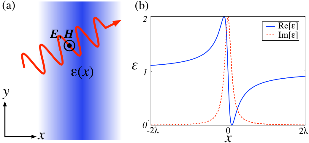
FIG. 1: We consider a wave propagating in the x - y plane in an inhomogeneous medium with permittivity \epsilon(x) (indicated by the blue shading in panel (a)). The TE polarization has an electric field pointing only along z and the TM polarization has a magnetic field pointing only along z . When the real (blue) and imaginary (red) parts of the permittivity are related to one another by the Kramers–Kronig relations as in panel (b) then the reflection vanishes for all angles of incidence. Panel (b) shows the permittivity profile \epsilon(x) given by equation (11) for the parameters A = 2.0 and \xi = 0.1\lambda with \lambda = 2\pi/k_0 .
