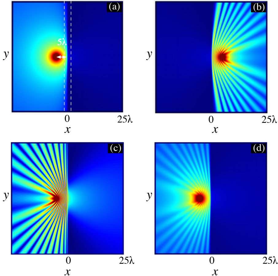
FIG. 2: To test the reflection for all angles of incidence we simulated a line source (pointing out of the page) placed within the inhomogeneous permittivity profile shown in figure 1b. The simulations were performed using Comsol Multiphysics, and panels (a) and (b) show the absolute value of the electric field of a line source placed at respective positions x = -5\lambda and x = +5\lambda in the permittivity profile. The region between the vertical dashed lines in (a) indicates the region plotted in figure 1b. Panels (c) and (d) are for identical parameters, but we have taken only the real and imaginary parts of the permittivity respectively. The absence of any oscillations in panel (a) shows that the reflection is completely suppressed for incidence from the left, for all incident angles.
