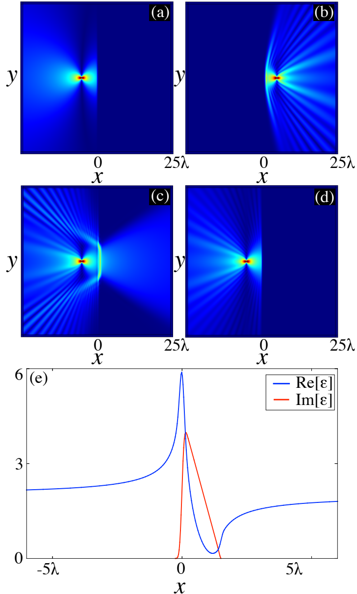
FIG. 3: In cases where the permittivity has neither poles nor zeros in the upper half position plane, then the reflection also vanishes for the TM polarization. Panel (a) shows the field of a dipole source aligned along the y axis (so that the field is TM polarized), and placed at x = -5\lambda in front of the permittivity profile shown in panel (e). Panel (b) shows a dipole radiating in the same profile but at x = +5\lambda . Panels (c-d) show the reflection from just the real and imaginary parts of the profile respectively. Panel (e) shows the permittivity profile, the imaginary part of which is given by (15) with \epsilon_b = 2 , L = 1.5\lambda , \xi = 0.1\lambda , and h = 4.5 . The real part of the profile was numerically calculated using (10).
